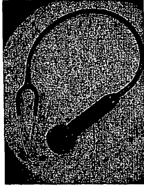
Figure 37: Bottom view of stethoscope prototype
