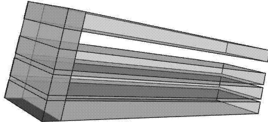
Fig. 24A. End of cell with Plurality of sacrificial cathodes And single outside Of cell connector
