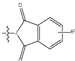
Formula C
