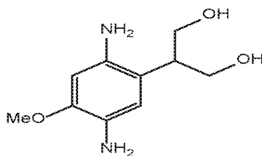
Methoxy, hydroxy PPD
