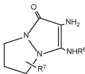
Formula IX
