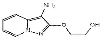
pyrrolopyridine
