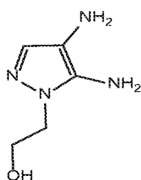
amino pyrazole
