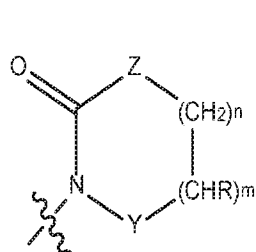
Formula A
