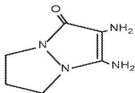
Dihydro PPZO
