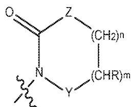
Formula A
