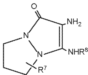
Formula IX
