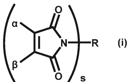
[Chem. 34]
