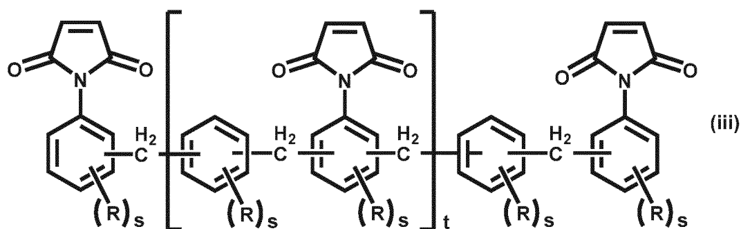
[Chem. 36]
