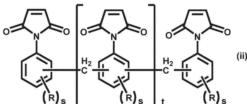
[Chem. 35]
