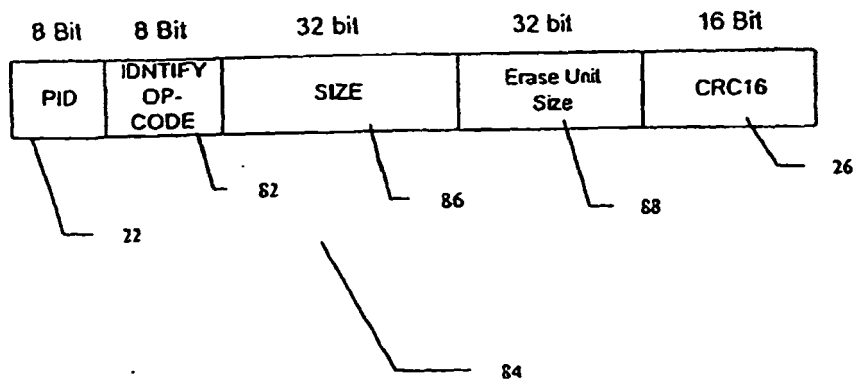
Fig 8 – Flash Identification Replay Packet
