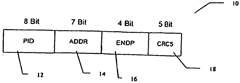
Figure 1 – Background Art USB Token Packet Structure
