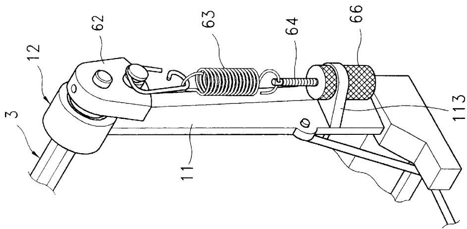
PRIOR ART FIG. 3A
