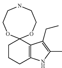
Impurity 3
