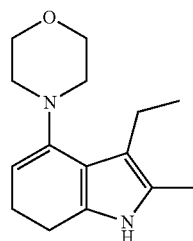
Impurity 4
