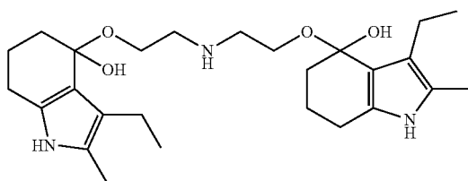
Impurity 2
