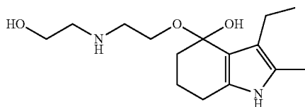
Impurity 1
