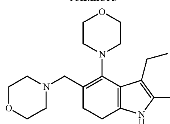
Impurity 5
