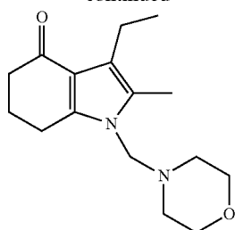
N-Morpholinomethyl SUMO-2
