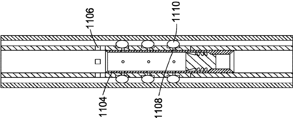
ACTIVE DONUT & SHEAR SLEEVE F/ CEMENTING
