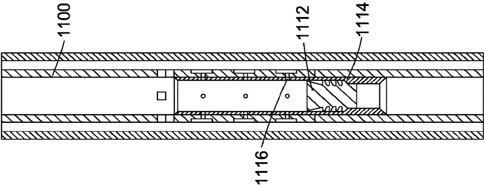
DROP CEMENTING DART & ALIGN PORTS
