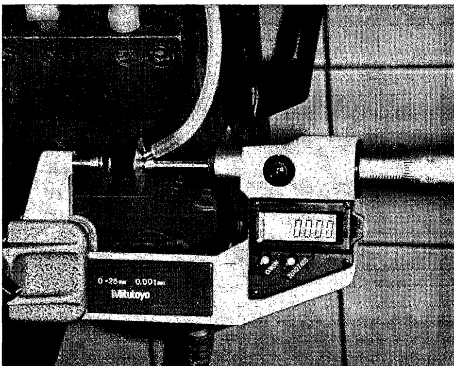
Photograph 4: Micrometer set-up in sample preparation for cavitation strength measurement
