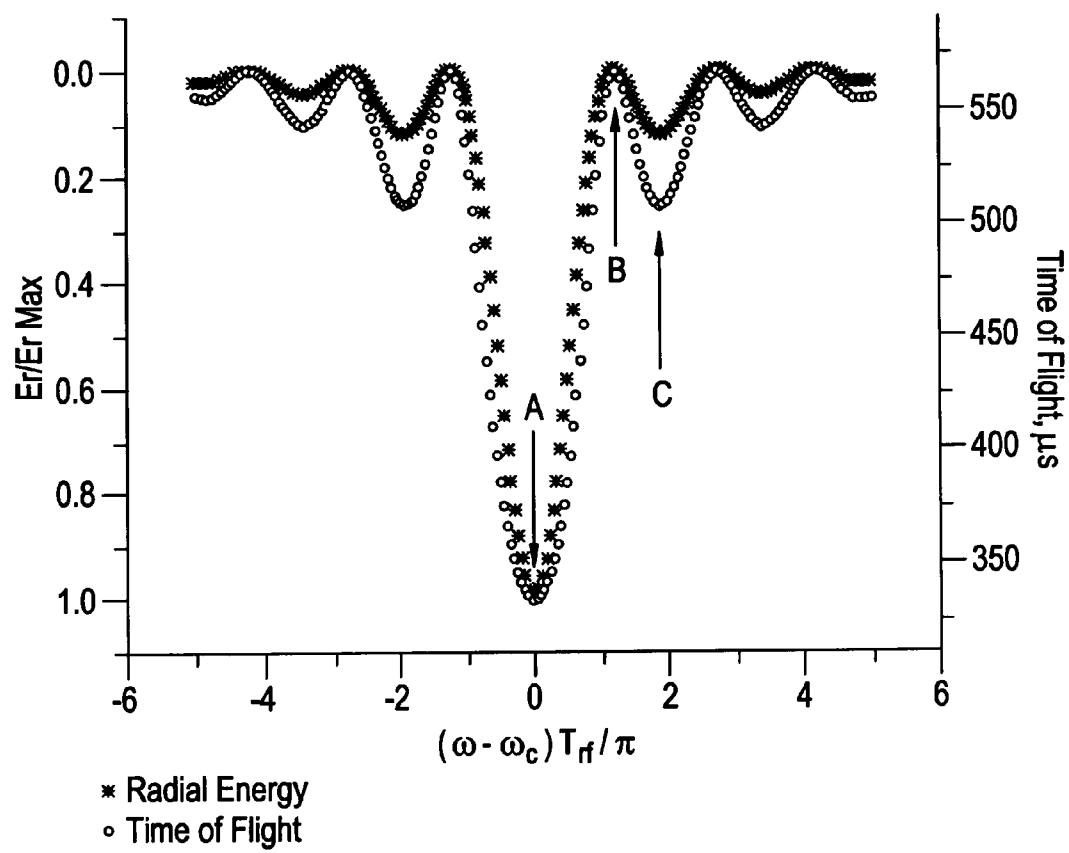
FIG. 3A CONVENTIONAL ART
