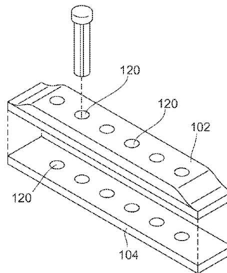
Fig. 20 PRIOR ART
