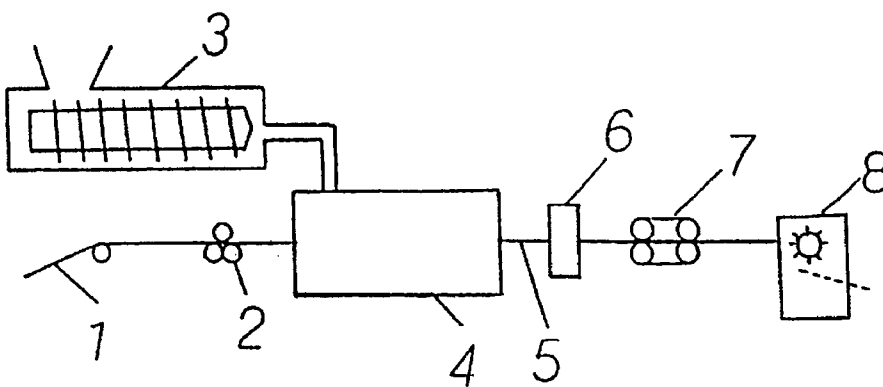
Fig. 6 (Prior Art)
