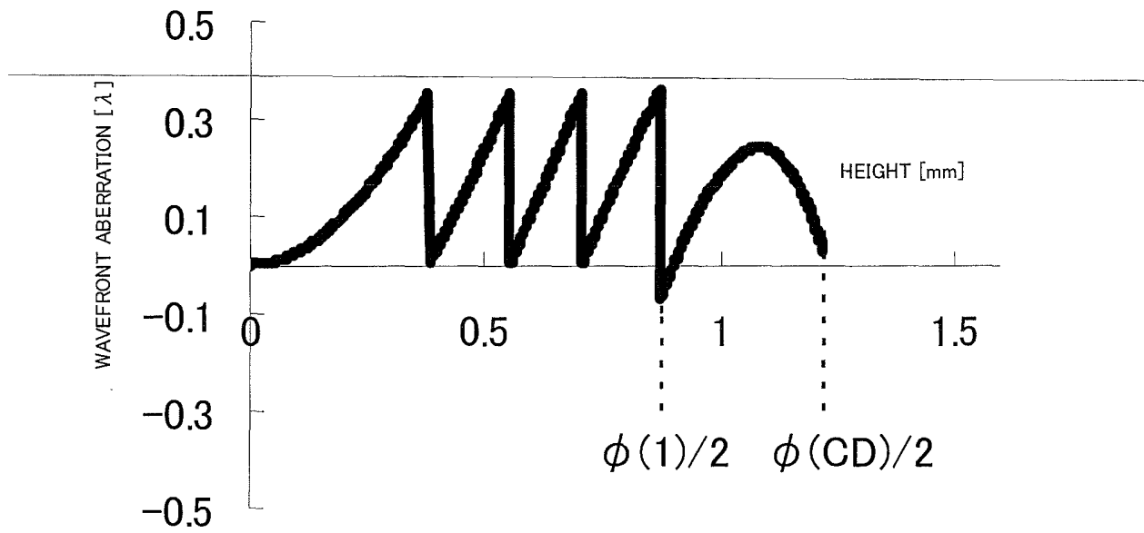
CD WAVEFRONT ABERRATION
