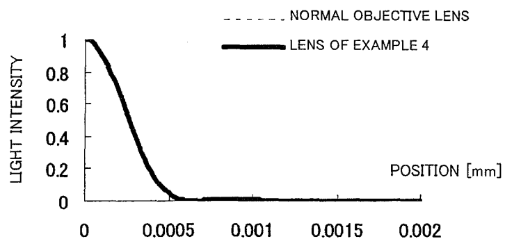
FIG.122 DVD SPOT SHAPE (GENERAL VIEW)
