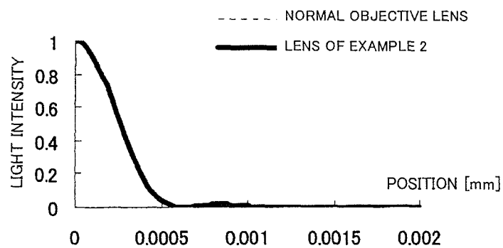
FIG.69 DVD SPOT SHAPE (GENERAL VIEW)
