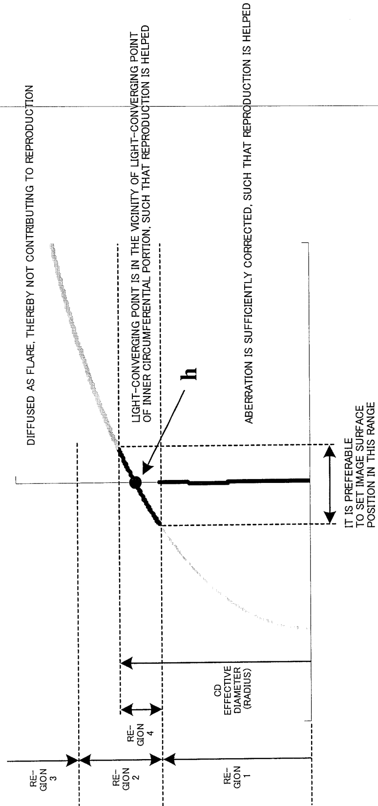
LONGITUDINAL SPHERICAL ABERRATION DIAGRAM FOR CD
