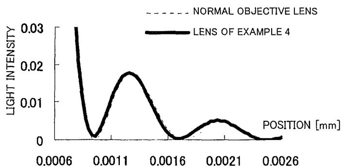
FIG.126 CD SPOT SHAPE (SIDE ROBE)
