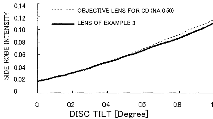
FIG.104 SIDE ROBE INTENSITY AT THE TIME OF DISC TILT OF CD
