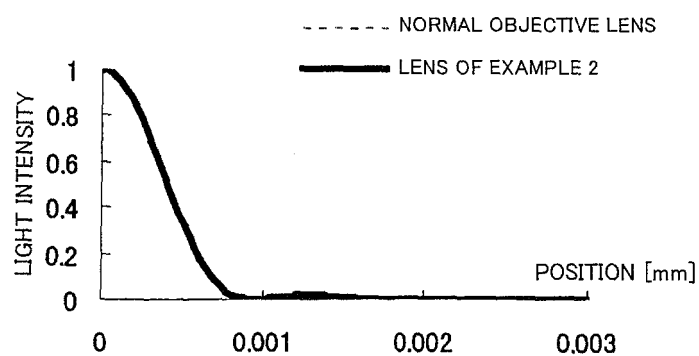
FIG.70 CD SPOT SHAPE (GENERAL VIEW)
