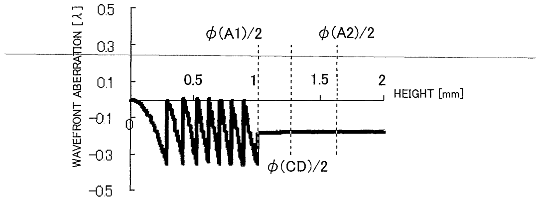
FIG.92 BD WAVEFRONT ABERRATION
