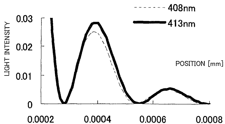
FIG.137 BD SPOT SHAPE (SIDE ROBE)
