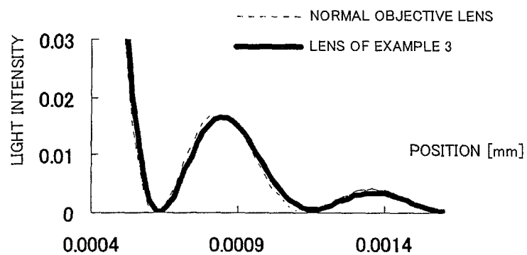
FIG.99 DVD SPOT SHAPE (SIDE ROBE)
