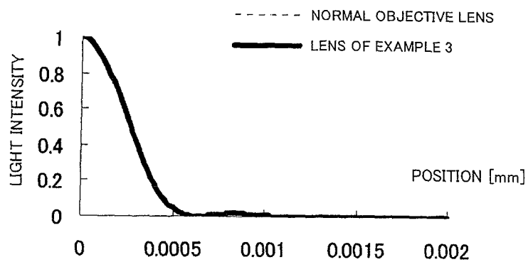
FIG.96 DVD SPOT SHAPE (GENERAL VIEW)
