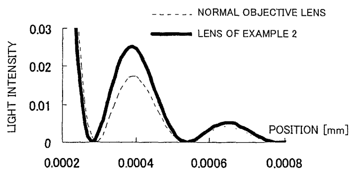
FIG.71 BD SPOT SHAPE (SIDE ROBE)
