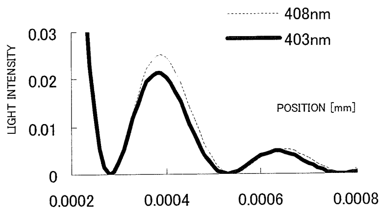
FIG.110 BD SPOT SHAPE (SIDE ROBE)
