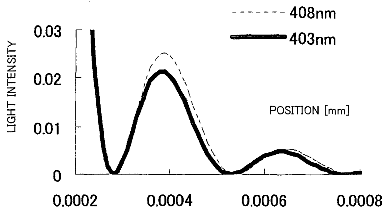
FIG.136 BD SPOT SHAPE (SIDE ROBE)
