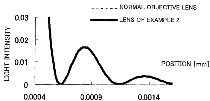
FIG.72 DVD SPOT SHAPE (SIDE ROBE)
