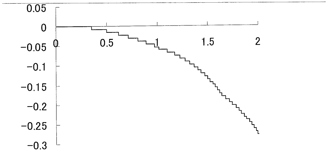
SECTIONAL SHAPE OF DIFFRACTIVE LENS STRUCTURE B
