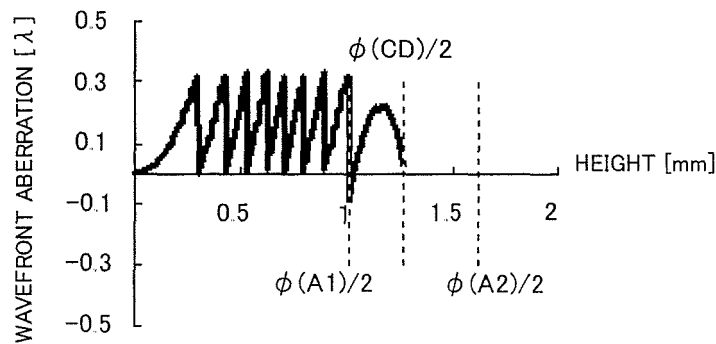
FIG.67 CD WAVEFRONT ABERRATION
