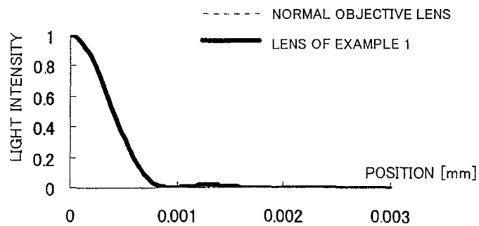
FIG.49 CD SPOT SHAPE (GENERAL VIEW)
