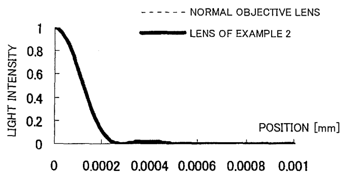
FIG.68 BD SPOT SHAPE (GENERAL VIEW)
