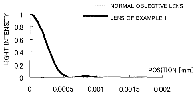
FIG.48 DVD SPOT SHAPE (GENERAL VIEW)
