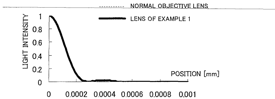
FIG.47 BD SPOT SHAPE (GENERAL VIEW)
