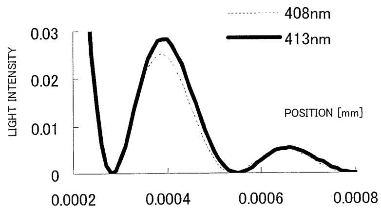
FIG.111 BD SPOT SHAPE (SIDE ROBE)
