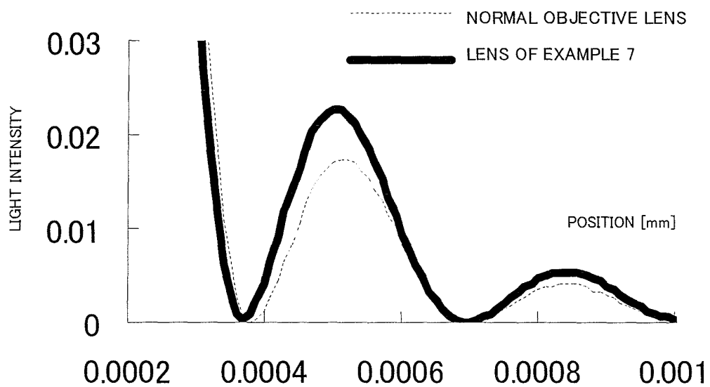
HD-DVD SPOT SHAPE (SIDE ROBE)
