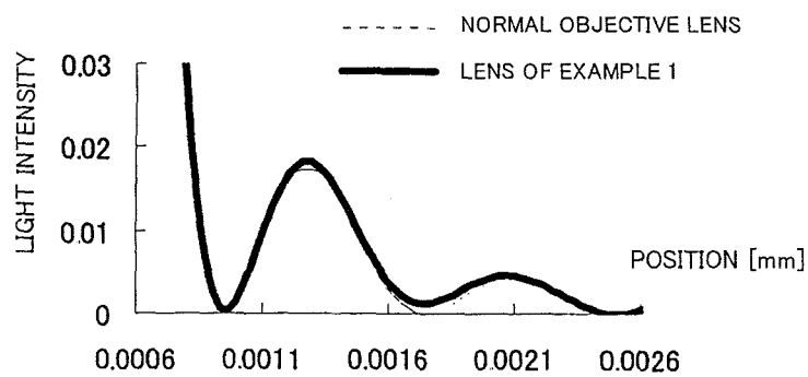
FIG.52 CD SPOT SHAPE (SIDE ROBE)
