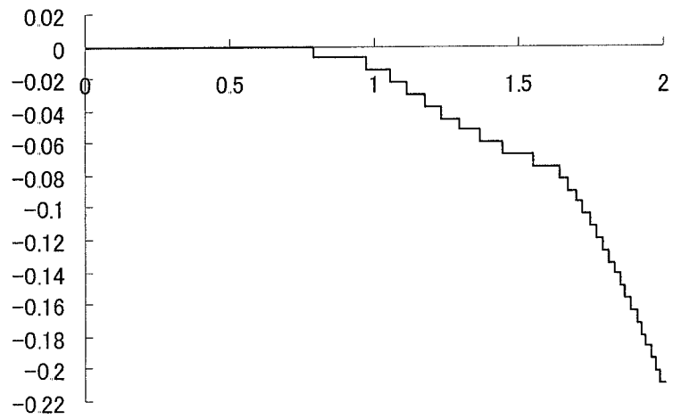
SECTIONAL SHAPE OF DIFFRACTIVE LENS STRUCTURE B
