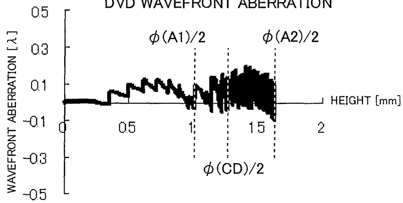
FIG.93 DVD WAVEFRONT ABERRATION
