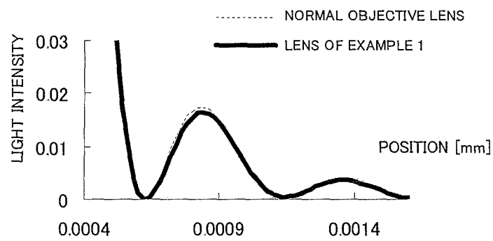
FIG.51 DVD SPOT SHAPE (SIDE ROBE)
