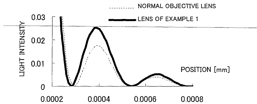
FIG.50 BD SPOT SHAPE (SIDE ROBE)
