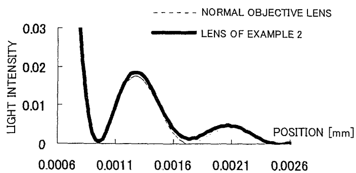
FIG.73 CD SPOT SHAPE (SIDE ROBE)
