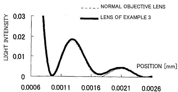
FIG.100 CD SPOT SHAPE (SIDE ROBE)
