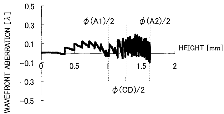
FIG.66 DVD WAVEFRONT ABERRATION
