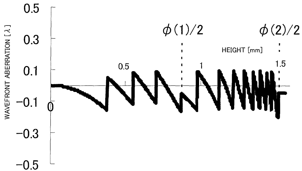
FIG.199 DVD WAVEFRONT ABERRATION
