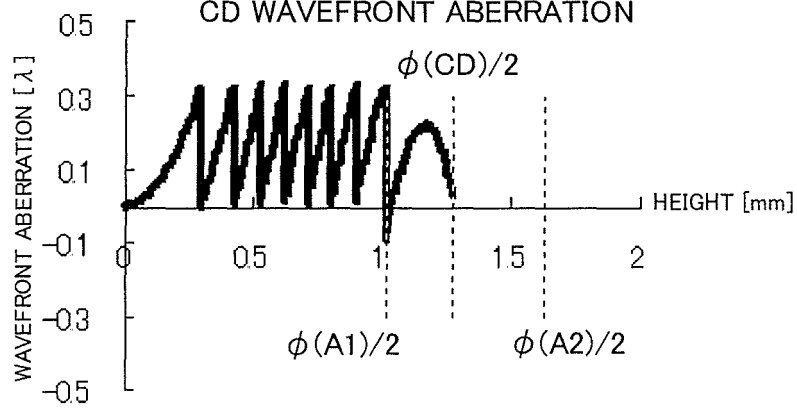
FIG.94 CD WAVEFRONT ABERRATION
