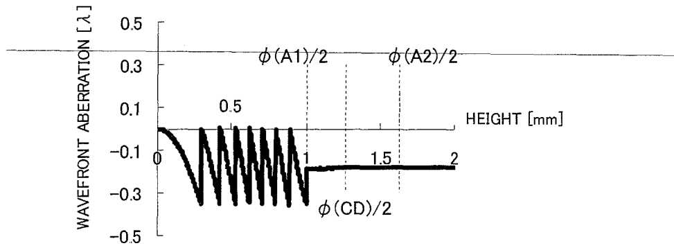
FIG.65 BD WAVEFRONT ABERRATION
