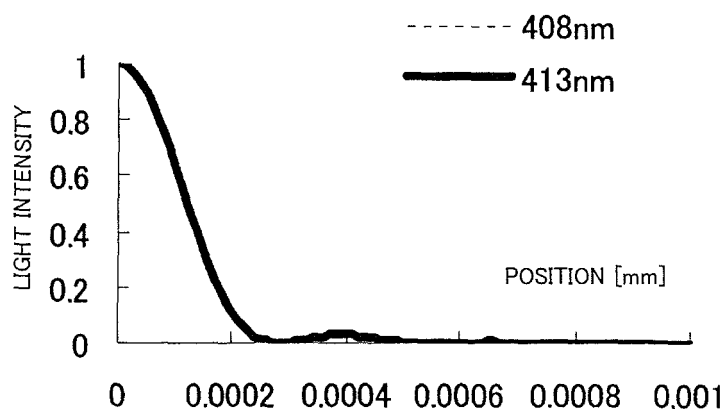
FIG.135 BD SPOT SHAPE (GENERAL VIEW)
