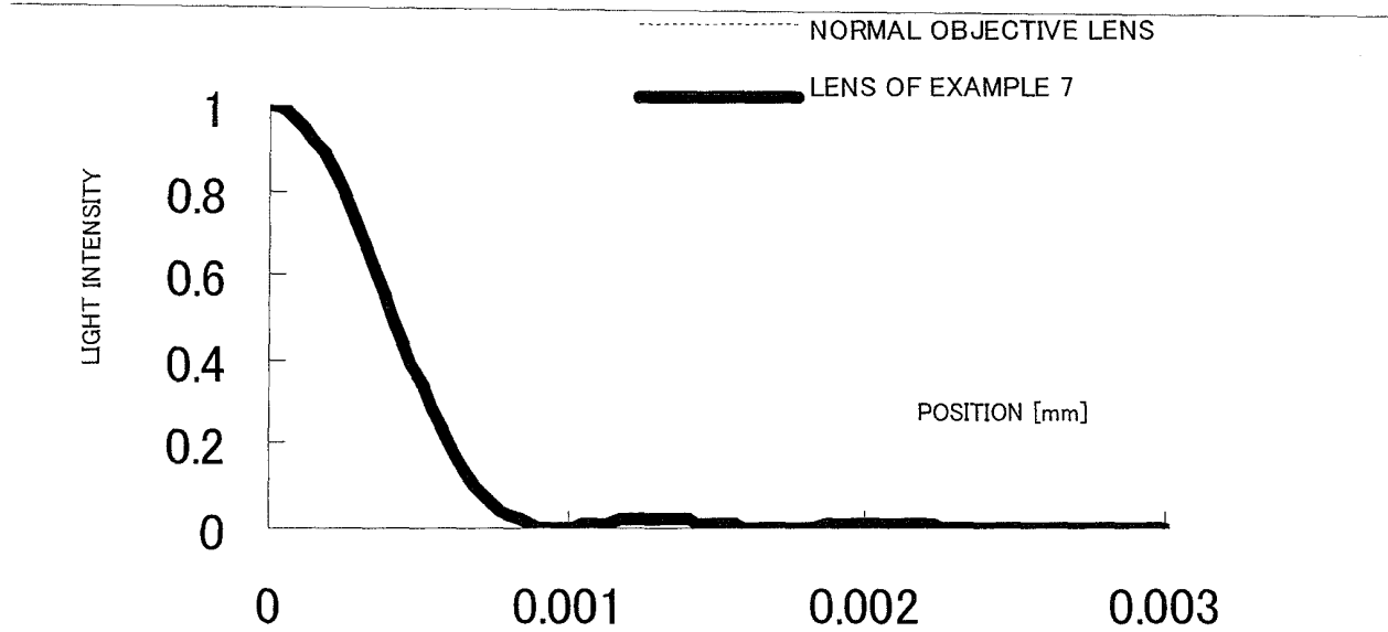
CD SPOT SHAPE (GENERAL VIEW)
