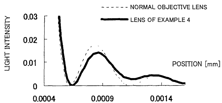
FIG.125 DVD SPOT SHAPE (SIDE ROBE)
