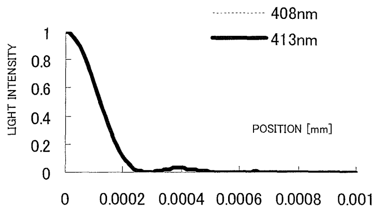
BD SPOT SHAPE (GENERAL VIEW)
