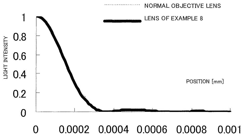
HD-DVD SPOT SHAPE (GENERAL VIEW)
