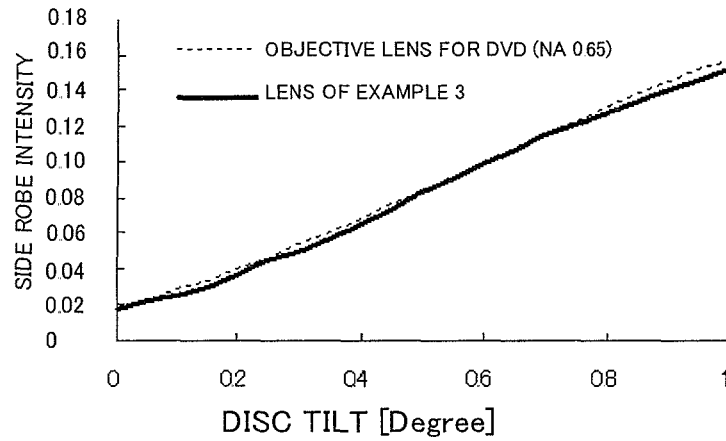
FIG.103 SIDE ROBE INTENSITY AT THE TIME OF DISC TILT OF DVD
