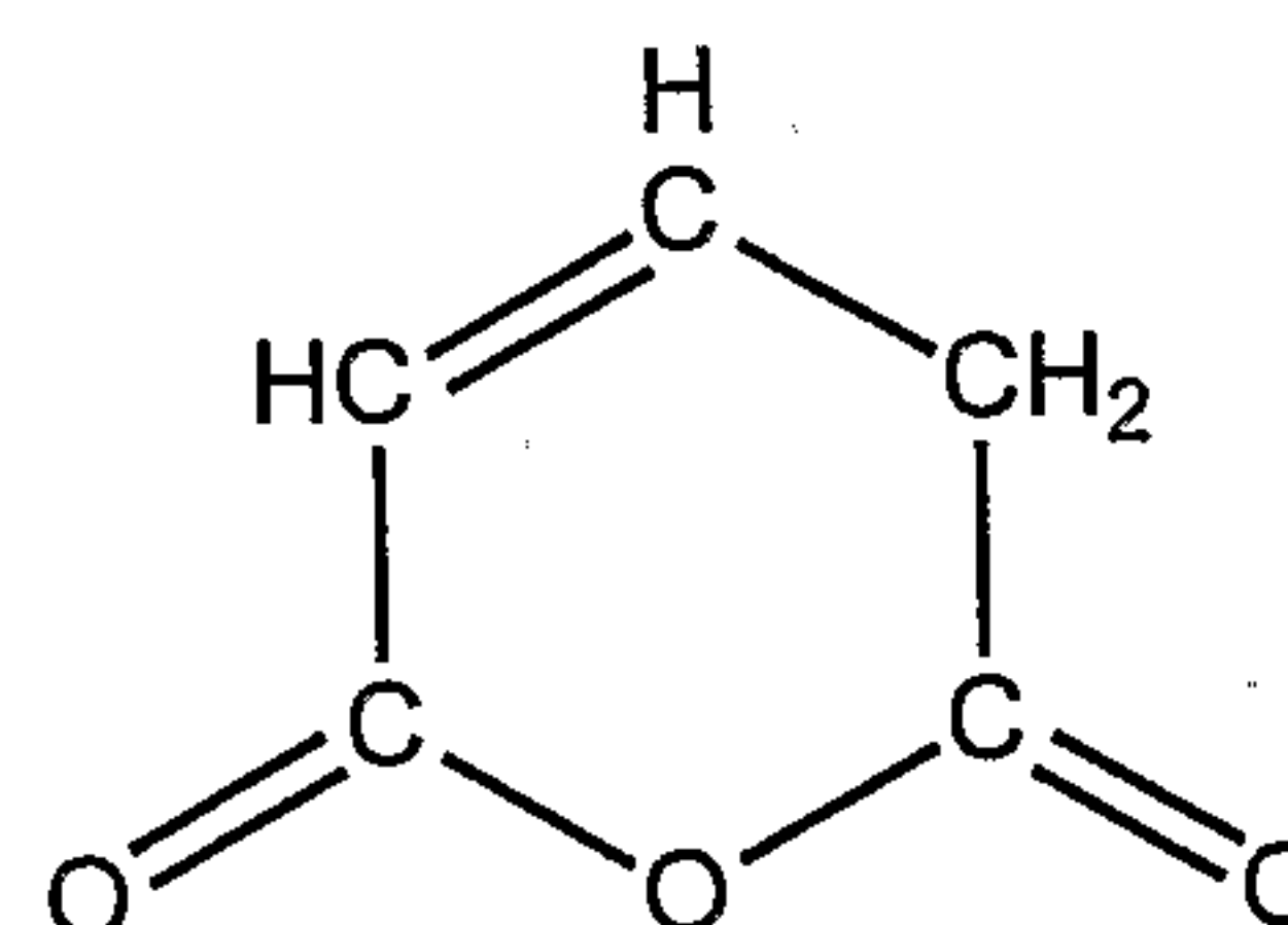
2-Pentendioic Anhydride
