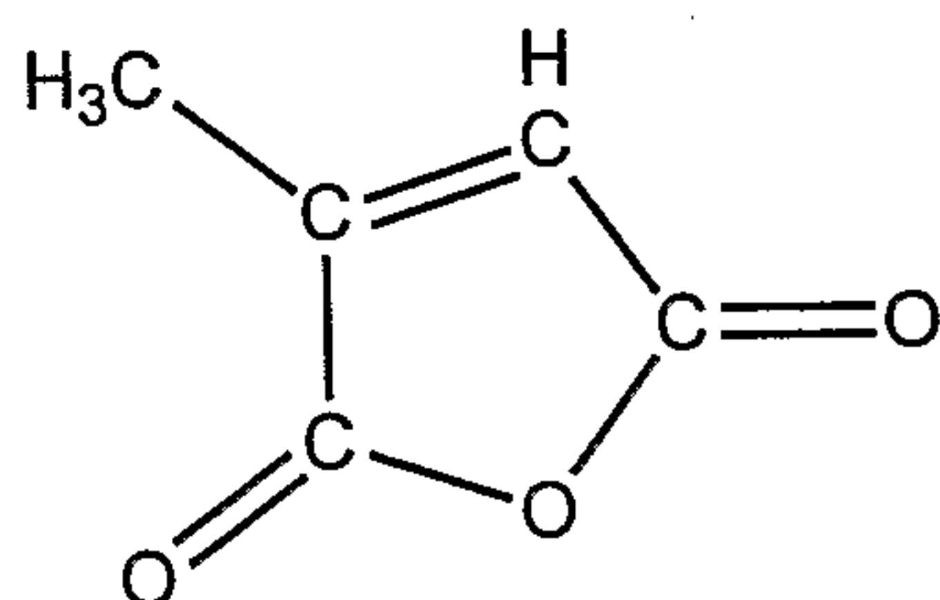
Citraconic Anhydride
