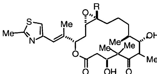
Epothilone A R=H
