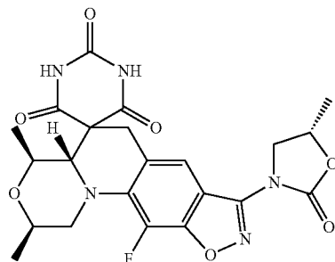
(2R,4S,4aS)-11-Fluoro-2,4-dimethyl-8-[(5S)-5-methyl-2-oxo-1,3-oxazolidin-3-yl]-1,2,4,4a-tetrahydro-2'H,6H-spiro[1,4-oxazino[4,3-a][1,2]oxazolo[4,5-g]quinoline-5,5'-pyrimidine]-2',4',6'(1'H,3'H)-trione
