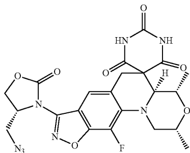
(2R,4S,4aS)-8-((R)-4-(Azidomethyl)-2-oxooxazolidin-3-yl)-11-fluoro-2,4-dimethyl-2,4,4a,6-tetrahydro-1H,1'H-spiro[isoxazolo[4,5-g][1,4]oxazino[4,3-a]quinoline-5,5'-pyrimidine]-2',4',6'(3'H)-trione
