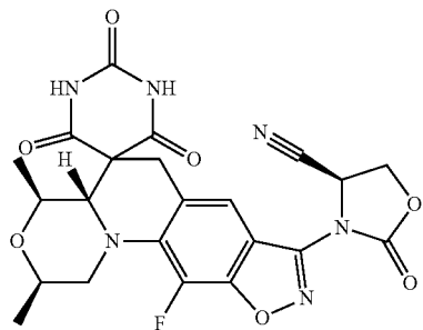
(4S)-3-[(2R,4S,4aS)-11-Fluoro-2,4-dimethyl-2',4',6'-trioxo-1,1',2,3',4,4',4a,6'-octahydro-2'H,6H-spiro[1,4-oxazino[4,3-a][1,2]oxazolo[4,5-g]quinoline-5,5'-pyrimidin]-8-yl]-2-oxo-1,3-oxazolidine-4-carbonitrile
