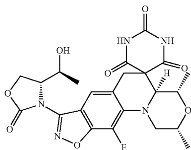
(2R,4S,4aS)-11-Fluoro-8-((R)-4-((S)-1-hydroxyethyl)-2-oxooxazolidin-3-yl)-2,4-dimethyl-2,4,4a,6-tetrahydro-1H,1'H-spiro[isoxazolo[4,5-g][1,4]oxazino[4,3-a]quinoline-5,5'-pyrimidine]-2',4',6'(3'H)trione
