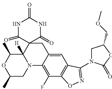
(2R,4S,4aS)-11-Fluoro-8-[(5R)-4-(methoxymethyl)-2-oxo-1,3-oxazolidin-3-yl]-2,4-dimethyl-1,2,4,4a-tetrahydro-2'H,6'H-spiro[1,4-oxazino[4,3-a][1,2]oxazolo[4,5-g]quinoline-5,5'-pyrimidine]-2',4',6'(1'H,3'H)-trione
