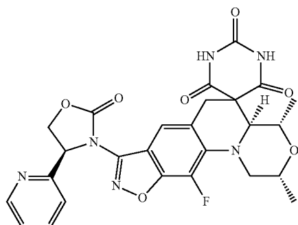
(2R,4S,4aS)-11-fluoro-2,4-dimethyl-8-((S)-2-oxo-4-(pyridin-2-yl)oxazolidin-3-yl)-2,4,4a,6-tetrahydro-1H,1'H-spiro[isoxazolo[4,5-g][1,4]oxazino[4,3-a]quinoline-5,5'-pyrimidine]-2',4',6'(3'H)-trione
