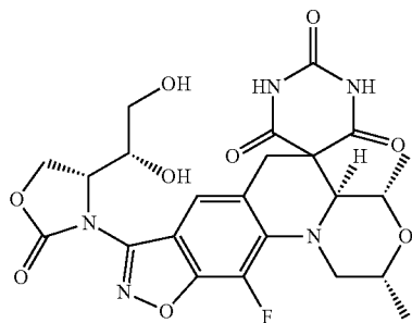
(2R,4S,4aS)-8-((R)-4-((R)-1,2-Dihydroxyethyl)-2-oxooxazolidin-3-yl)-11-fluoro-2,4-dimethyl-2,4,4a,6-tetrahydro-1H,1'H-spiro[isoxazolo[4,5-g][1,4]oxazino[4,3-a]quinoline-5,5'-pyrimidine]-2',4',6'(3'H)-trione
