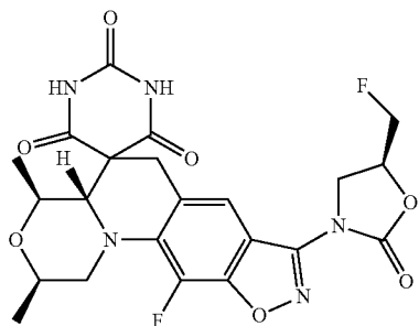
(2R,4S,4aS)-11-Fluoro-8-((S)-5-(fluoromethyl)-2-oxooxazolidin-3-yl)-2,4-dimethyl-2,4,4a,6-tetrahydro-1H,1'H-spiro[isoxazolo[4,5-g][1,4]oxazino[4,3-a]quinoline-5,5'-pyrimidine]-2',4',6'(3'H)-trione
