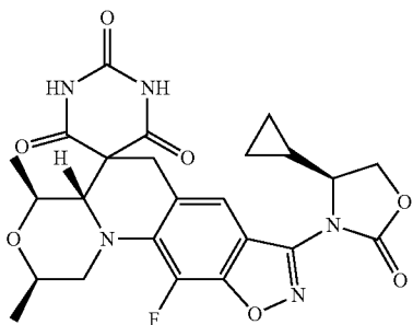
(2R,4S,4aS)-8-((S)-4-Cyclopropyl-2-oxooxazolidin-3-yl)-11-fluoro-2,4-dimethyl-2,4,4a,6-tetrahydro-1H,1'H-spiro[isoxazolo[4,5-g][1,4]oxazino[4,3-a]quinoline-5,5'-pyrimidine]-2',4',6'(3'H)-trione
