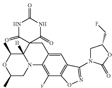
(2R,4S,4aS)-11-Fluoro-8-[(5R)-5-(fluoromethyl)-2-oxo-1,3-oxazolidin-3-yl]-2,4-dimethyl-1,2,4,4a-tetrahydro-2'H,6H-spiro[1,4-oxazino[4,3-a][1,2]oxazolo[4,5-g]quinoline-5,5'-pyrimidine]-2',4',6'(1'H,3'H)-trione
