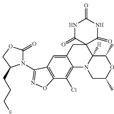
(2R,4S,4aS)-11-Chloro-8-((S)-4-(3-fluoropropyl)-2-oxooxazolidin-3-yl)-2,4-dimethyl-2,4,4a,6-tetrahydro-1H,1'H-spiro[isoxazolo[4,5-g][1,4]oxazino[4,3-a]quinoline-5,5'-pyrimidine]-2',4',6'(3'H)-trione
