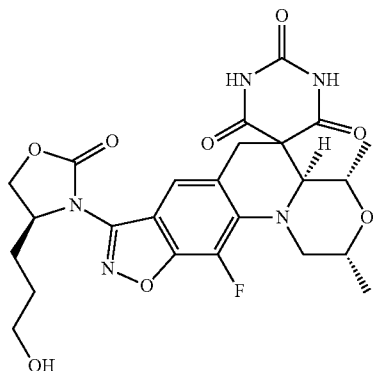
(2R,4S,4aS)-11-Fluoro-8-((S)-4-(3-hydroxypropyl)-2-oxooxazolidin-3-yl)-2,4-dimethyl-2,4,4a,6-tetrahydro-1H,1'H-spiro[isoxazolo[4,5-g][1,4]oxazino[4,3-a]quinoline-5,5'-pyrimidine]-2',4',6'(3'H)-trione
