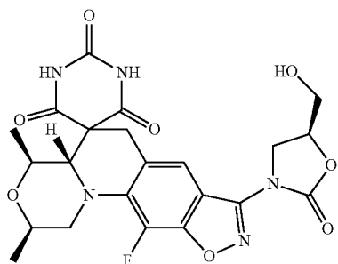
(2R,4S,4aS)-11-Fluoro-8-((S)-5-(hydroxymethyl)-2-oxooxazolidin-3-yl)-2,4-dimethyl-2,4,4a,6-tetrahydro-1H,1'H-spiro[isoxazolo[4,5-g][1,4]oxazino[4,3-a]quinoline-5,5'-pyrimidine]-2',4',6'(3'H)-trione
