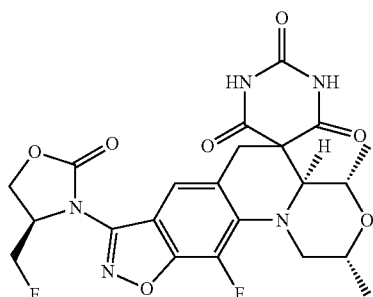
(2R,4S,4aS)-11-Fluoro-8-[(4R)-4-(fluoromethyl)-2-oxo-1,3-oxazolidin-3-yl]-2,4-dimethyl-1,2,4,4a-tetrahydro-2'H,6H-spiro[1,4-oxazino[4,3-a][1,2]oxazolo[4,5-g]quinoline-5,5'-pyrimidine]-2',4',6'(1'H,3'H)-trione
