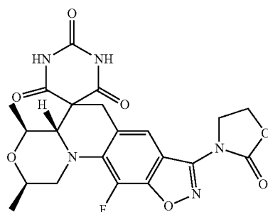
(2R,4S,4aS)-11-Fluoro-2,4-dimethyl-8-[(2-oxo-1,3-oxazolidin-3-yl)-1,2,4,4a-tetrahydro-2'H,6H-spiro[1,4-oxazino[4,3-a][1,2]oxazolo[4,5-g]quinoline-5,5'-pyrimidine]-2',4',6'(1'H,3'H)-trione
