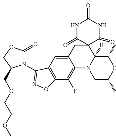
(2R,4S,4aS)-11-Fluoro-8-[(4S)-4-[(2-methoxyethoxy)methyl]-2-oxo-1,3-oxazolidin-3-yl]-2,4-dimethyl-1,2,4,4a-tetrahydro-2'H,6H-spiro[1,4-oxazino[4,3-a][1,2]oxazolo[4,5-g]quinoline-5,5'-pyrimidine]-2',4',6'(1'H,3'H)-trione
