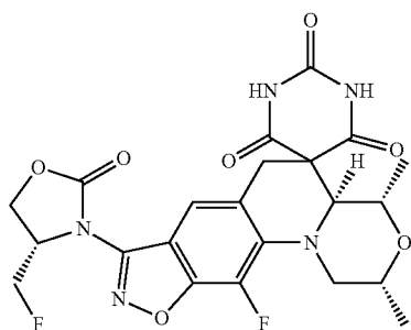
(2R,4S,4aS)-11-Fluoro-8-[(4S)-4-(fluoromethyl)-2-oxo-1,3-oxazolidin-3-yl]-2,4-dimethyl-1,2,4,4a-tetrahydro-2'H,6H-spiro[1,4-oxazino[4,3-a][1,2]oxazolo[4,5-g]quinoline-5,5'-pyrimidine]-2',4',6'(1'H,3'H)-trione
