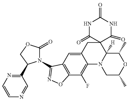
(2R,4S,4aS)-11-fluoro-2,4-dimethyl-8-((S)-2-oxo-4-(pyrazin-2-yl)oxazolidin-3-yl)-2,4,4a,6-tetrahydro-1H,1'H-spiro[isoxazolo[4,5-g][1,4]oxazino[4,3-a]quinoline-5,5'-pyrimidine]-2',4',6'(3'H)-trione
