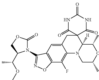
(2R,4S,4aS)-11-Fluoro-8-((R)-4-((R)-1-methoxyethyl)-2-oxooxazolidin-3-yl)-2,4-dimethyl-2,4,4a,6-tetrahydro-1H,1'H-spiro[isoxazolo[4,5-g][1,4]oxazino[4,3-a]quinoline-5,5'-pyrimidine]-2',4',6'(3'H)-trione
