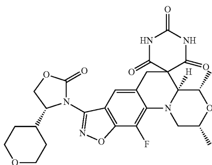
((2R,4S,4aS)-11-Fluoro-2,4-dimethyl-8-[(4R-(tetrahydro-2H-pyran-4-yl)-2-oxo-1,3-oxazolidin-3-yl]-1,2,4,4a-tetrahydro-2'H,6H-spiro[1,4-oxazino[4,3-a][1,2]oxazolo[4,5-g]quinoline-5,5'-pyrimidine]-2',4',6'(1'H,3'H)-trione
