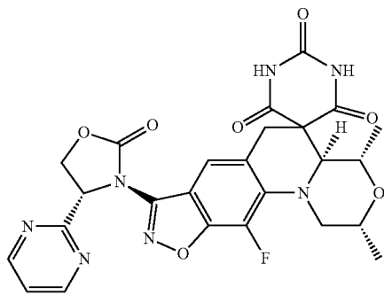
(2R,4S,4aS)-11-Fluoro-2,4-dimethyl-8-((R)-2-oxo-4-(pyrimidin-2-yl)oxazolidin-3-yl)-2,4,4a,6-tetrahydro-1H,1'H-spiro[isoxazolo[4,5-g][1,4]oxazino[4,3-a]quinoline-5,5'-pyrimidine]-2',4',6'(3'H)-trione
