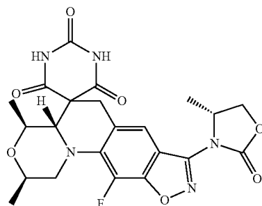
(2R,4S,4aS)-11-Fluoro-2,4-dimethyl-8-[(4R)-4-methyl-2-oxo-1,3-oxazolidin-3-yl]-1,2,4,4a-tetrahydro-2'H,6H-spiro[1,4-oxazino[4,3-a][1,2]oxazolo[4,5-g]quinoline-5,5'-pyrimidine]-2',4',6'(1'H,3'H)-trione
