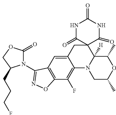
(2R,4S,4aS)-11-Fluoro-8-((S)-4-(3-fluoropropyl)-2-oxooxazolidin-3-yl)-2,4-dimethyl-2,4,4a,6-tetrahydro-1H,1'H-spiro[isoxazolo[4,5-g][1,4]oxazino[4,3-a]quinoline-5,5'-pyrimidine]-2',4',6'(3'H)-trione
