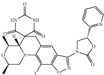
(2R,4S,4aS)-11-Fluoro-2,4-dimethyl-8-((R)-2-oxo-5-(pyridin-2-yl)oxazolidin-3-yl)-2,4,4a,6-tetrahydro-1H,1'H-spiro[isoxazolo[4,5-g][1,4]oxazino[4,3-a]quinoline-5,5'-pyrimidine]-2',4',6'(3'H)-trione
