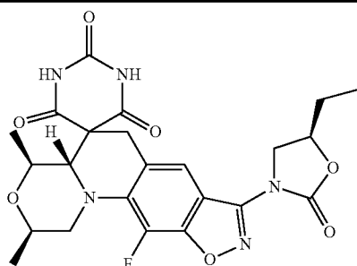
(2R,4S,4aS)-8-[(5R)-5-Ethyl-2-oxo-1,3-oxazolidin-3-yl]-11-fluoro-2,4-dimethyl-1,2,4,4a-tetrahydro-2'H,6H-spiro[1,4-oxazino[4,3-a][1,2]oxazolo[4,5-g]quinoline-5,5'-pyrimidine]-2',4',6'(1'H,3'H)-trione
