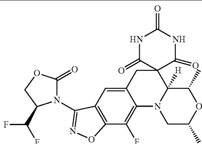
(2R,4S,4aS)-8-((R)-4-(Difluoromethyl)-2-oxooxazolidin-3-yl)-11-fluoro-2,4-dimethyl-2,4,4a,6-tetrahydro-1H,1'H-spiro[isoxazolo[4,5-g][1,4]oxazino[4,3-a]quinoline-5,5'-pyrimidine]-2',4',6'(3'H)-trione
