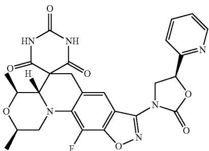
(2R,4S,4aS)-11-fluoro-2,4-dimethyl-8-((S)-2-oxo-5-(pyridin-2-yl)oxazolidin-3-yl)-2,4,4a,6-tetrahydro-1H,1'H-spiro[isoxazolo[4,5-g][1,4]oxazino[4,3-a]quinoline-5,5'-pyrimidine]-2',4',6'(3'H)-trione
