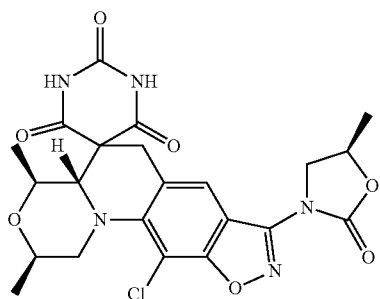
((2R,4S,4aS)-11-Chloro-2,4-dimethyl-8-((R)-5-methyl-2-oxooxazolidin-3-yl)-2,4,4a,6-tetrahydro-1H,1'H-spiro[isoxazolo[4,5-g][1,4]oxazino[4,3-a]quinoline-5,5'-pyrimidine]-2',4',6'(3'H)-trione
