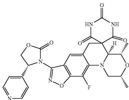
(2R,4S,4aS)-11-Fluoro-2,4-dimethyl-8-((R)-2-oxo-4-(pyridin-4-yl)oxazolidin-3-yl)-2,4,4a,6-tetrahydro-1H,1'H-spiro[isoxazolo[4,5-g][1,4]oxazino[4,3-a]quinoline-5,5'-pyrimidine]-2',4',6'(3'H)-trione
