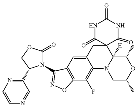
(2R,4S,4aS)-11-Fluoro-2,4-dimethyl-8-((R)-2-oxo-4-(pyrazin-2-yl)oxazolidin-3-yl)-2,4,4a,6-tetrahydro-1H,1'H-spiro[isoxazolo[4,5-g][1,4]oxazino[4,3-a]quinoline-5,5'-pyrimidine]-2',4',6'(3'H)-trione
