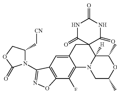
{(4S)-3-[(2R,4S,4aS)-11-Fluoro-2,4-dimethyl-2',4',6'-trioxo-1,1',2,3',4,4',4a,6'-octahydro-2'H,6H-spiro[1,4-oxazino[4,3-a][1,2]oxazolo[4,5-g]quinoline-5,5'-pyrimidin]-8-yl]-2-oxo-1,3-oxazolidin-4-yl}acetonitrile
