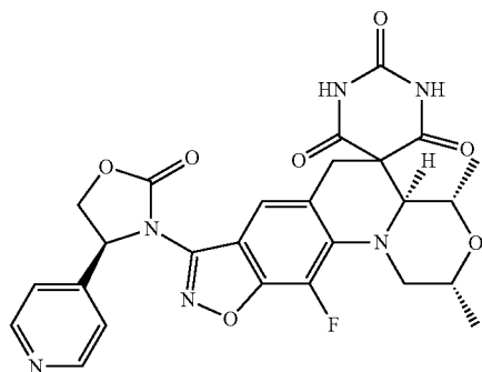
(2R,4S,4aS)-11-fluoro-2,4-dimethyl-8-((S)-2-oxo-4-(pyridin-4-yl)oxazolidin-3-yl)-2,4,4a,6-tetrahydro-1H,1'H-spiro[isoxazolo[4,5-g][1,4]oxazino[4,3-a]quinoline-5,5'-pyrimidine]-2',4',6'(3'H)-trione
