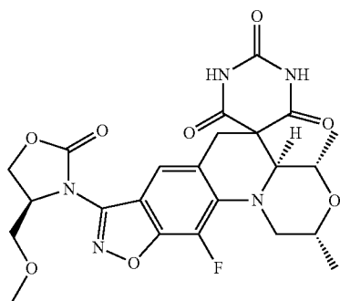
(2R,4S,4aS)-11-Fluoro-8-[(4S)-4-(methoxymethyl)-2-oxo-1,3-oxazolidin-3-yl]-2,4-dimethyl-1,2,4,4a-tetrahydro-2'H,6H-spiro[1,4-oxazino[4,3-a][1,2]oxazolo[4,5-g]quinoline-5,5'-pyrimidine]-2',4',6'(1'H,3'H)-trione
