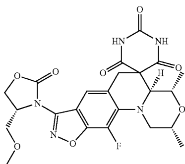
(2R,4S,4aS)-11-Fluoro-8-[(4R)-4-(methoxymethyl)-2-oxo-1,3-oxazolidin-3-yl]-2,4-dimethyl-1,2,4,4a-tetrahydro-2'H,6H-spiro[1,4-oxazino[4,3-a][1,2]oxazolo[4,5-g]quinoline-5,5'-pyrimidine]-2',4',6'(1'H,3'H)-trione
