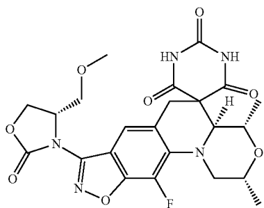
(2R,4S,4aS)-11-Fluoro-8-[(4S)-4-(methoxymethyl)-2-oxo-1,3-oxazolidin-3-yl]-2,4-dimethyl-1,2,4,4a-tetrahydro-2'H,6'H-spiro[1,4-oxazino[4,3-a][1,2]oxazolo[4,5-g]quinoline-5,5'-pyrimidine]-2',4',6'(1'H,3'H)-trione
