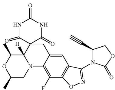
(2R,4S,4aS)-8-((S)-4-Ethynyl-2-oxooxazolidin-3-yl)-11-fluoro-2,4-dimethyl-2,4,4a,6-tetrahydro-1H,1'H-spiro[isoxazolo[4,5-g][1,4]oxazino[4,3-a]quinoline-5,5'-pyrimidine]-2',4',6'(3'H)-trione
