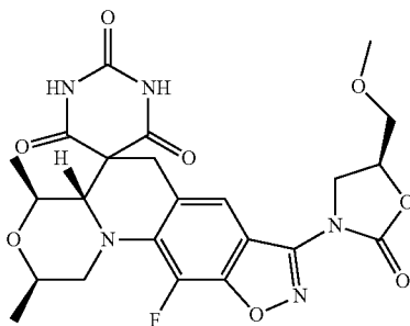
(2R,4S,4aS)-11-Fluoro-8-[(5S)-4-(methoxymethyl)-2-oxo-1,3-oxazolidin-3-yl]-2,4-dimethyl-1,2,4,4a-tetrahydro-2'H,6'H-spiro[1,4-oxazino[4,3-a][1,2]oxazolo[4,5-g]quinoline-5,5'-pyrimidine]-2',4',6'(1'H,3'H)-trione
