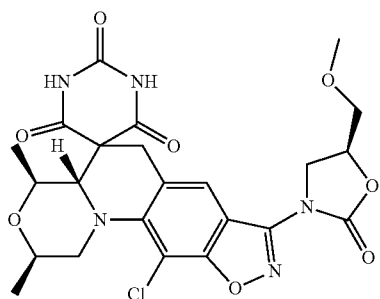
(2R,4S,4aS)-11-Chloro-8-[(5S)-4-(methoxymethyl)-2-oxo-1,3-oxazolidin-3-yl]-2,4-dimethyl-1,2,4,4a-tetrahydro-2'H,6H-spiro[1,4-oxazino[4,3-a][1,2]oxazolo[4,5-g]quinoline-5,5'-pyrimidine]-2',4',6'(1'H,3'H)-trione
