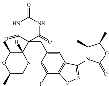
(2R,4S,4aS)-8-((4S,5R)-4,5-Dimethyl-2-oxooxazolidin-3-yl)-11-fluoro-2,4-dimethyl-2,4,4a,6-tetrahydro-1H,1'H-spiro[isoxazolo[4,5-g][1,4]oxazino[4,3-a]quinoline-5,5'-pyrimidine]-2',4',6'(3'H)-trione
