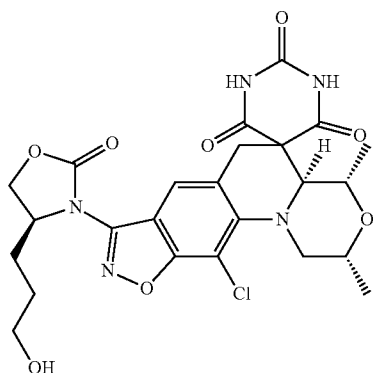
(2R,4S,4aS)-11-Chloro-8-((S)-4-(3-hydroxypropyl)-2-oxooxazolidin-3-yl)-2,4-dimethyl-2,4,4a,6-tetrahydro-1H,1'H-spiro[isoxazolo[4,5-g][1,4]oxazino[4,3-a]quinoline-5,5'-pyrimidine]-2',4',6'(3'H)-trione
