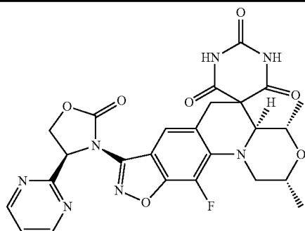
(2R,4S,4aS)-11-fluoro-2,4-dimethyl-8-((S)-2-oxo-4-(pyrimidin-2-yl)oxazolidin-3-yl)-2,4,4a,6-tetrahydro-1H,1'H-spiro[isoxazolo[4,5-g][1,4]oxazino[4,3-a]quinoline-5,5'-pyrimidine]-2',4',6'(3'H)-trione
