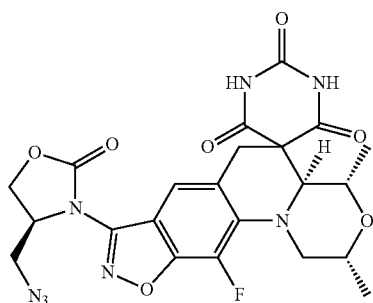
(2R,4S,4aS)-8-((S)-4-(azidomethyl)-2-oxooxazolidin-3-yl)-11-fluoro-2,4-dimethyl-2,4,4a,6-tetrahydro-1H,1'H-spiro[isoxazolo[4,5-g][1,4]oxazino[4,3-a]quinoline-5,5'-pyrimidine]-2',4',6'(3'H)-trione
