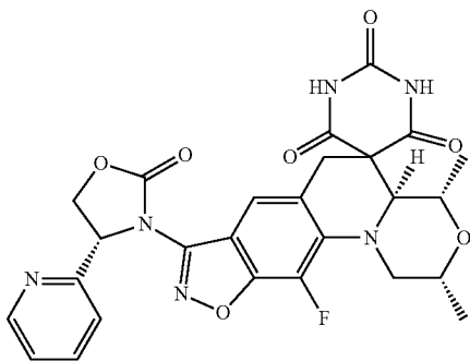
(2R,4S,4aS)-11-Fluoro-2,4-dimethyl-8-((R)-2-oxo-4-(pyridin-2-yl)oxazolidin-3-yl)-2,4,4a,6-tetrahydro-1H,1'H-spiro[isoxazolo[4,5-g][1,4]oxazino[4,3-a]quinoline-5,5'-pyrimidine]-2',4',6'(3'H)-trione
