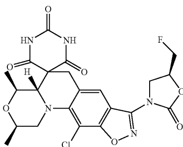
(2R,4S,4aS)-11-Chloro-8-((S)-5-(fluoromethyl)-2-oxooxazolidin-3-yl)-2,4-dimethyl-2,4,4a,6-tetrahydro-1H,1'H-spiro[isoxazolo[4,5-g][1,4]oxazino[4,3-a]quinoline-5,5'-pyrimidine]-2',4',6'(3'H)-trione
