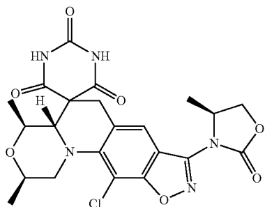
(2R,4S,4aS)-11-Chloro-2,4-dimethyl-8-((S)-4-methyl-2-oxooxazolidin-3-yl)-2,4,4a,6-tetrahydro-1H,1'H-spiro[isoxazolo[4,5-g][1,4]oxazino[4,3-a]quinoline-5,5'-pyrimidine]-2',4',6'(3'H)-trione
