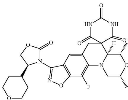
(2R,4S,4aS)-11-fluoro-2,4-dimethyl-8-[(4S-(tetrahydro-2H-pyran-4-yl)-2-oxo-1,3-oxazolidin-3-yl]-1,2,4,4a-tetrahydro-2'H,6H-spiro[1,4-oxazino[4,3-a][1,2]oxazolo[4,5-g]quinoline-5,5'-pyrimidine]-2',4',6'(1'H,3'H)-trione
