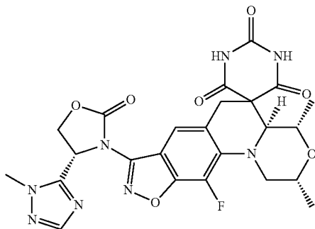
(2R,4S,4aS)-11-Fluoro-2,4-dimethyl-8-((R)-4-(1-methyl-1H-1,2,4-triazol-5-yl)-2-oxooxazolidin-3-yl)-2,4,4a,6-tetrahydro-1H,1'H-spiro[isoxazolo[4,5-g][1,4]oxazino[4,3-a]quinoline-5,5'-pyrimidine]-2',4',6'(3'H)-trione
