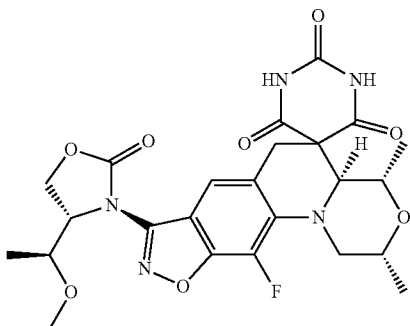
(2R,4S,4aS)-11-Fluoro-8-((R)-4-((S)-1-methoxyethyl)-2-oxooxazolidin-3-yl)-2,4-dimethyl-2,4,4a,6-tetrahydro-1H,1'H-spiro[isoxazolo[4,5-g][1,4]oxazino[4,3-a]quinoline-5,5'-pyrimidine]-2',4',6'(3'H)-trione
