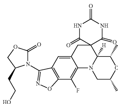
(2R,4S,4aS)-11-Fluoro-8-((S)-4-(2-hydroxyethyl)-2-oxooxazolidin-3-yl)-2,4-dimethyl-2,4,4a,6-tetrahydro-1H,1'H-spiro[isoxazolo[4,5-g][1,4]oxazino[4,3-a]quinoline-5,5'-pyrimidine]-2',4',6'(3'H)-trione
