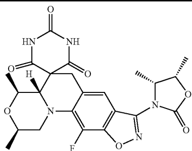
(2R,4S,4aS)-8-((4R,5S)-4,5-Dimethyl-2-oxooxazolidin-3-yl)-11-fluoro-2,4-dimethyl-2,4,4a,6-tetrahydro-1H,1'H-spiro[isoxazolo[4,5-g][1,4]oxazino[4,3-a]quinoline-5,5'-pyrimidine]-2',4',6'(3'H)-trione
