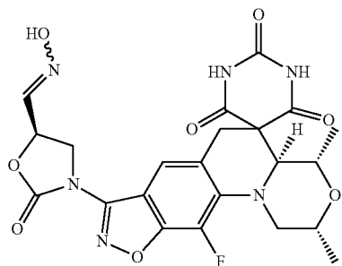
(2R,4S,4aS)-11-Fluoro-8-[(5R)-5-[(hydroxyimino)methyl]-2-oxo-1,3-oxazolidin-3-yl]-2,4-dimethyl-1,2,4,4a-tetrahydro-2'H,6H-spiro[1,4-oxazino[4,3a][1,2]oxazolo[4,5-g]quinoline-5,5'-pyrimidine]-2',4',6'(1'H,3'H)-trione
