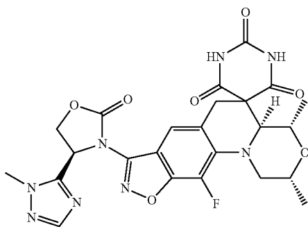
(2R,4S,4aS)-11-Fluoro-2,4-dimethyl-8-((S)-4-(1-methyl-1H-1,2,4-triazol-5-yl)-2-oxooxazolidin-3-yl)-2,4,4a,6-tetrahydro-1H,1'H-spiro[isoxazolo[4,5-g][1,4]oxazino[4,3-a]quinoline-5,5'-pyrimidine]-2',4',6'(3'H)-trione
