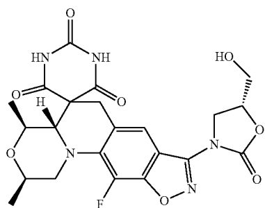
(2R,4S,4aS)-11-Fluoro-8-[(5R)-5-(hydroxymethyl)-2-oxo-1,3-oxazolidin-3-yl]-2,4-dimethyl-1,2,4,4a-tetrahydro-2'H,6H-spiro[1,4-oxazino[4,3-a][1,2]oxazolo[4,5-g]quinoline-5,5'-pyrimidine]-2',4',6'(1'H,3'H)-trione
