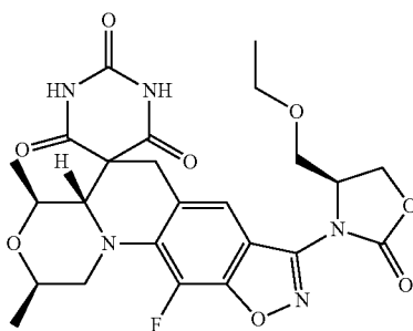
(2R,4S,4aS)-8-[(4S)-4-(Ethoxymethyl)-2-oxo-1,3-oxazolidin-3-yl]-11-fluoro-2,4-dimethyl-1,2,4,4a-tetrahydro-2'H,6H-spiro[1,4-oxazino[4,3-a][1,2]oxazolo[4,5-g]quinoline-5,5'-pyrimidine]-2',4',6'(1'H,3'H)-trione
