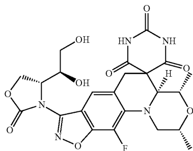
(2R,4S,4aS)-8-((R)-4-((S)-1,2-Dihydroxyethyl)-2-oxooxazolidin-3-yl)-11-fluoro-2,4-dimethyl-2,4,4a,6-tetrahydro-1H,1'H-spiro[isoxazolo[4,5-g][1,4]oxazino[4,3-a]quinoline-5,5'-pyrimidine]-2',4',6'(3'H)-trione
