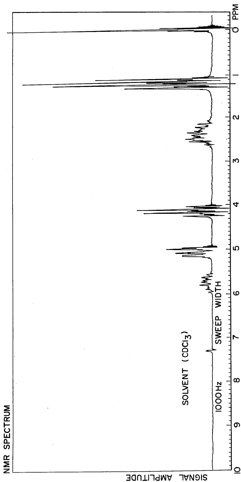
FIG. 1 EXAMPLE I Ethyl-2-methyl-4-pentenoate
