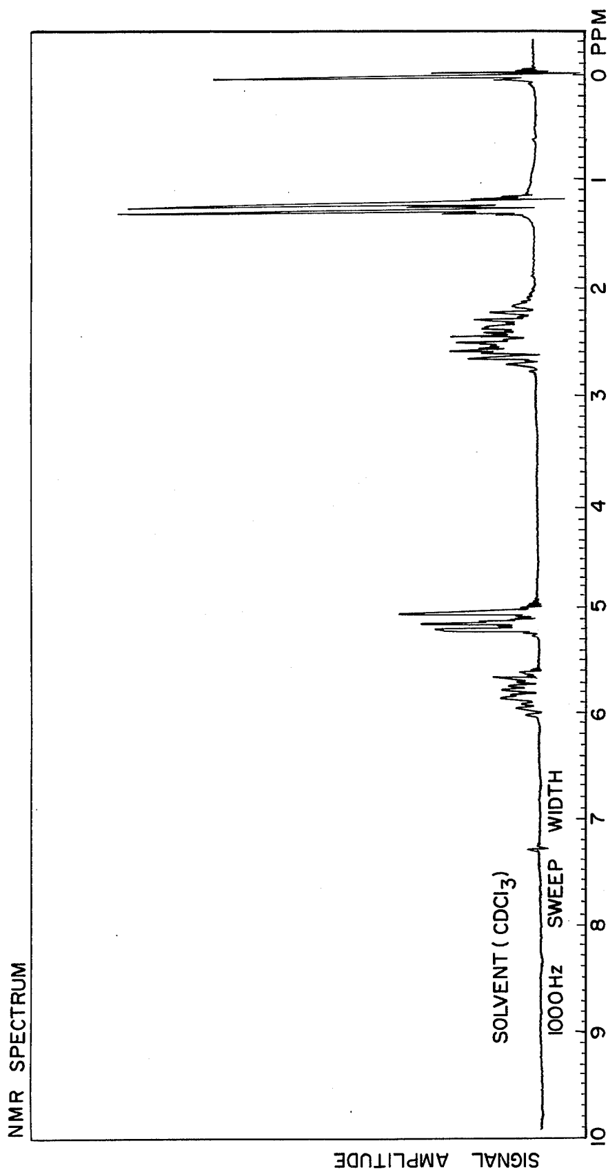
FIG. 3 EXAMPLE II 2-methyl-4-pentenoic acid
