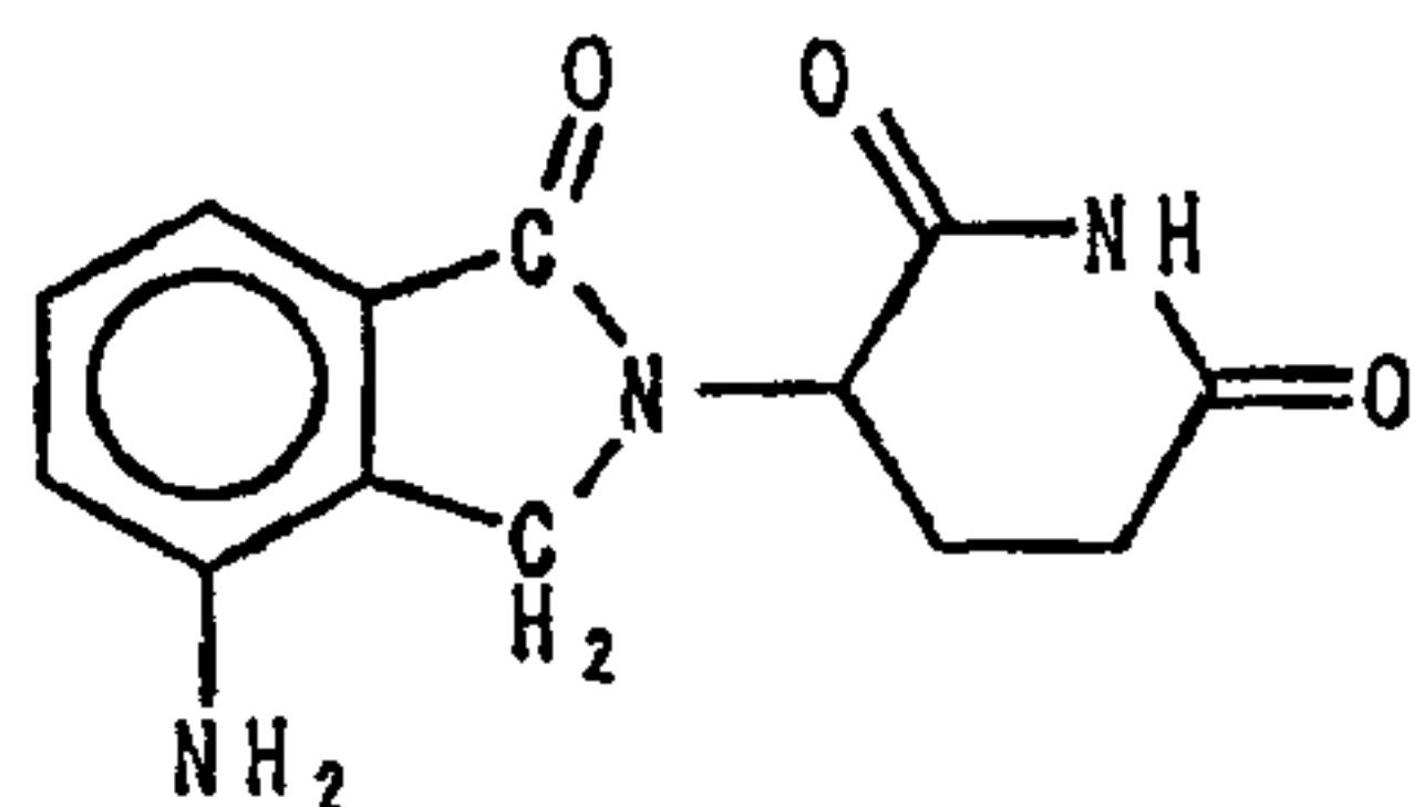
1-oxo-2-(2,6-dioxopiperidin-3-yl)-4-aminoisoindoline;
