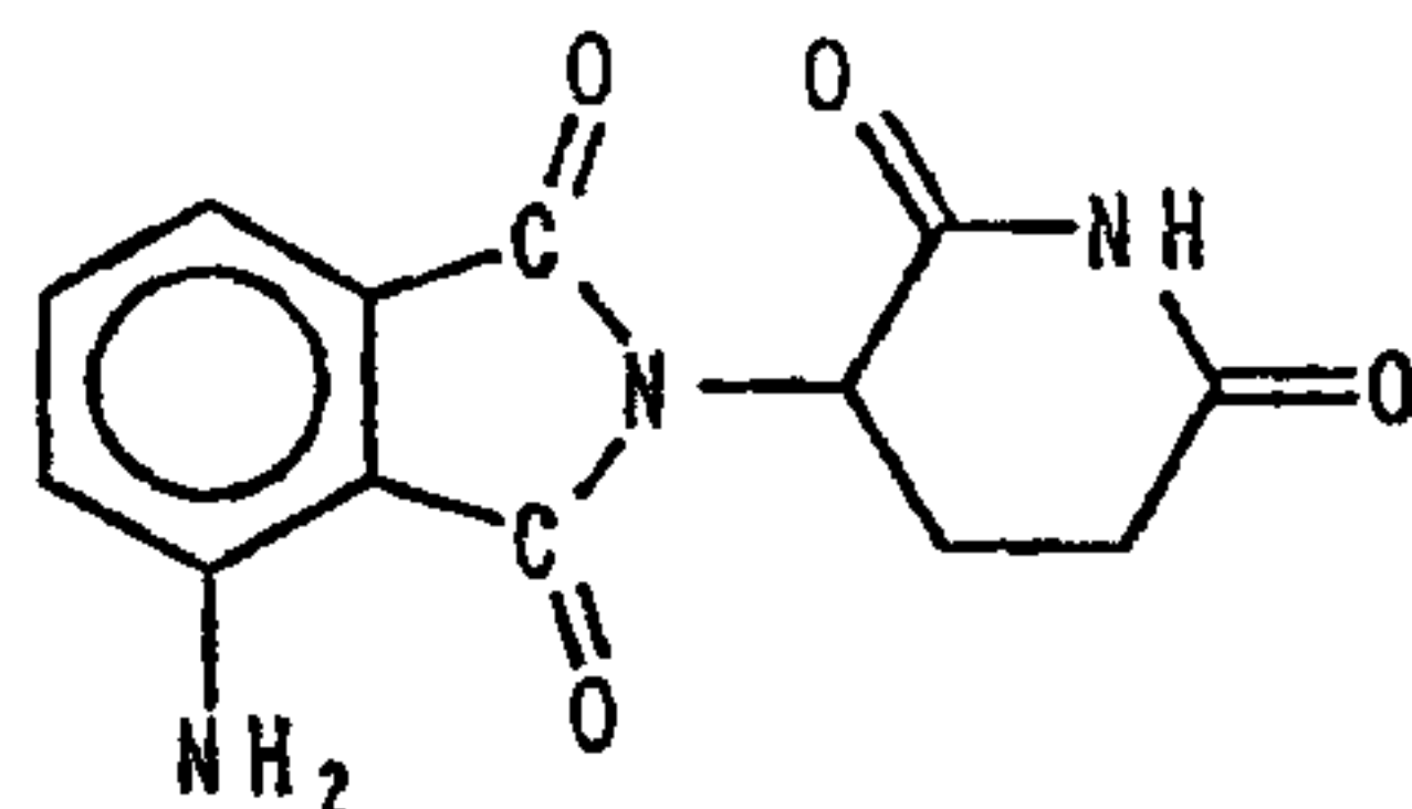
1,3-dioxo-2-(2,6-dioxopiperidin-3-yl)-4-aminoisoindoline;
