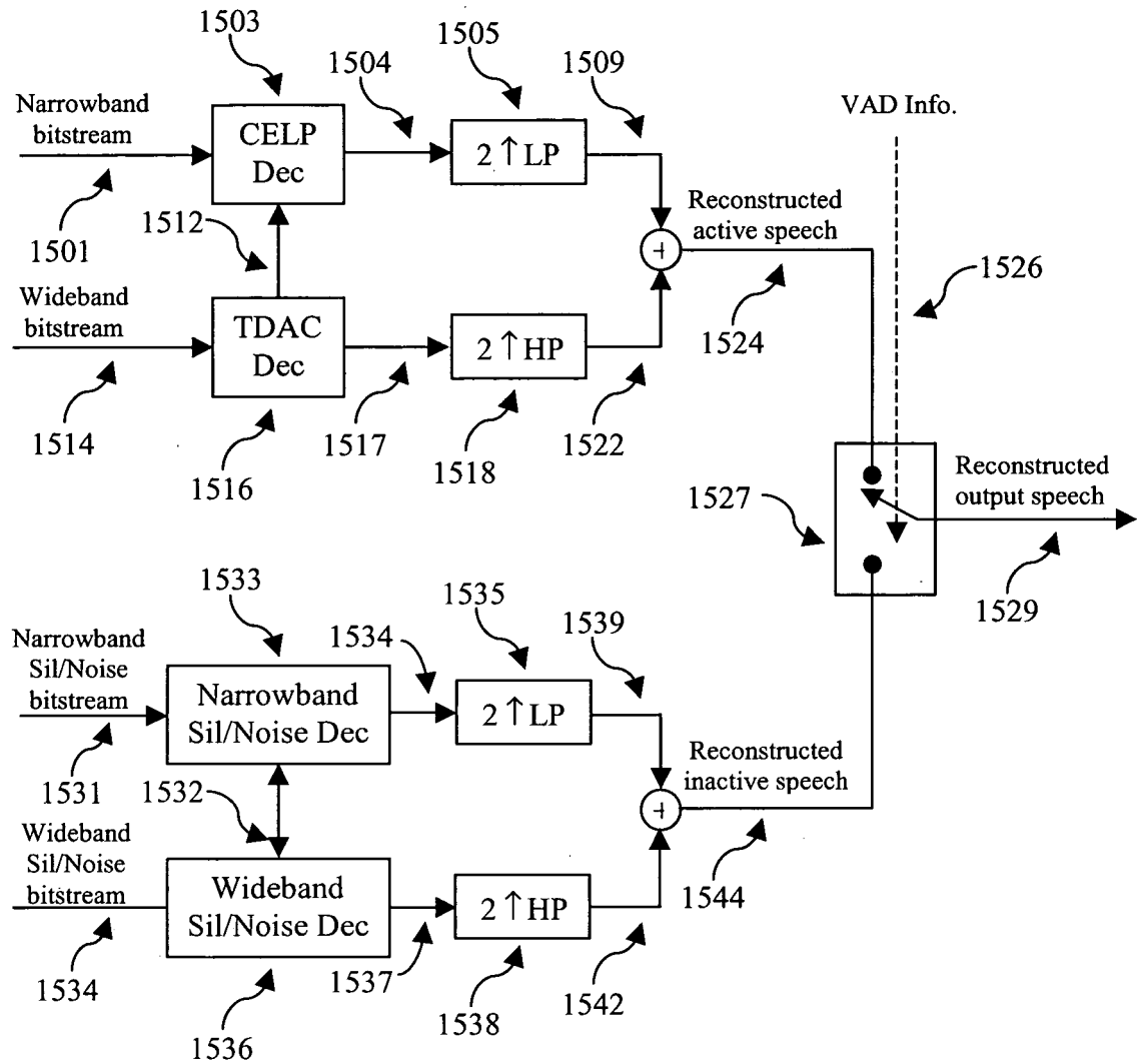
Figure 15: G.729.1 Decoder with an Embedded Silence/Background-Noise Compression
