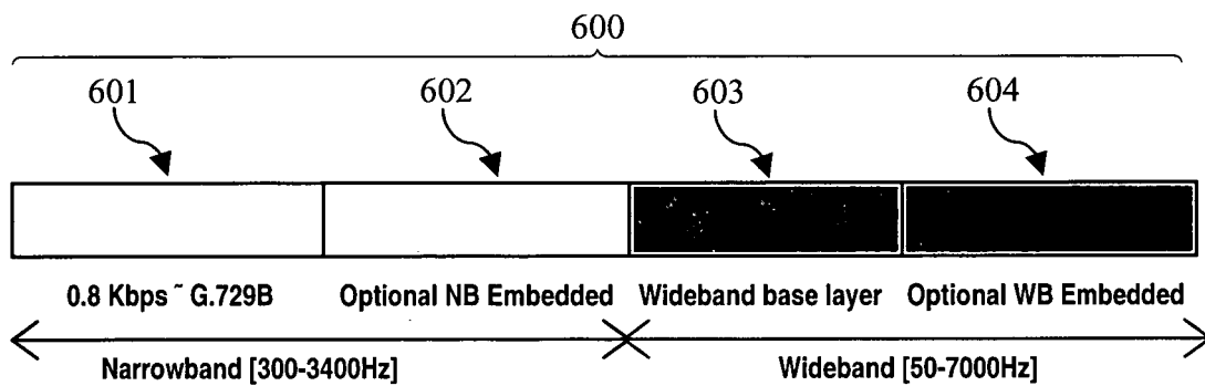
Figure 6: Silence/Background-Noise Embedded Bitstream
