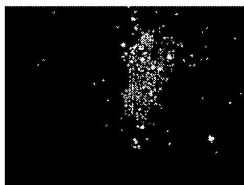
beta-D-thio-LNA; 2746
