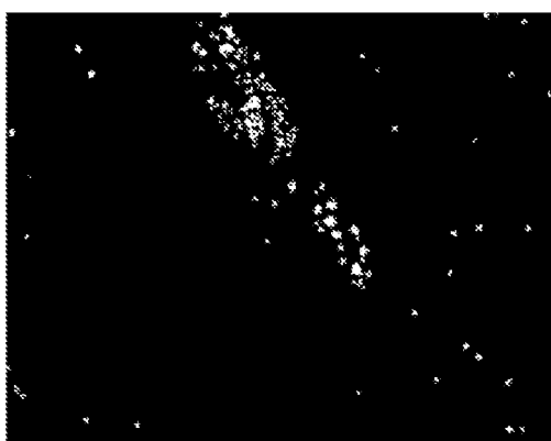
beta-D-oxy-LNA; 2740
