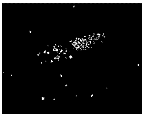
alpha-L-oxy-LNA; 2774
