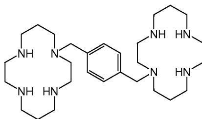
AMD3100
