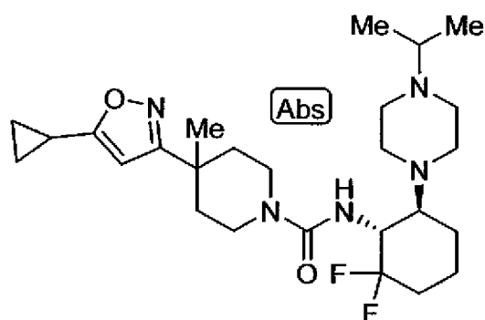
4-(5-cyclopropyl-1,2,4-oxadiazol-3-yl)-N-((1R,6S)-2,2-
