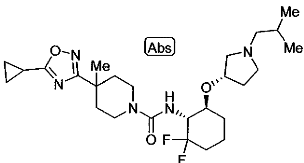
N-[(1R,6S)-6-{[(3S)-1-(cyclopropylmethyl)pyrrolidin-3-yl]oxy}-2,2-difluorocyclohexyl]-4-{5-[(1S,2S)-2-fluorocyclopropyl]-1,2,4-oxadiazol-3-yl}-4-methylpiperidine-1-carboxamide
