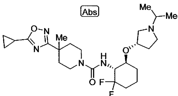
N-[(1R,6S)-2,2-difluoro-6-[[ (3S)-1-(propan-2-yl)pyrrolidin-3-yl]oxy]cyclohexyl]-4-{5-[(1S,2S)-2-fluorocyclopropyl]-1,2,4-oxadiazol-3-yl}-4-methylpiperidine-1-carboxamide
