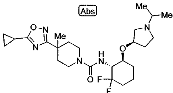
N-[(1R,6S)-2,2-difluoro-6-[[ (3R)-1-(propan-2-yl)pyrrolidin-3-yl]oxy]cyclohexyl]-4-methyl-4-(4-methylphenyl)piperidine-1-carboxamide
