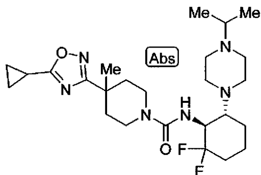
4-(5-cyclopropyl-1,2,4-oxadiazol-3-yl)-N-((1R,6S)-2,2-difluoro-6-[4-(propan-2-yl)piperazin-1-yl]cyclohexyl)-4-methylpiperidine-1-carboxamide
