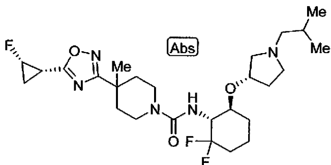
4-(5-cyclopropyl-1,2,4-oxadiazol-3-yl)-N-[(1R,6S)-2,2-difluoro-6-{[(3S)-1-(2-methylpropyl)pyrrolidin-3-yl]oxy}cyclohexyl]-4-methylpiperidine-1-carboxamide
