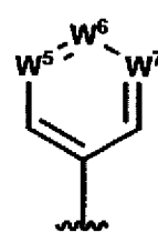
(1b-4)
