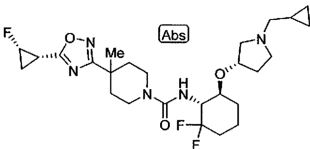
4-(5-cyclopropyl-1,2,4-oxadiazol-3-yl)-N-[(1R,6S)-6-{[(3S)-1-(2,2-dimethylpropyl)pyrrolidin-3-yl]oxy}-2,2-difluorocyclohexyl]-4-methylpiperidine-1-carboxamide
