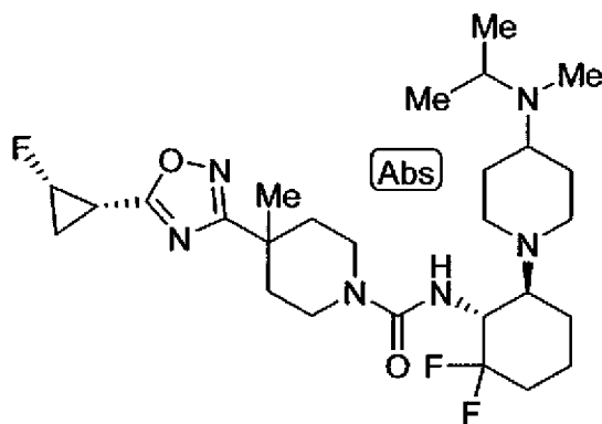
N-[(1R,6S)-6-{(3S)-3-[cyclopropyl(methyl)amino]pyrrolidin-1-yl}-2,2-difluorocyclohexyl]-4-{5-[(1S,2S)-2-fluorocyclopropyl]-1,2,4-oxadiazol-3-yl}-4-methylpiperidine-1-carboxamide
