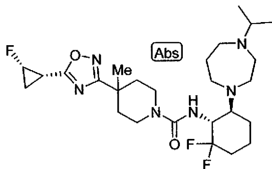
4-{5-[(1S,2S)-2-fluorocyclopropyl]-1,2,4-oxadiazol-3- yl}-N-({(1R,2S,6S)-2-fluoro-6-[4-(propan-2-yl)piperazin-1-
