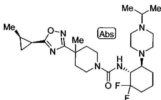
Example 69: N-((1R,6S)-2,2-difluoro-6-[4-(propan-2-yl)piperazin-1-yl]cyclohexyl)-4-methyl-4-{5-[(1R,2S)-2-methylcyclopropyl]-1,2,4-oxadiazol-3-yl}piperidine-1-carboxamide
