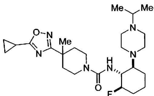
Example 152: N-[(1R,6S)-2,2-difluoro-6-[4-(propan-2-
