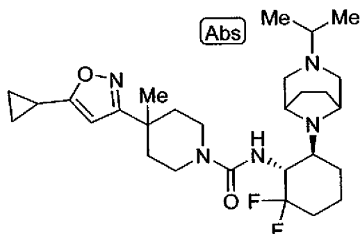
Example 66: N-((1R,6S)-2,2-difluoro-6-[4-(propan-2-
