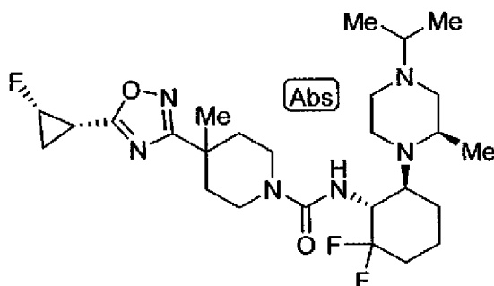
Example 112: N-[(1R,6S)-2,2-difluoro-6-((3R)-3-
