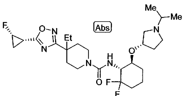
Example 107: N-[(1R,6S)-2,2-difluoro-6-{[(3S)-1-(2-methylpropyl)pyrrolidin-3-yl]oxy}cyclohexyl]-4-(5-{[(1S,2S)-2-fluorocyclopropyl]-1,2,4-oxadiazol-3-yl}-4-methylpiperidine-1-carboxamide
