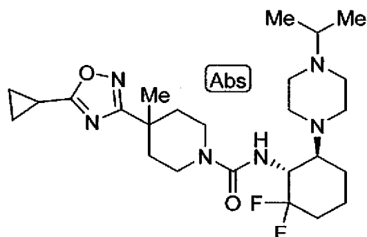
4-(5-cyclopropyl-1,2-oxazol-3-yl)-N-((1R,6S)-2,2-difluoro-6-[4-(propan-2-yl)piperazin-1-yl]cyclohexyl)-4-methylpiperidine-1-carboxamide
