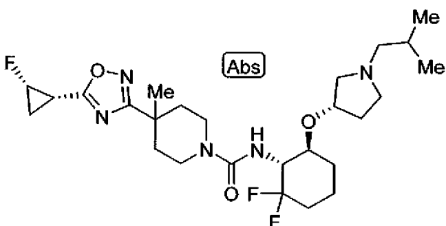
Example 116: 4-(5-cyclopropyl-1,2,4-oxadiazol-3-yl)-N-[(1R,6S)-2,2-difluoro-6-{[(3S)-1-(2-methylpropyl)pyrrolidin-3-yl]oxy}cyclohexyl]-4-methylpiperidine-1-carboxamide
