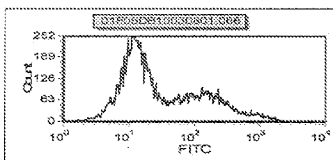
CRLR L24-Q33: RAMP1
