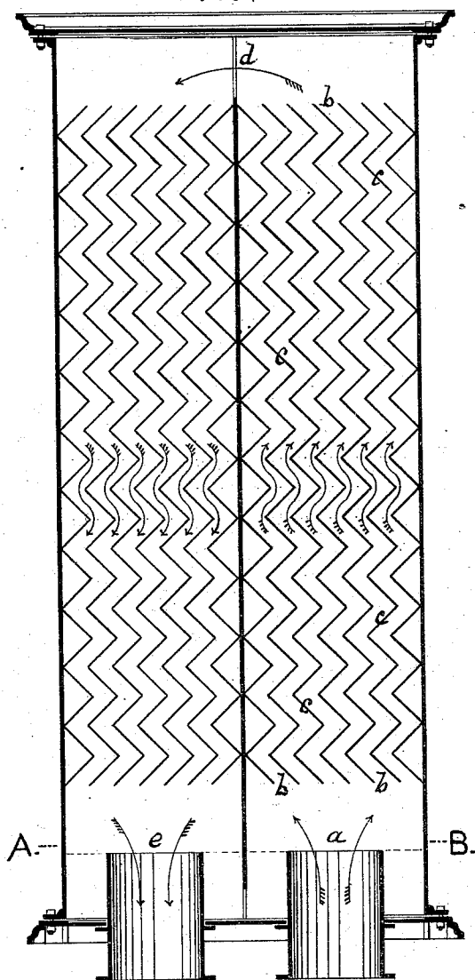
— LONGITUDINAL SECTION. —
