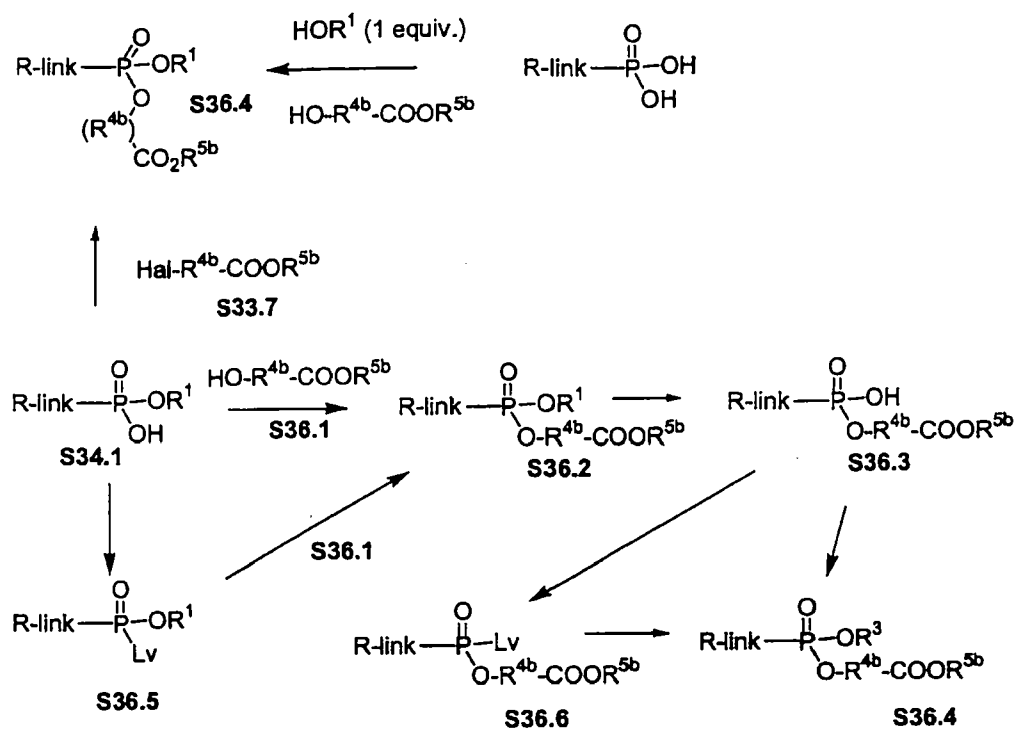
Scheme 36
