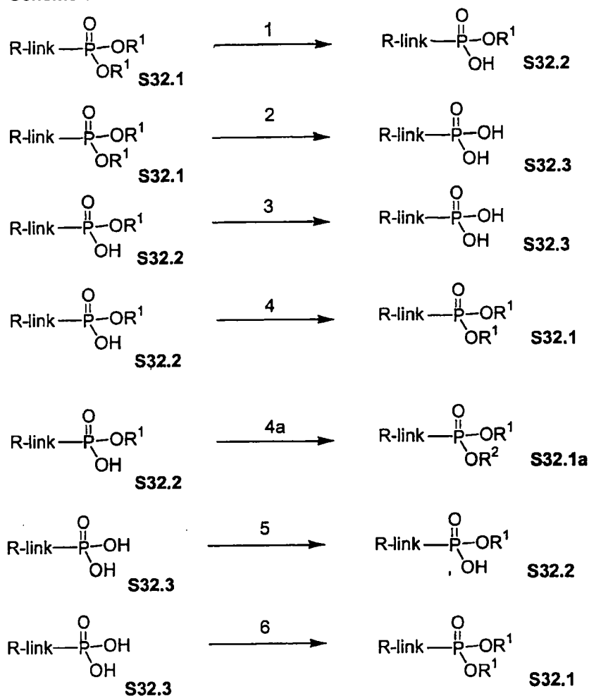
Scheme 32
