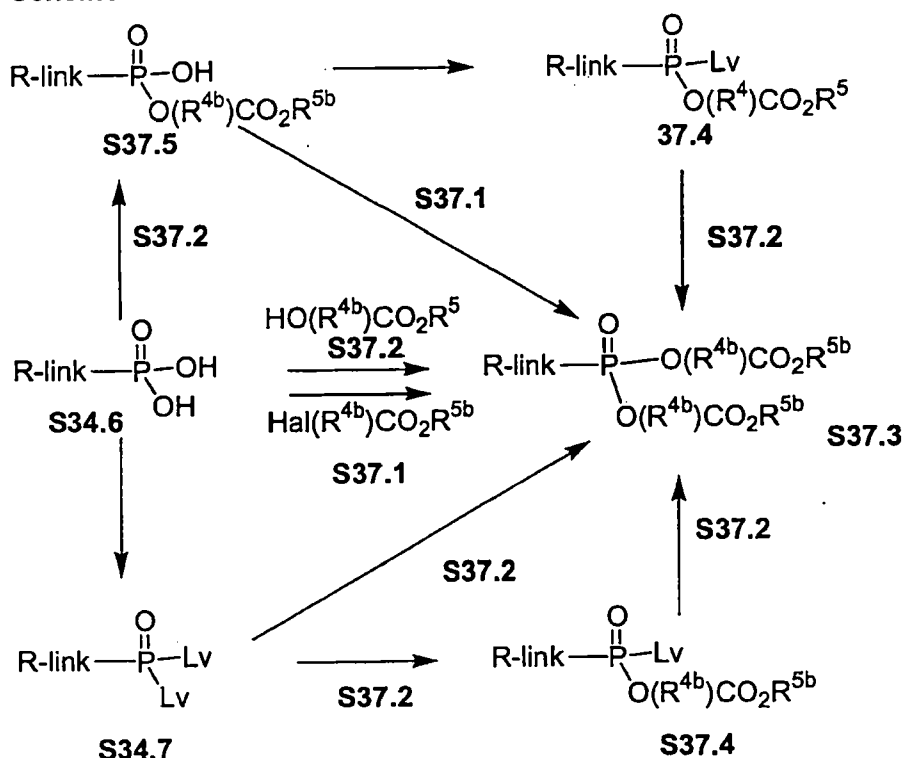
Scheme 37
