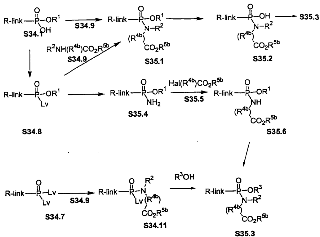
Scheme 35
