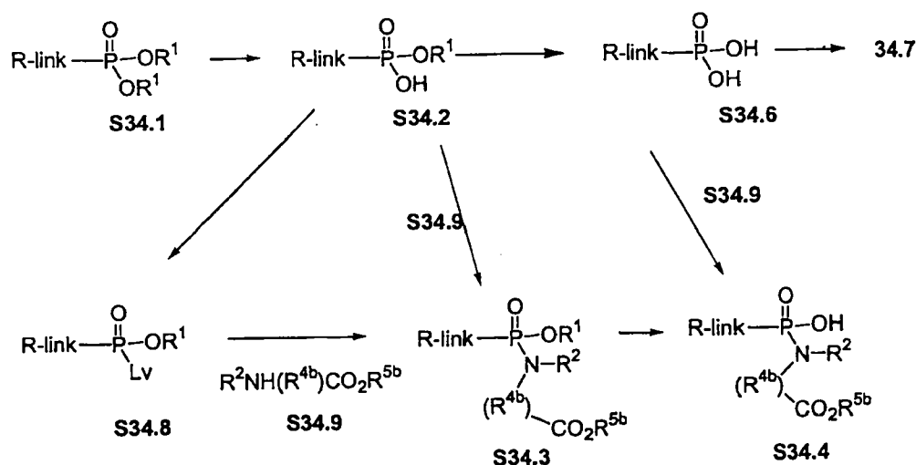
Scheme 34
