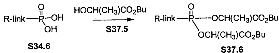
Scheme 37 Example 2
