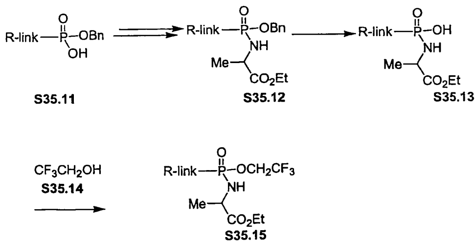
Scheme 35 Example 2
