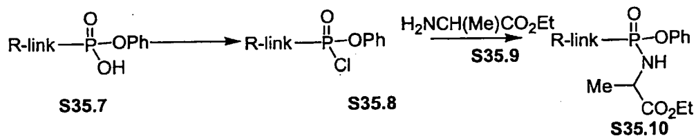
Scheme 35 Example 2
