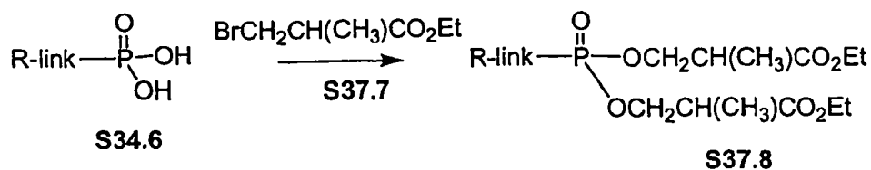
Scheme 37 Example 2
