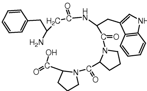
II-3-d ( \text{H}_2\text{N-}\beta^3\text{hoPhe-Trp-Pro-Pro-OH} ),
