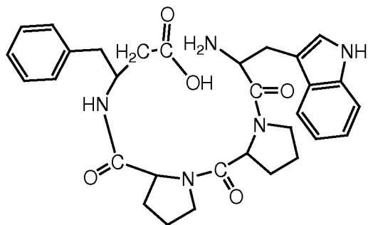
II-2-d ( \text{H-Pro-Pro-}\beta^3\text{hoPhe-Trp-OH} ),
