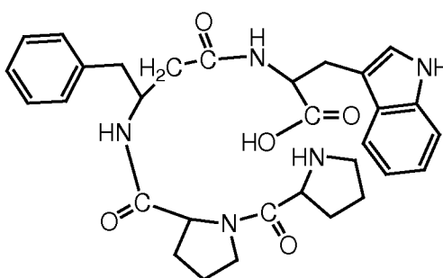
II-1-d ( \text{H-Pro-Pro-}\beta^3\text{hoPhe-Trp-OH} ),
