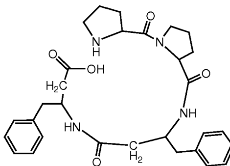
II-1-c ( \text{H-Pro-Pro-}\beta^3\text{hoPhe-}\beta^3\text{hoPhe-OH} ),
