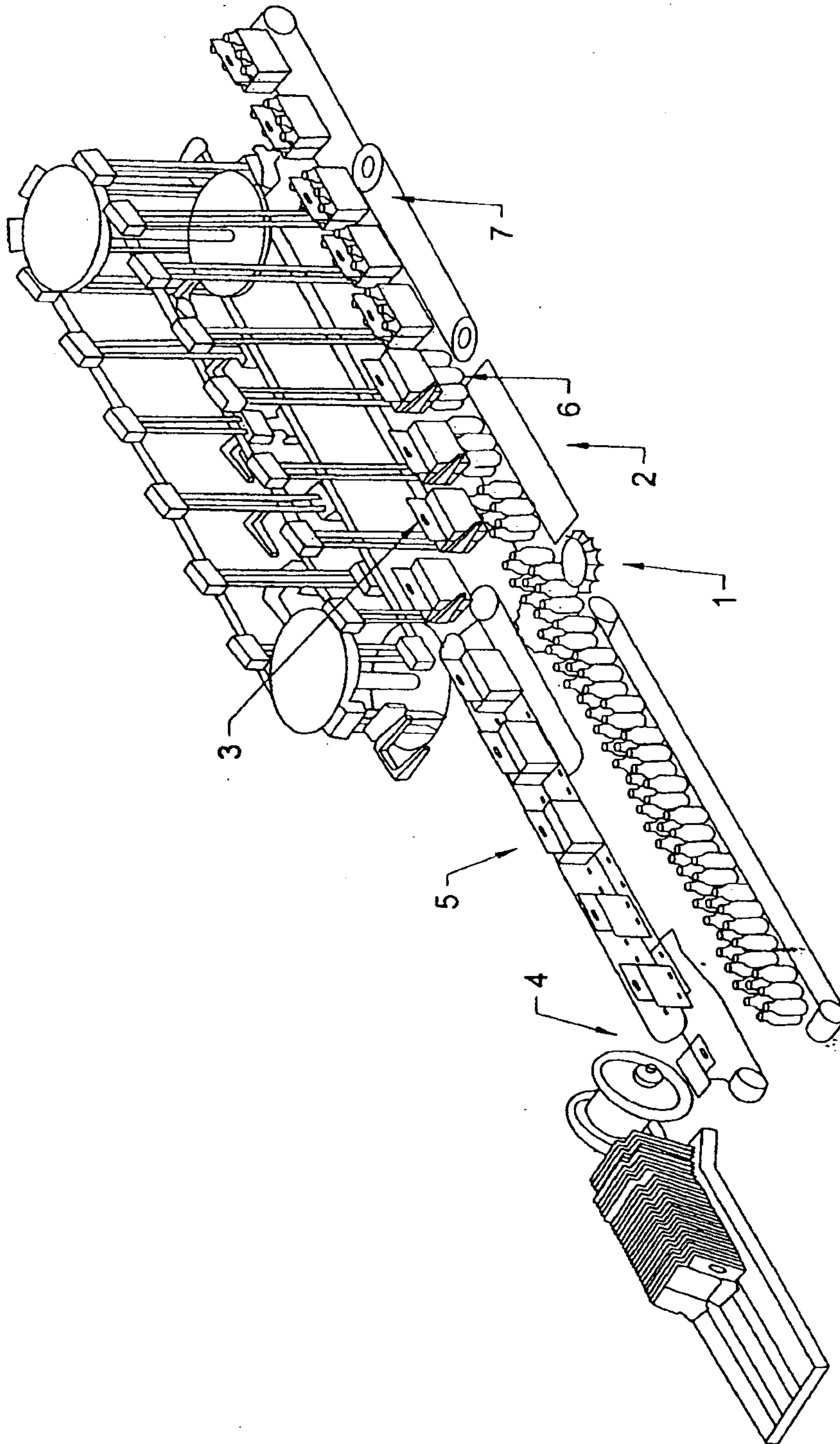
Fig. 1 (PRIOR ART)
