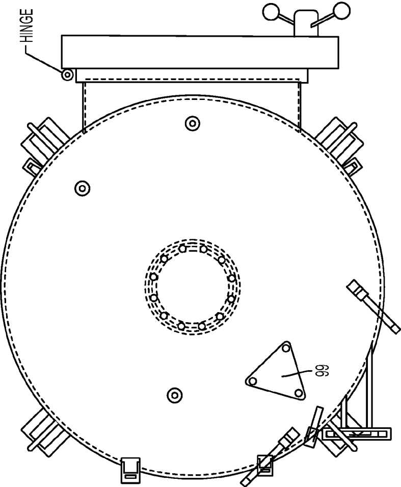
PLAN VIEW FIG. 11B
