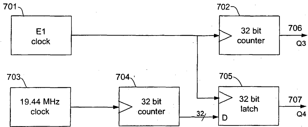
ATM 155 ICU counter structure
