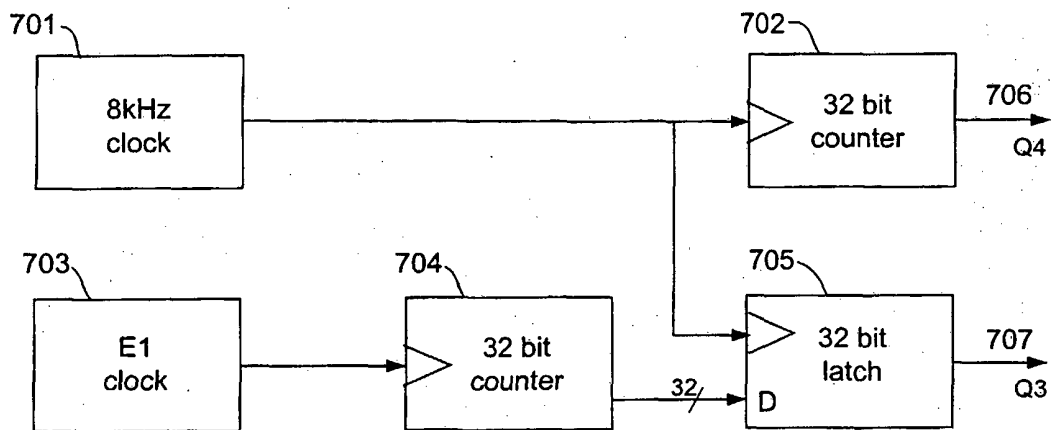
ATM 25 ICU counter structure
