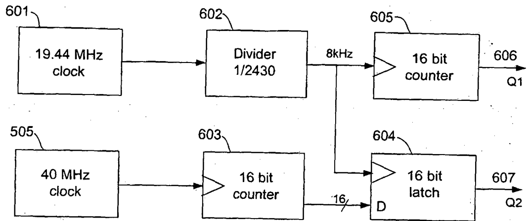
MAC counter structure for ATM 155 ODU
