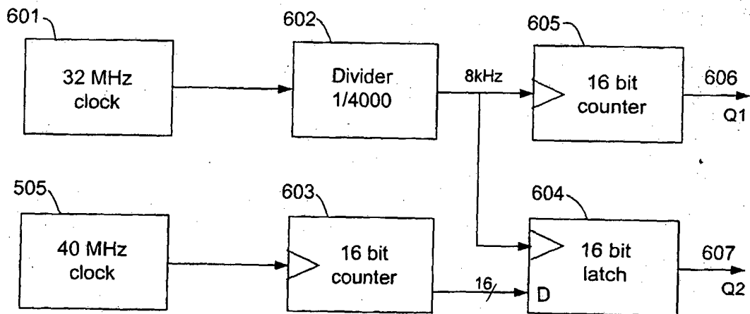
MAC counter structure for ATM 25 ODU
