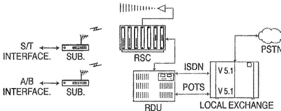
ISDN AND POTS NETWORK INTERFACE
