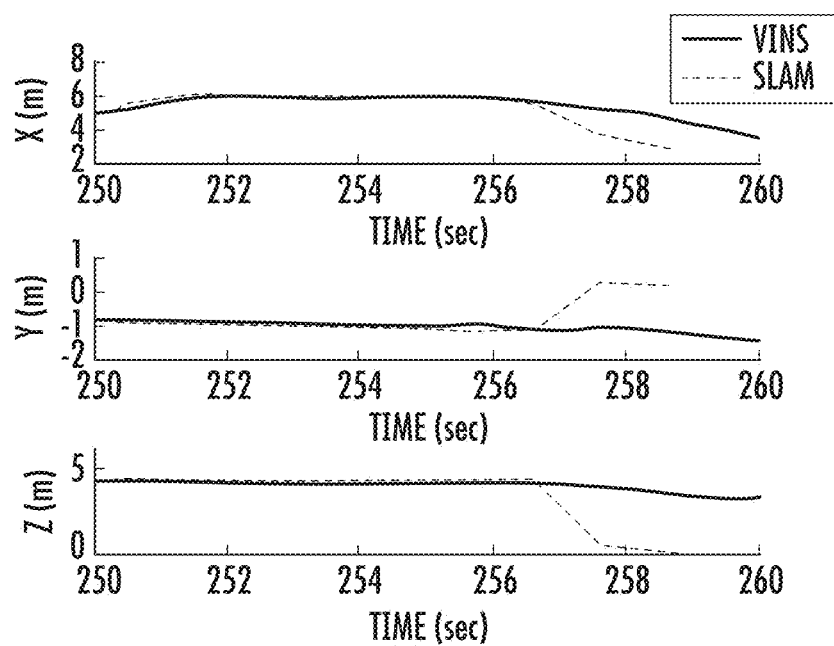
POSITION ESTIMATES DURING LOOP CLOSURE
