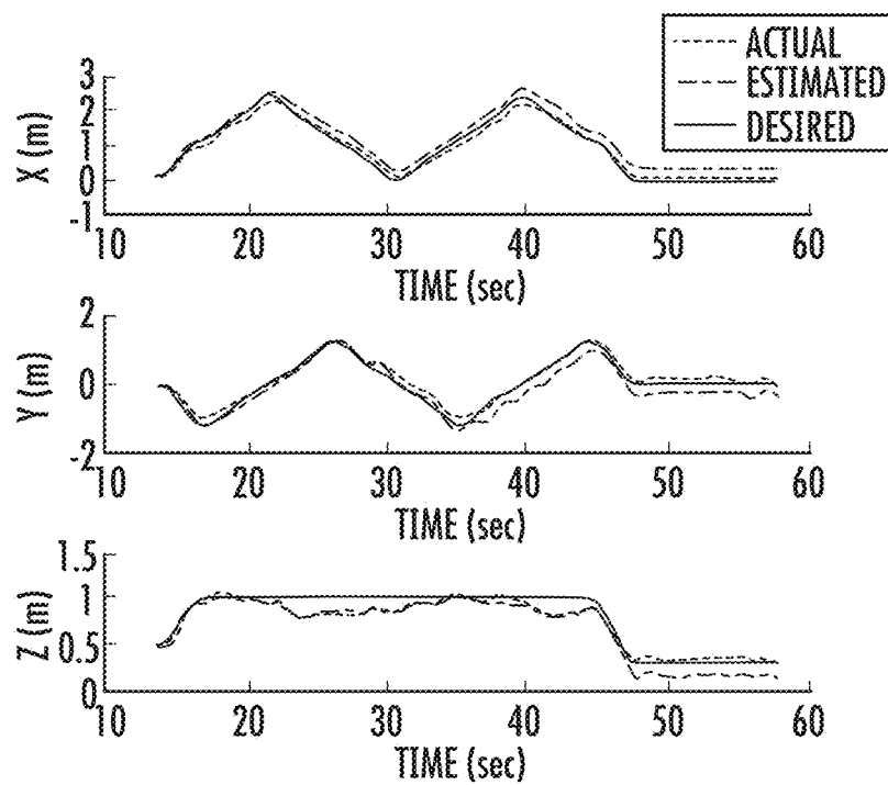
DESIRED, ESTIMATED, AND ACTUAL POSITIONS
