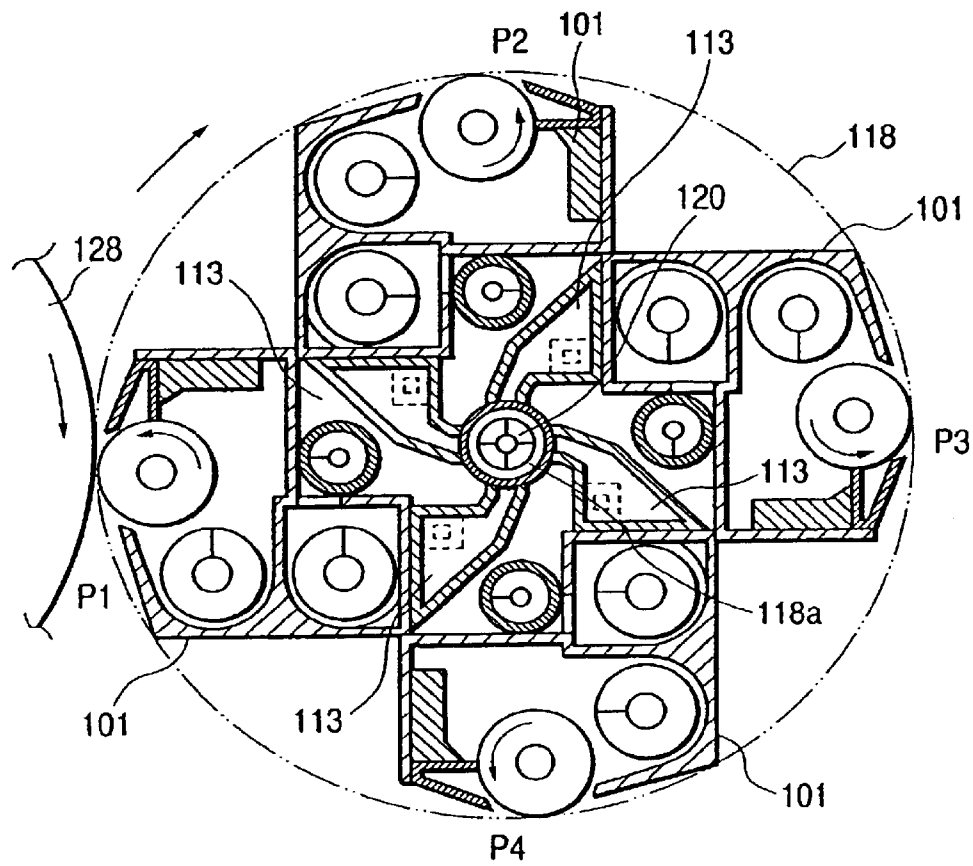
FIG. 12 PRIOR ART
