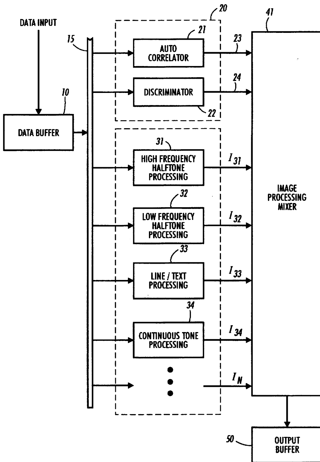
FIG. 15 (Prior Art)
