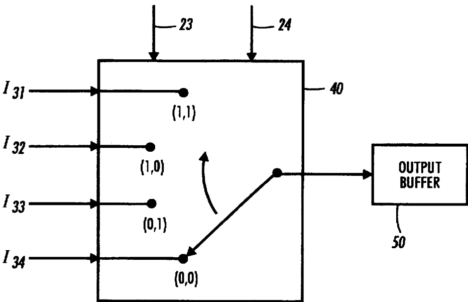
FIG. 17 (Prior Art)
