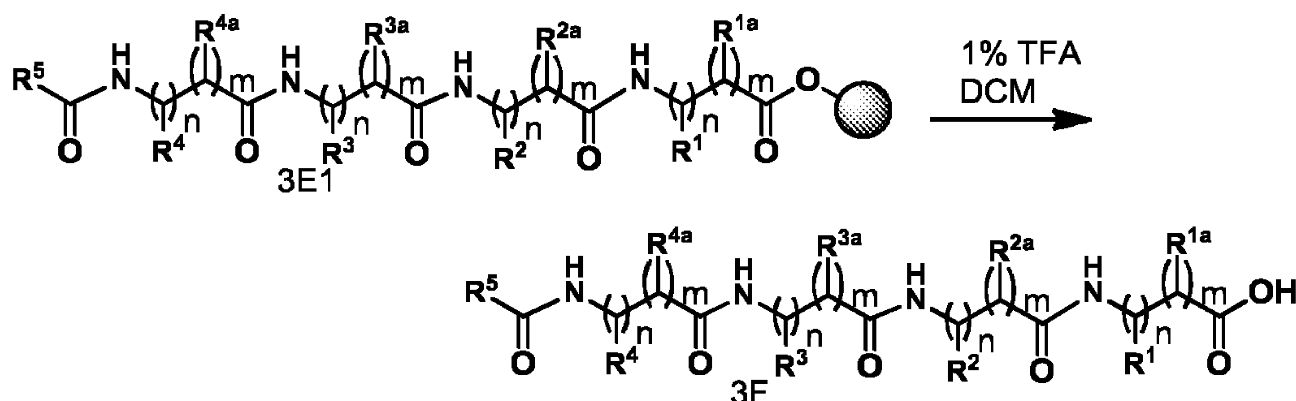
Scheme XVIII
