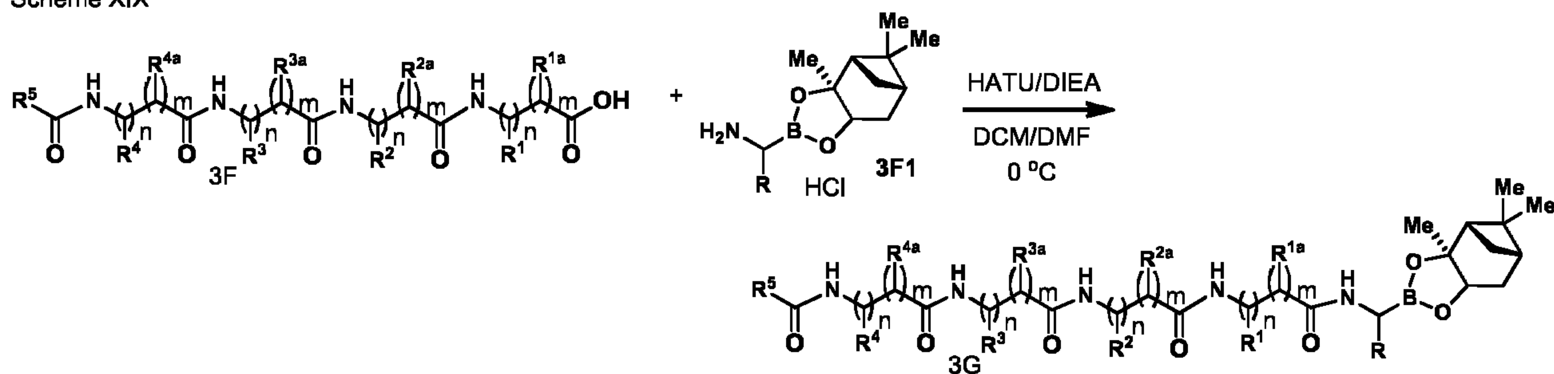
Scheme XIX
