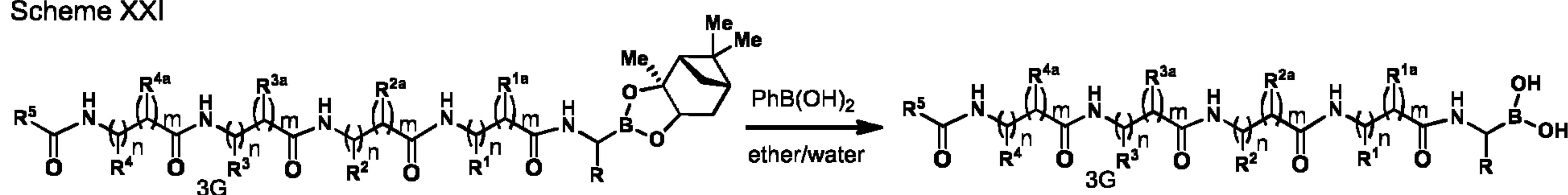
Scheme XXI
