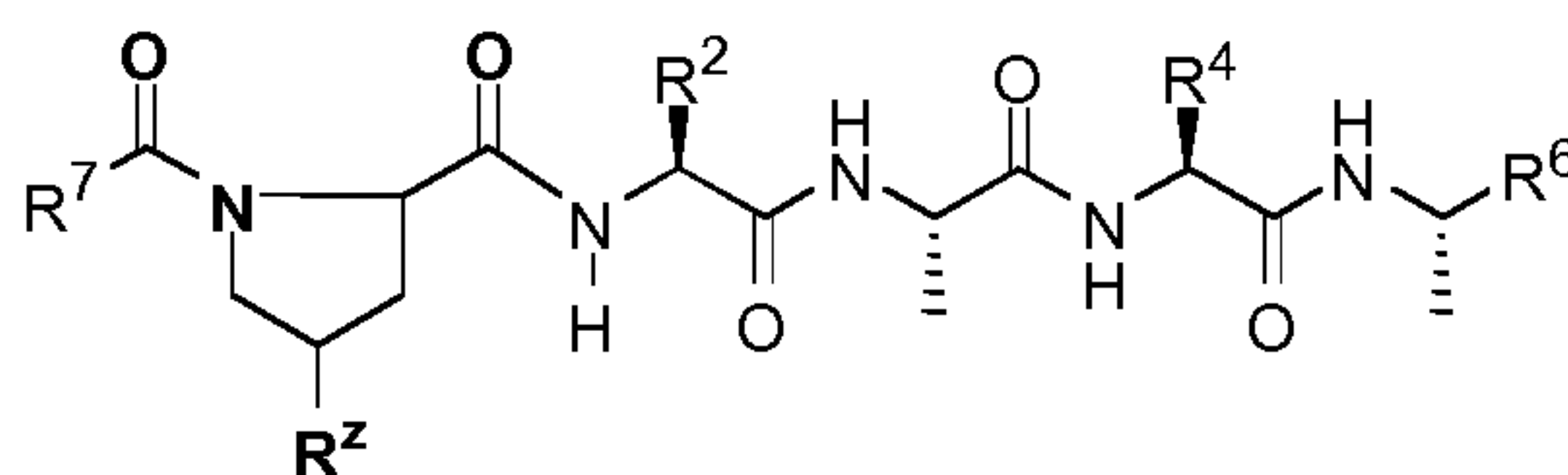
Formula (Id);
