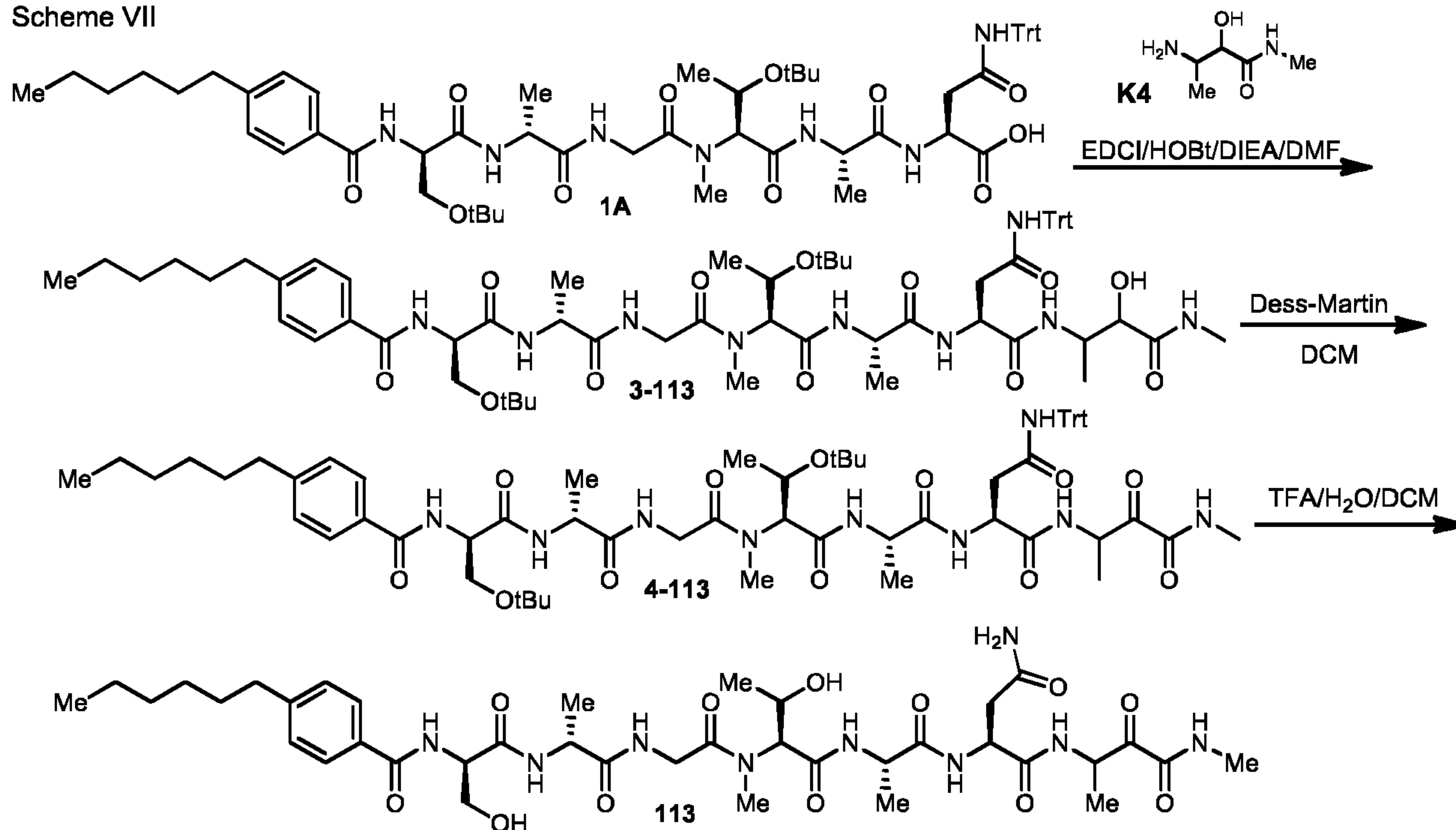
Scheme VII
