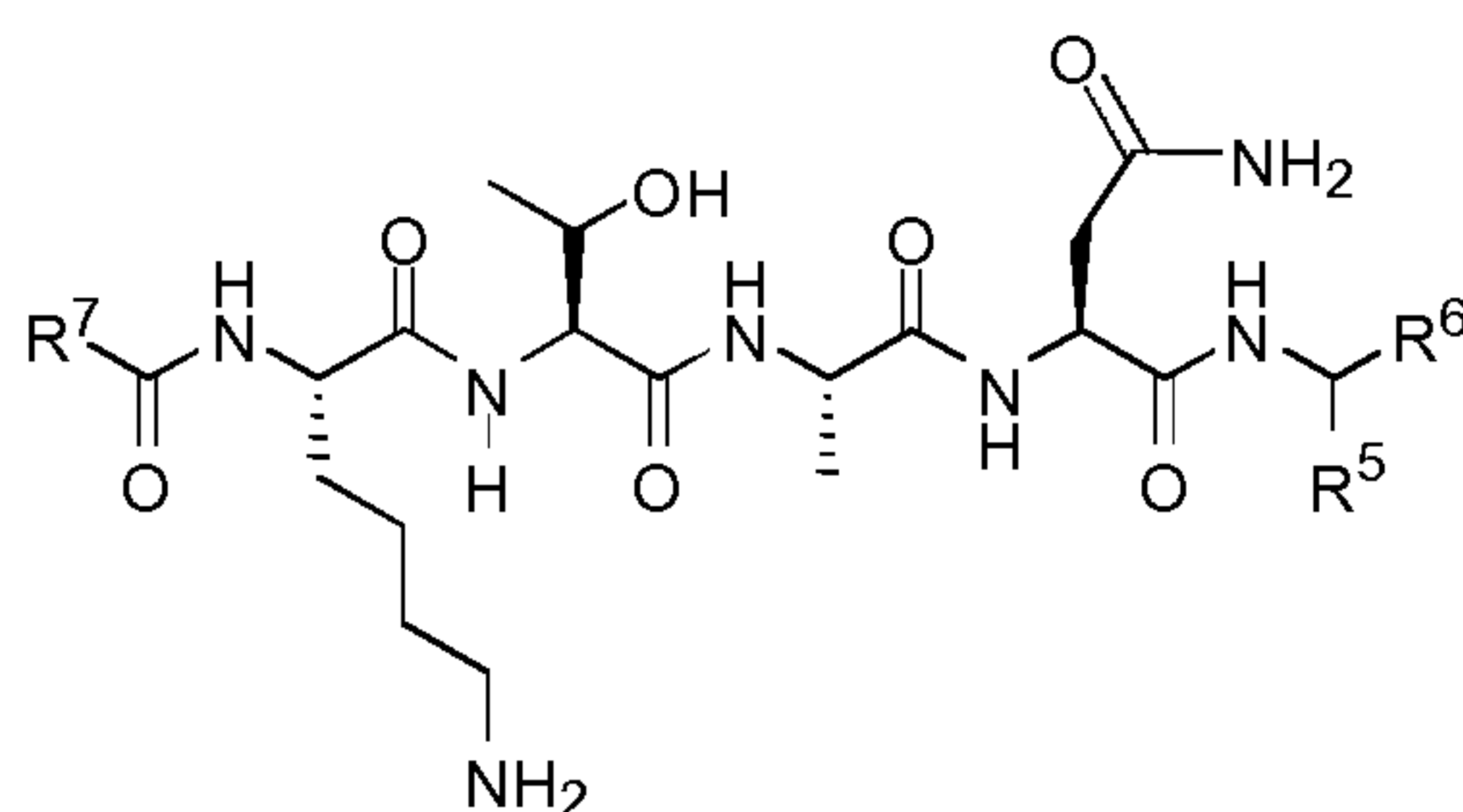
Formula (Icc);
