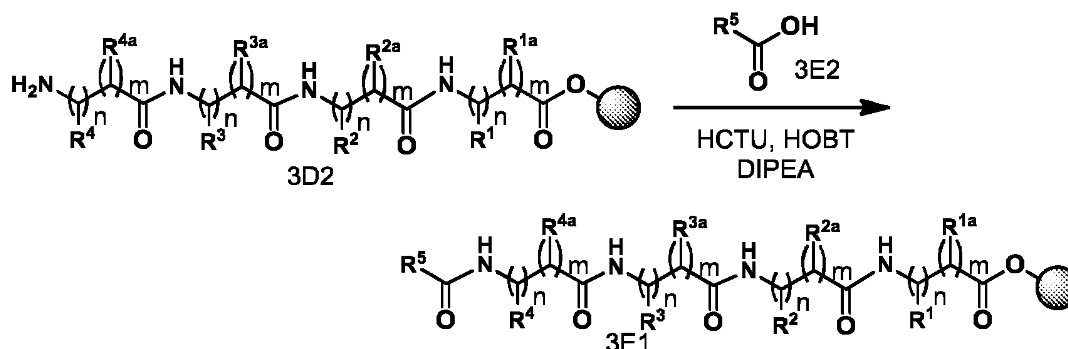
Scheme XVII
