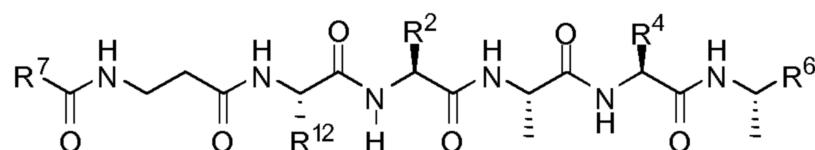
Formula (Ib);
