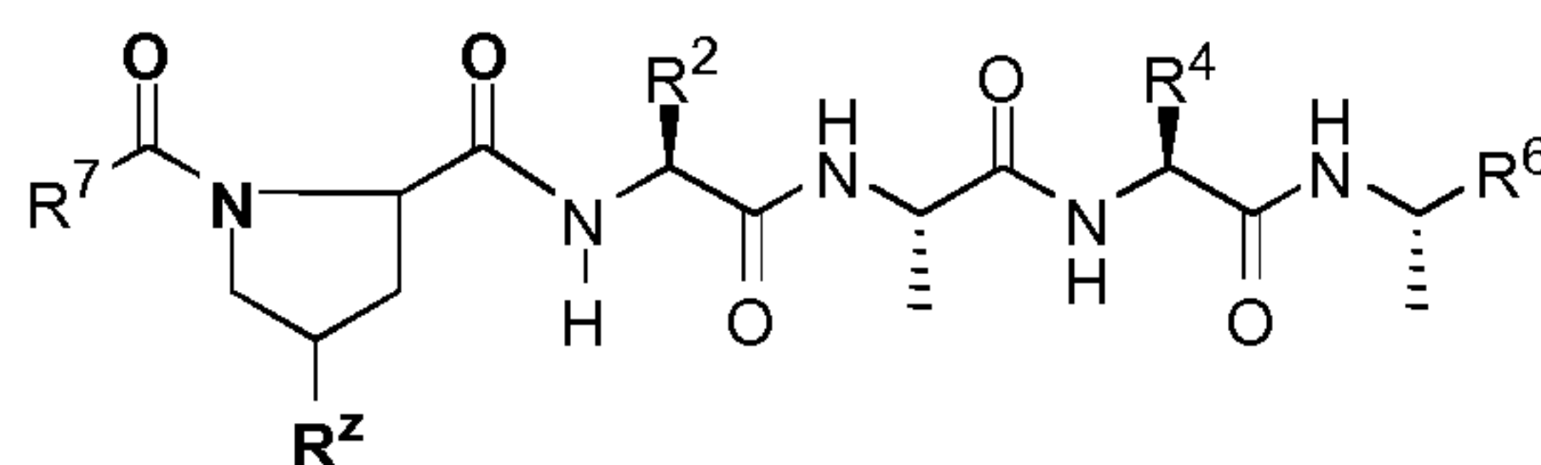
Formula (Id);
