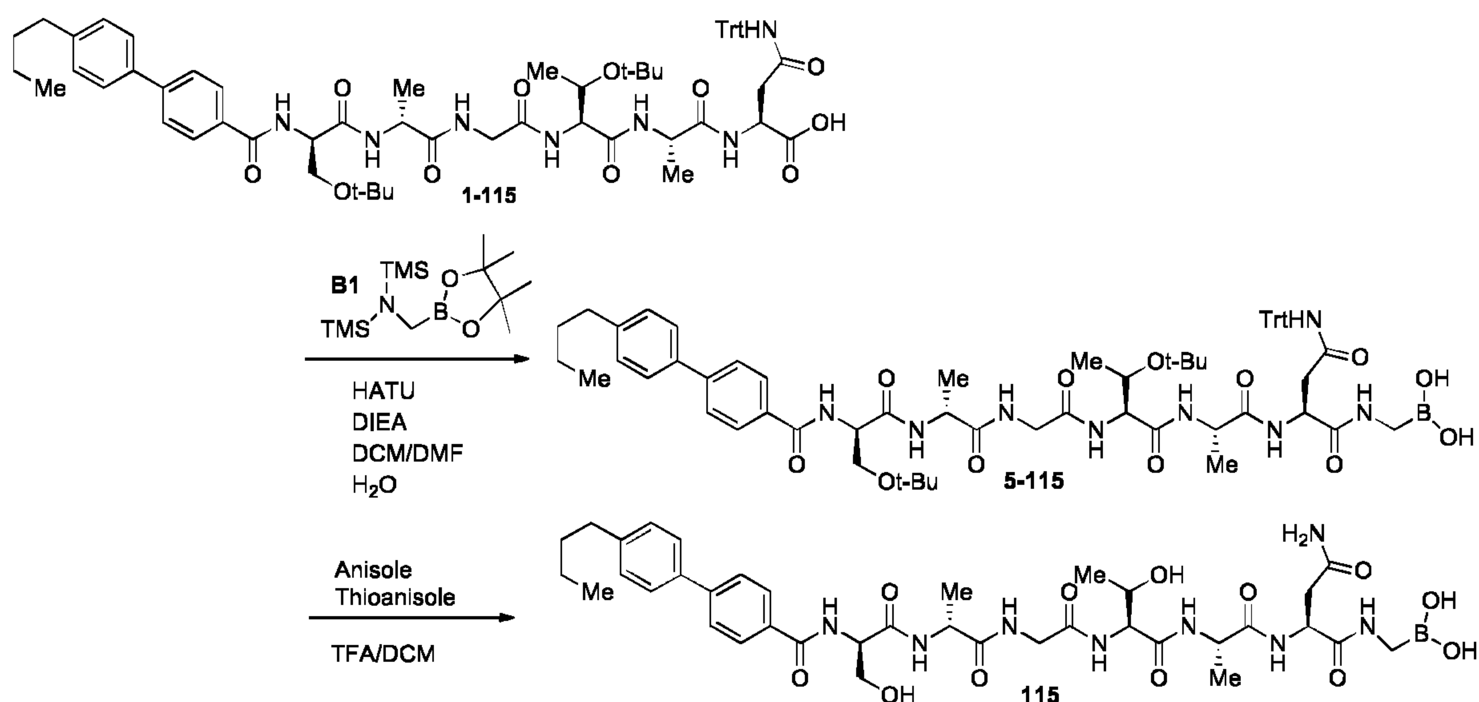
Scheme IX
