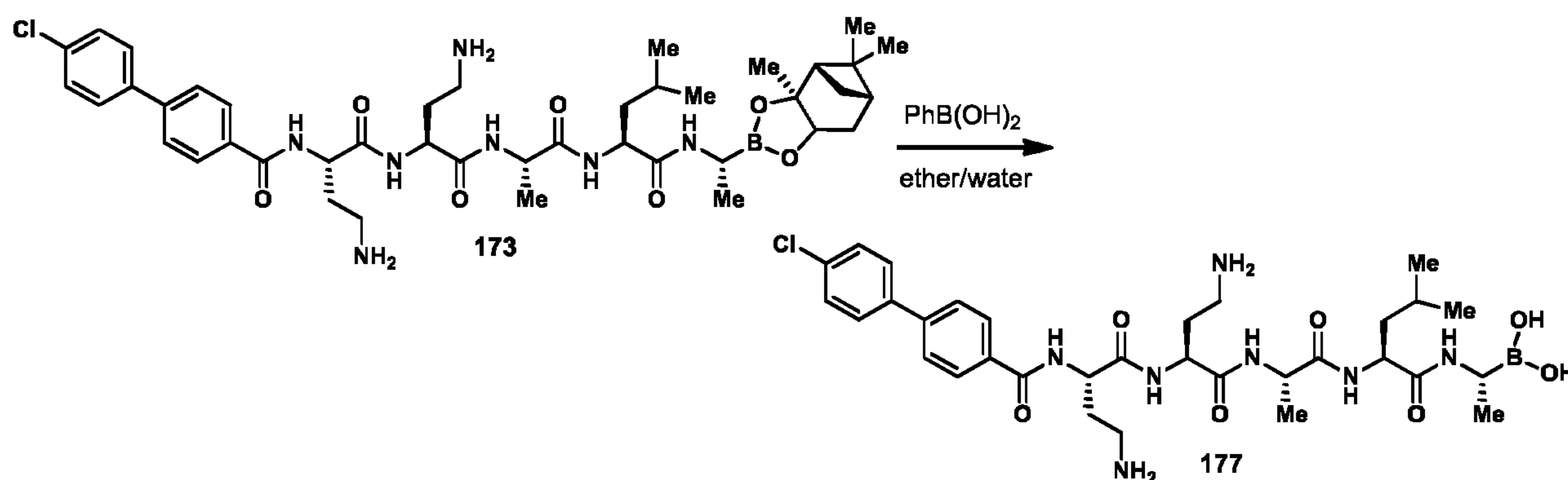
Scheme XXII
