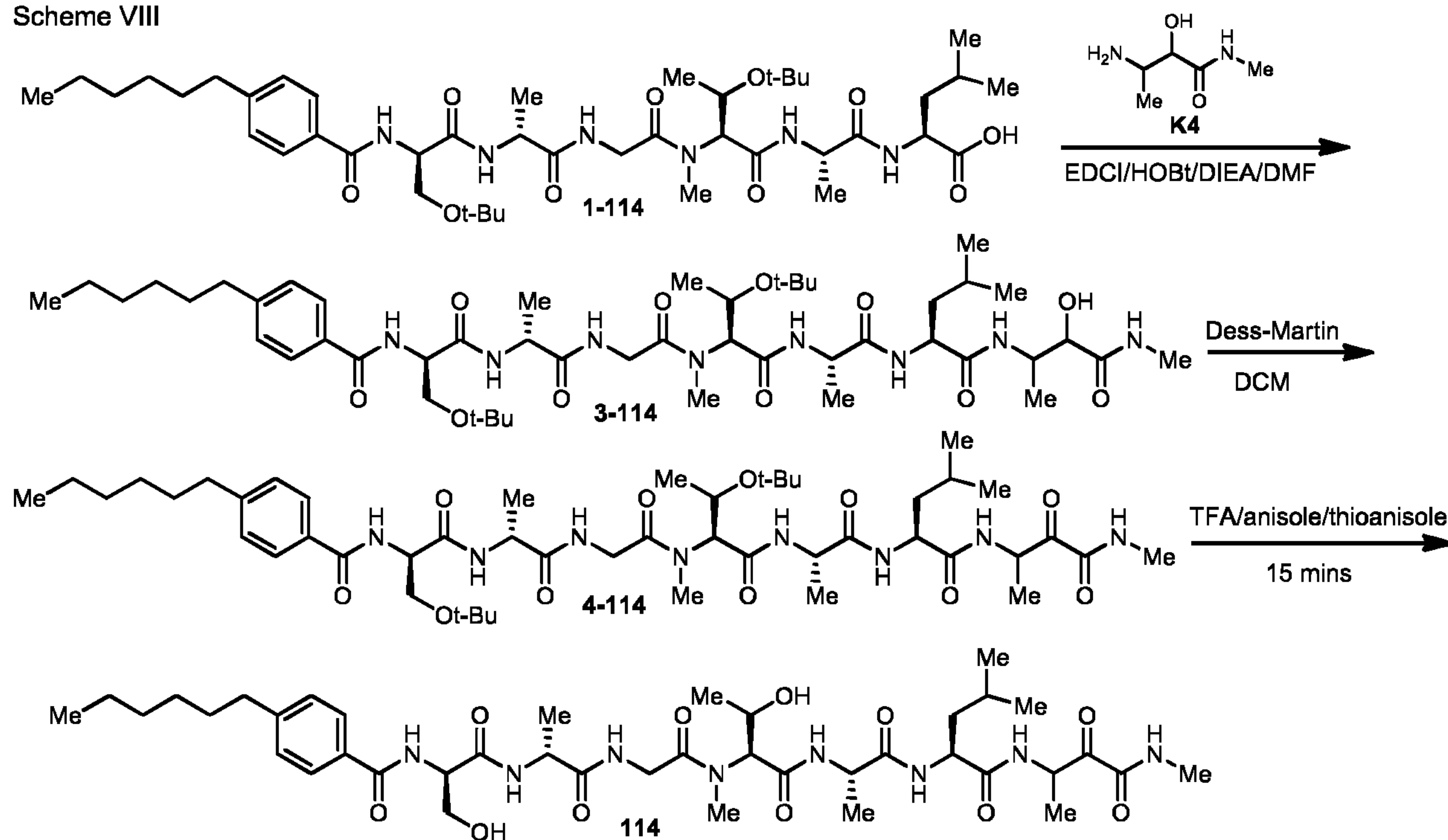
Scheme VIII
