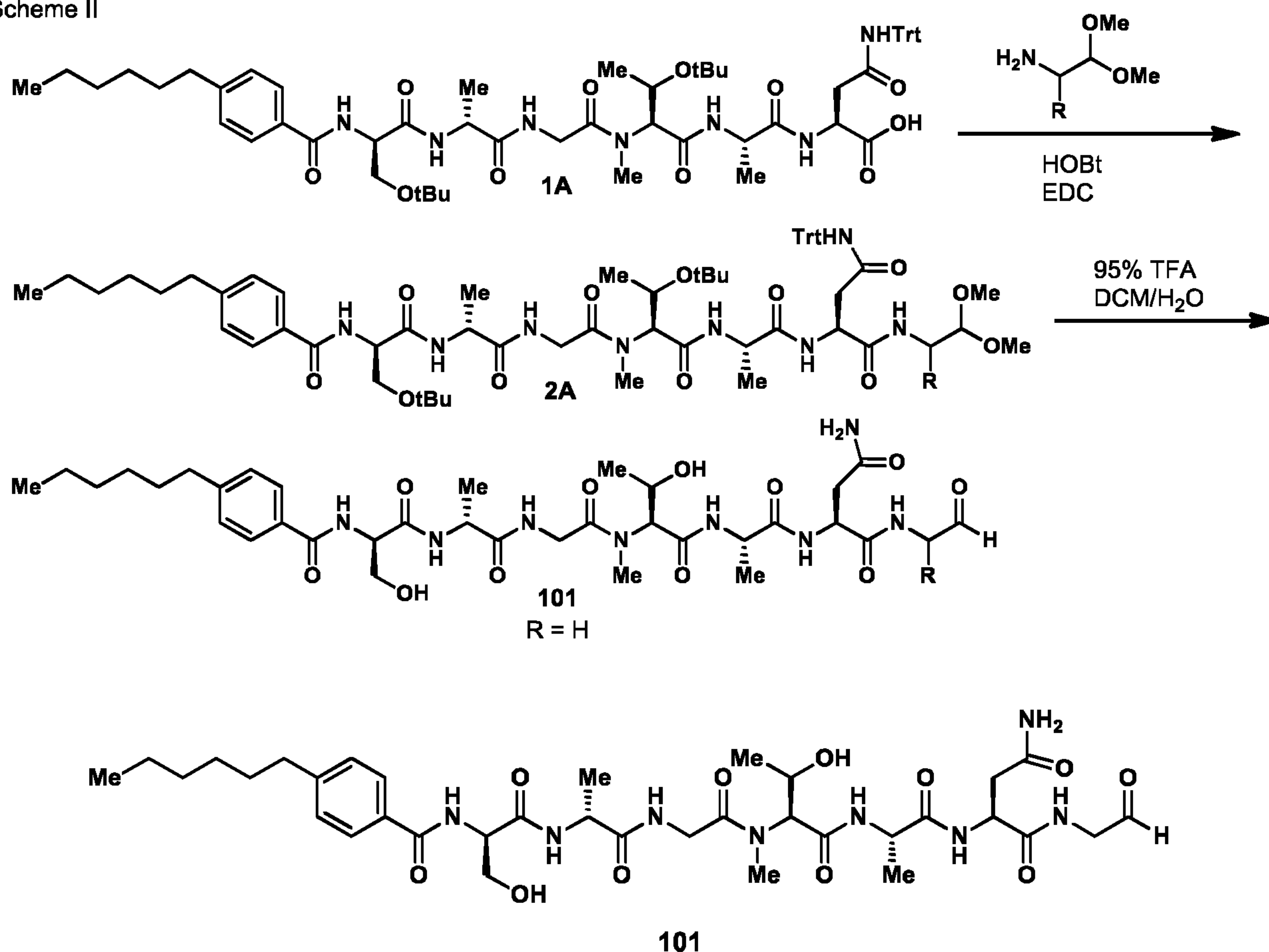
Scheme II
