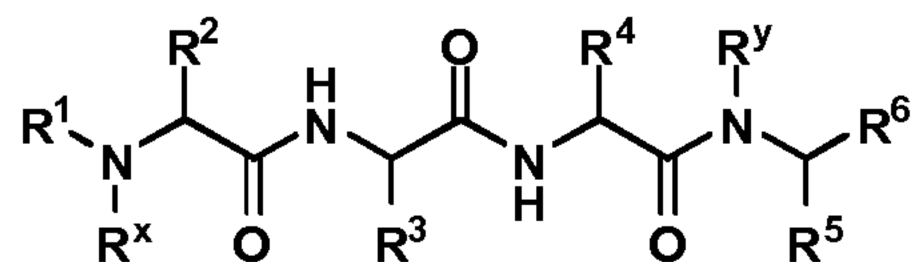
Formula (I)
