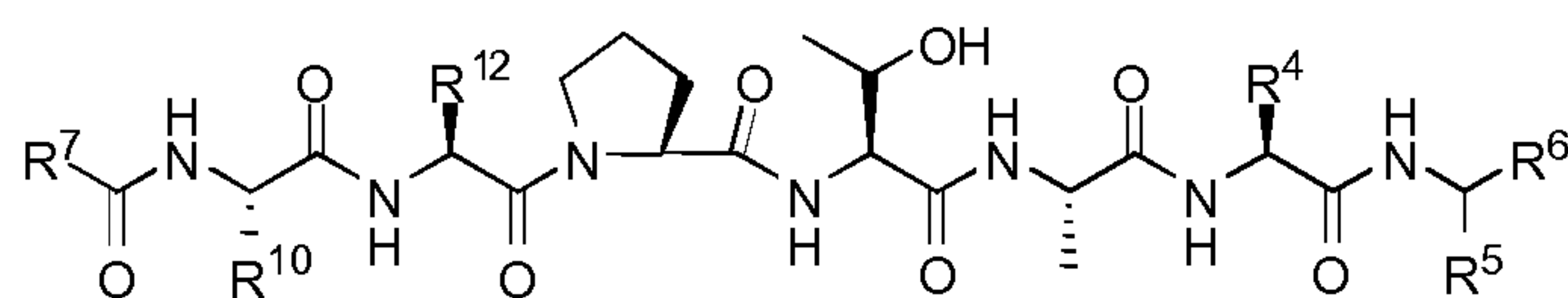
Formula (Idd);
