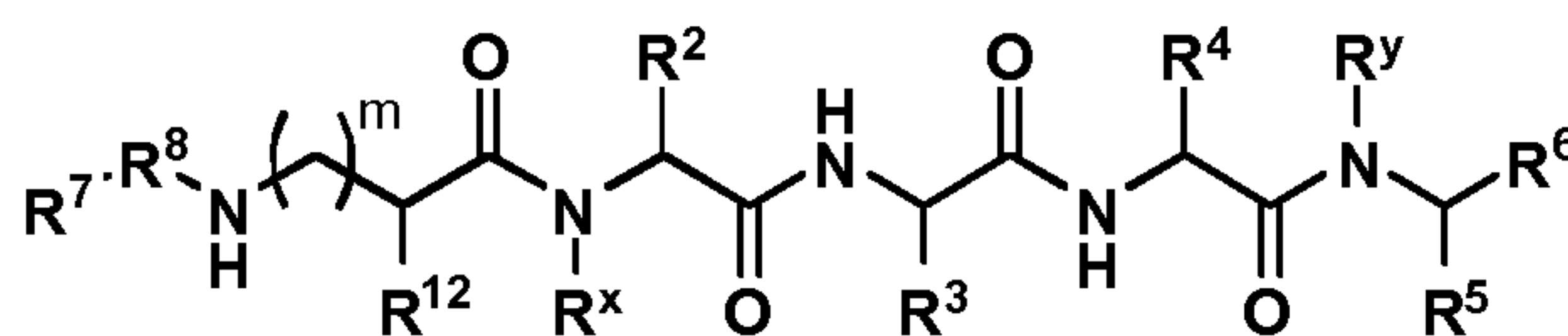
Formula (II)
