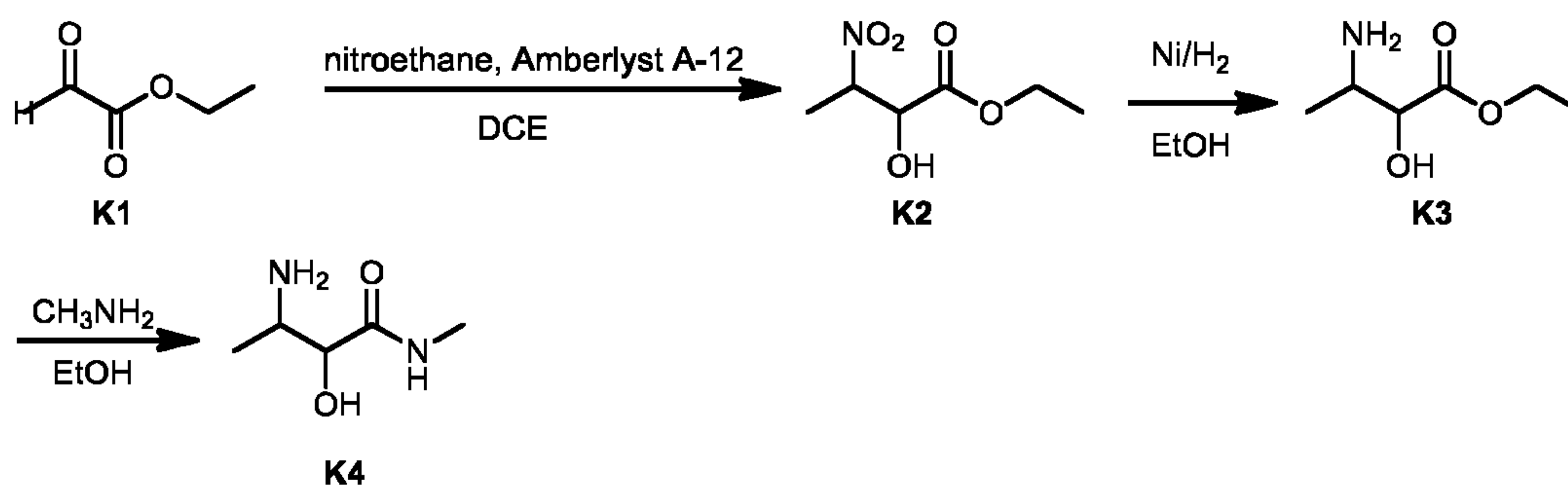
Scheme IV
