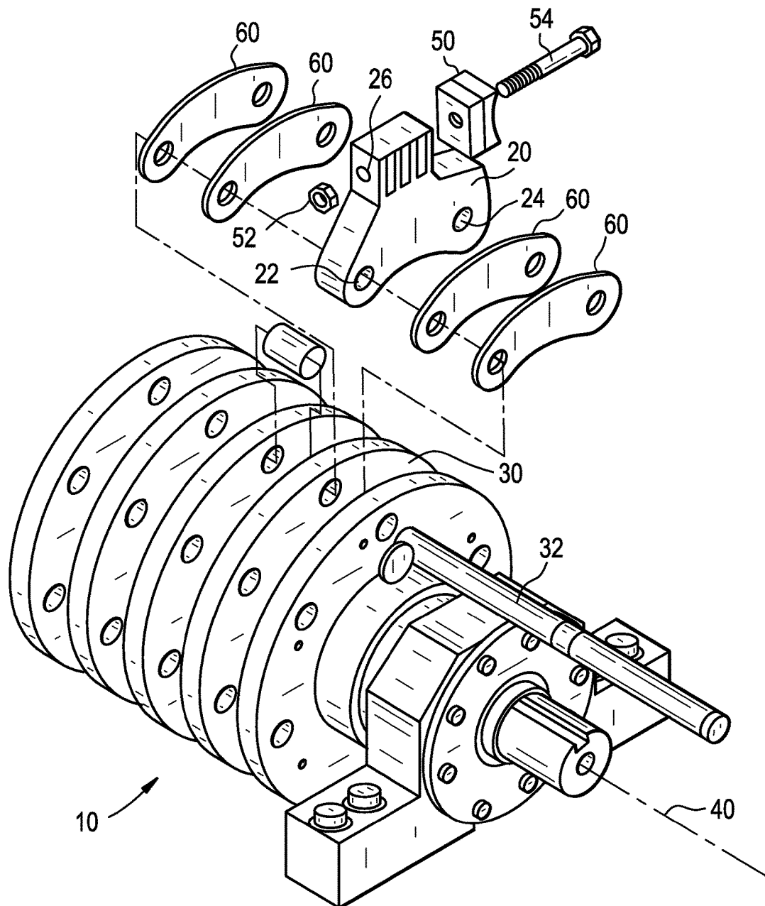
FIG. 2 PRIOR ART
