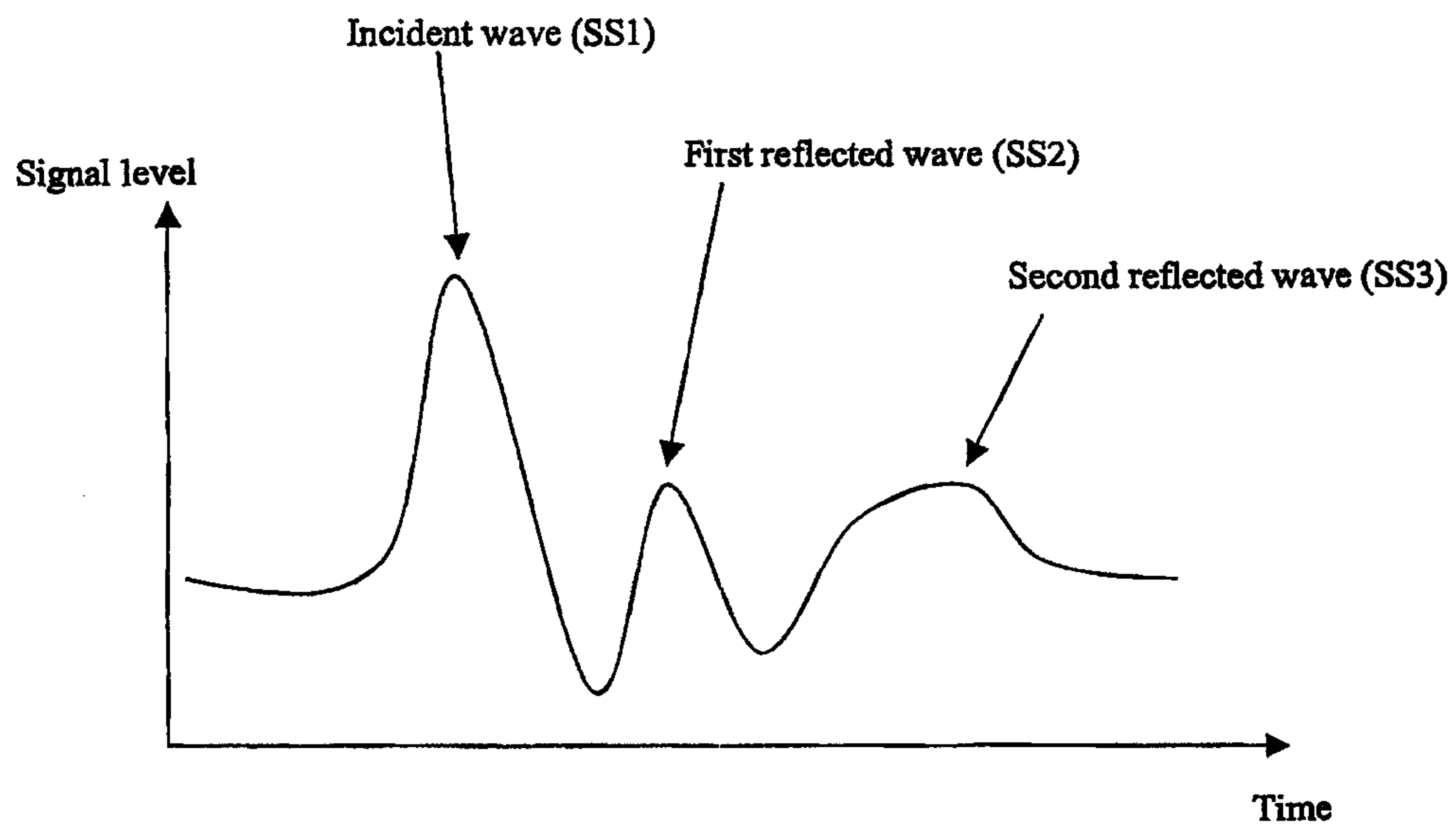
Figure 2: Idealised Suprasystolic Signal
