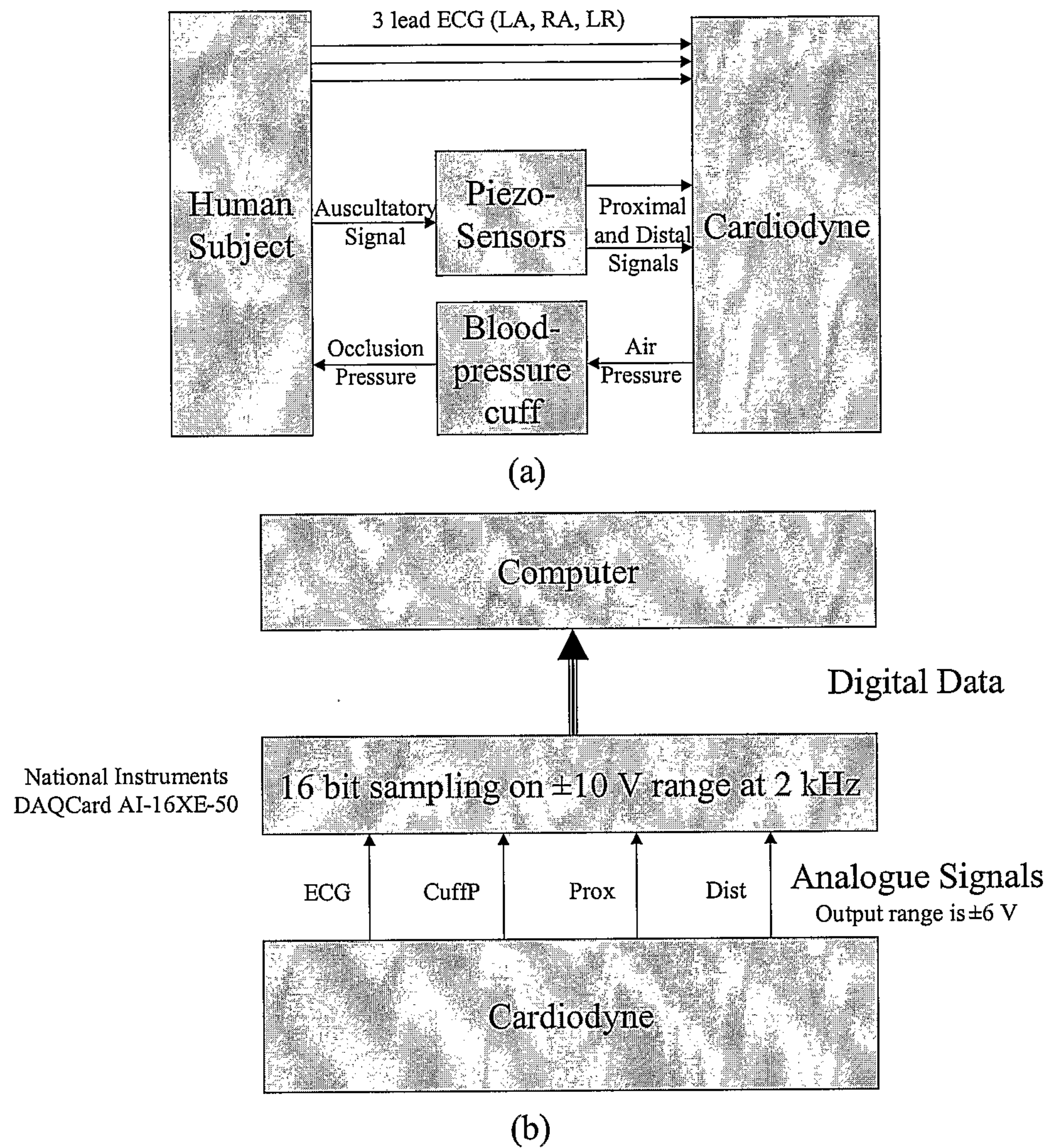
Figure 9: Measurement device interface with subject (a) and computer (b)
