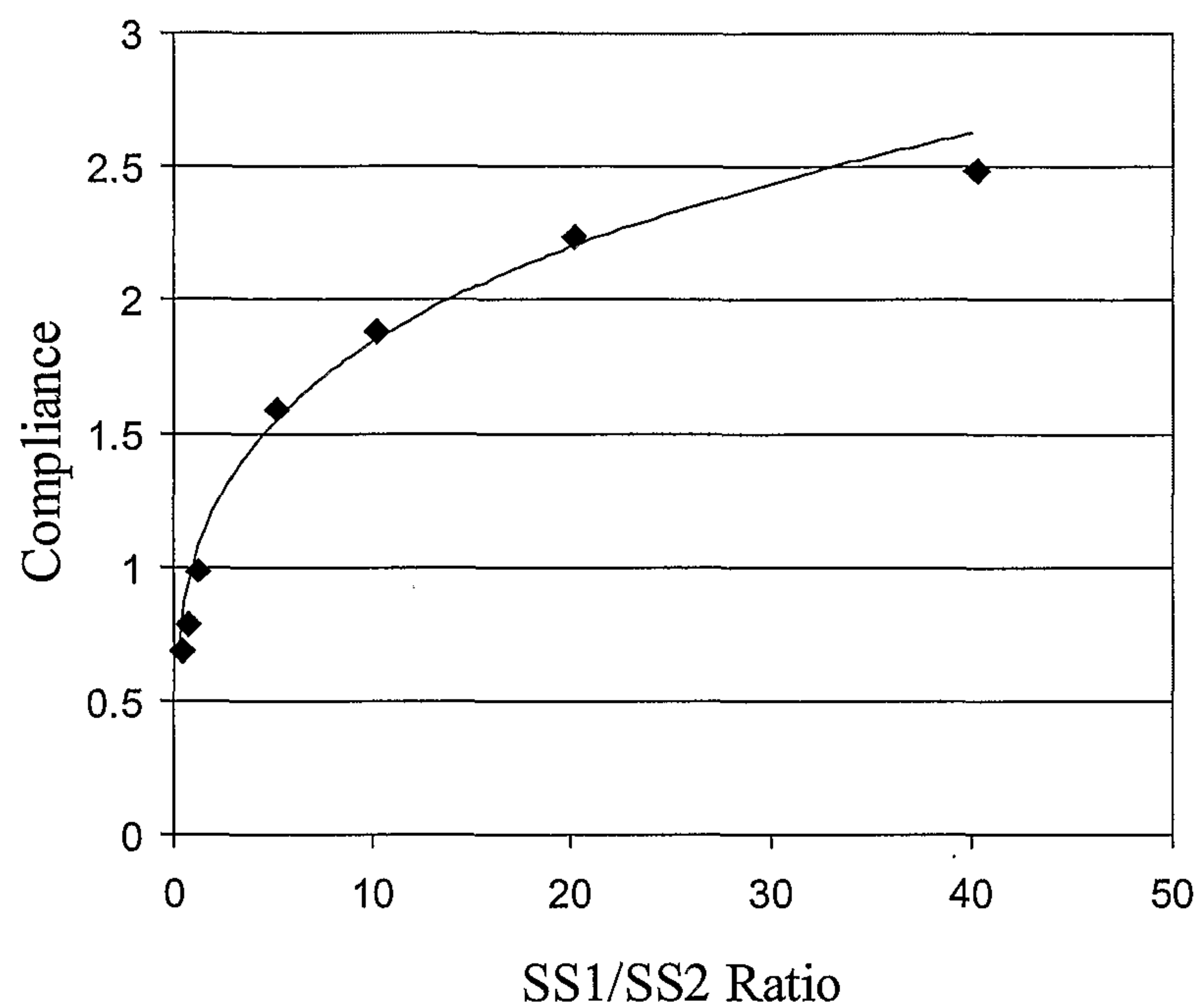
Figure 19: Relationship between SS1/SS2 and compliance.
