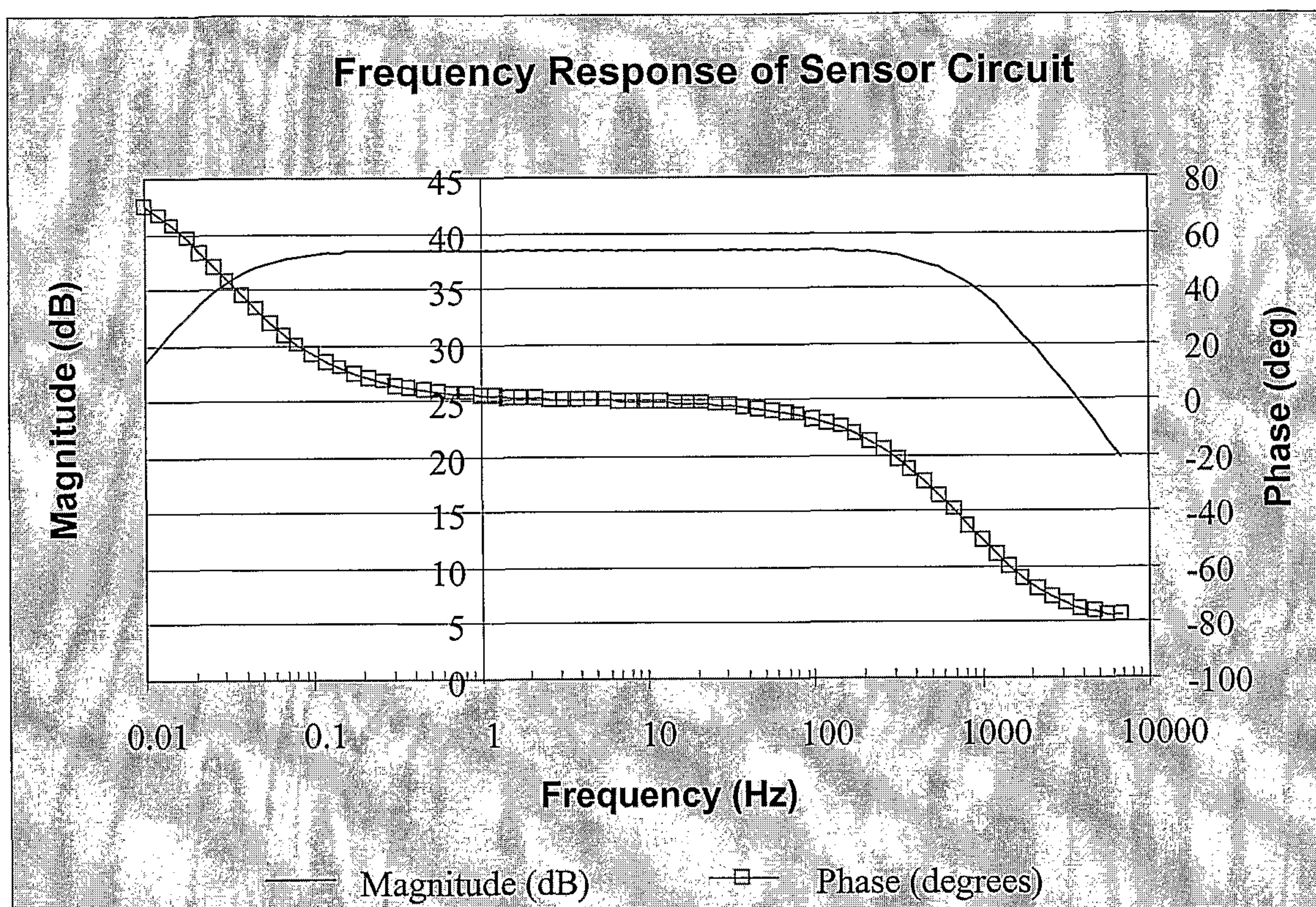
Figure 6: Frequency response of sensor
