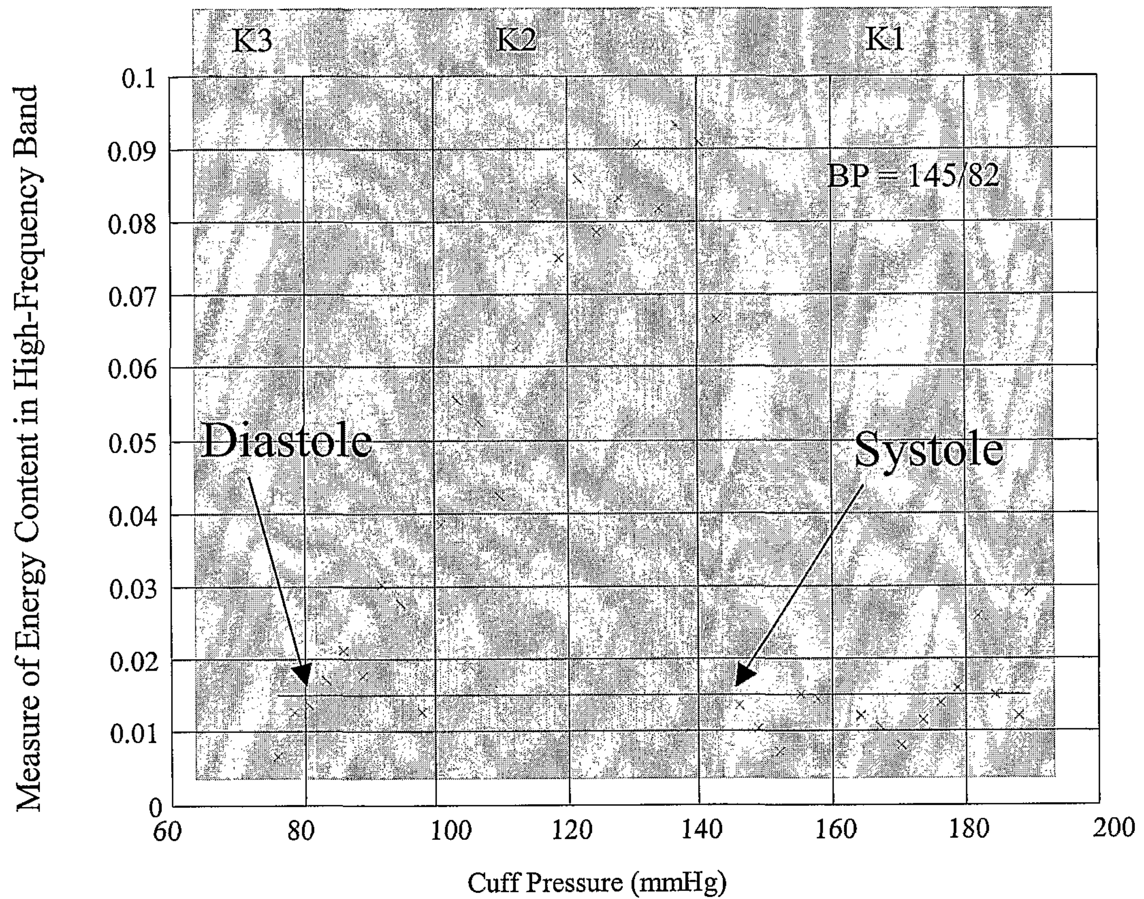
Figure 8: High frequency content of recorded beats
