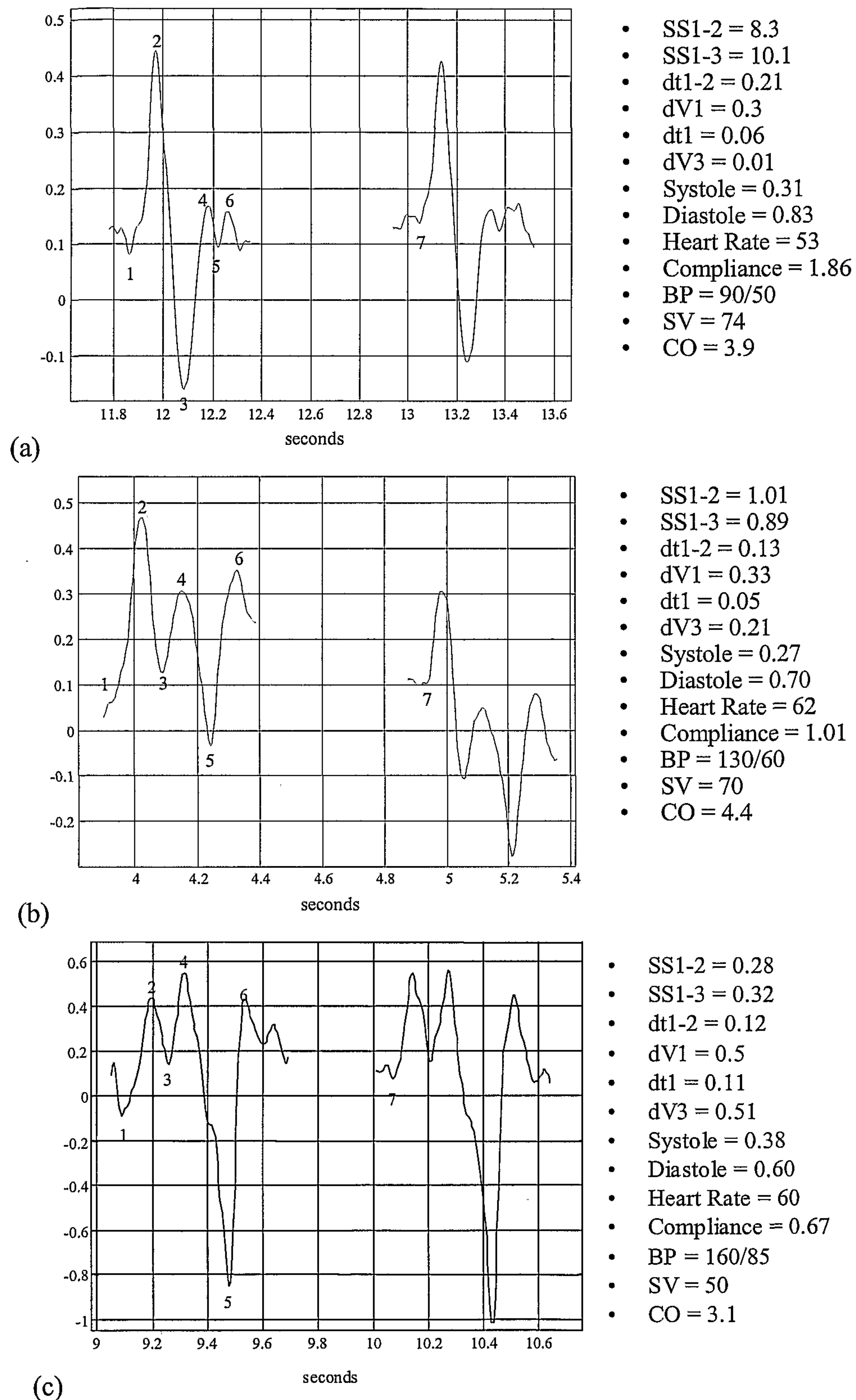
Figure 10: Representative suprasystolic waveforms for (a) young person, (b) moderately reduced compliance, (c) elderly person with hypertension. Vertical axis in all cases is in Volts.
