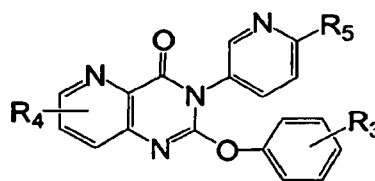
Formula IX
