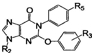
Formula IIa
