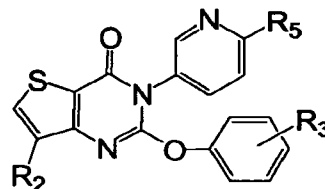
Formula VIIa
