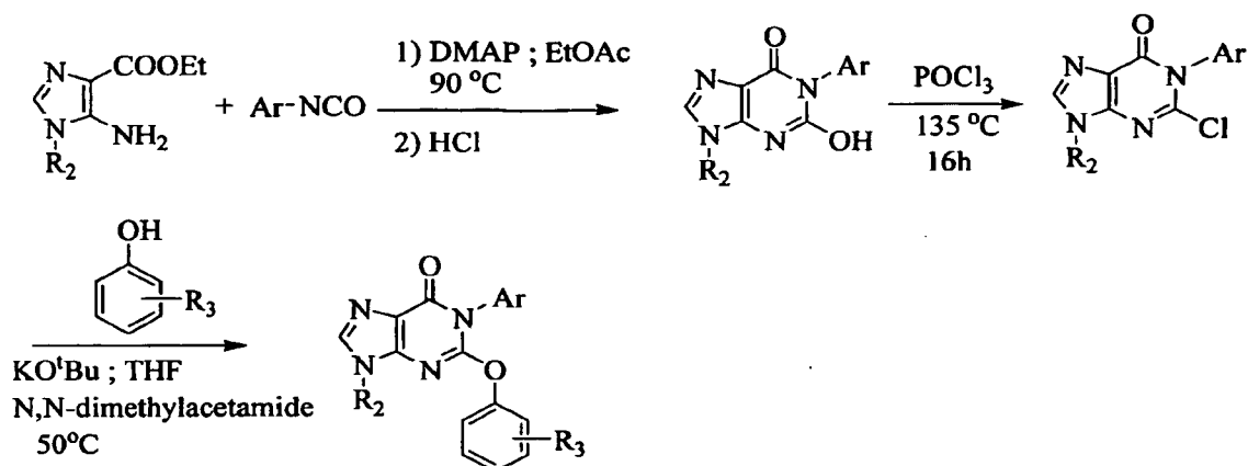
Scheme 5
