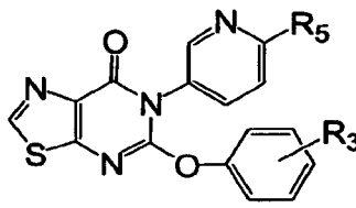
Formula VIa
