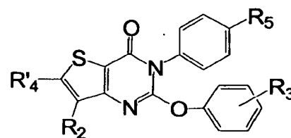
Formula IV
