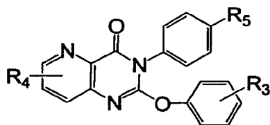
Formula VIII
