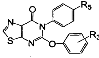
Formula IIIa
