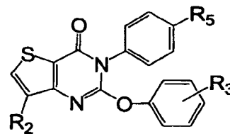
Formula IVa
