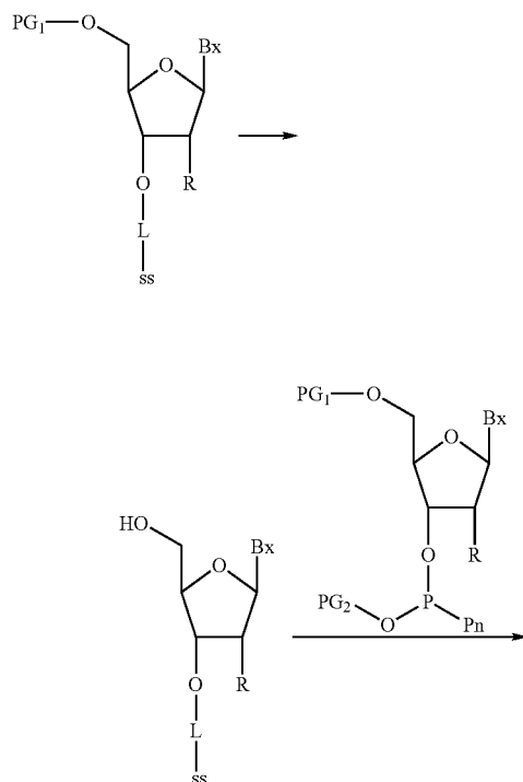
Scheme 1: Solid phase Synthesis of Oligonucleotides
