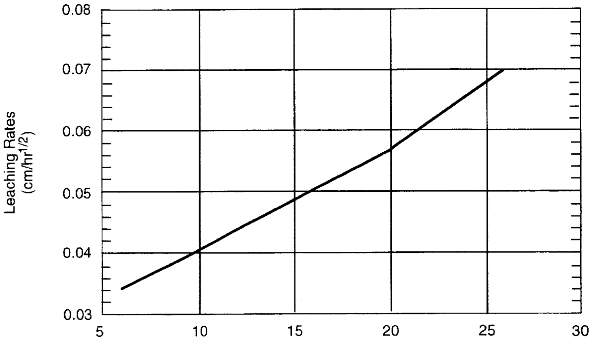
Leaching Rates of Silica Doped Alumina Cores (250 c/1800 psi/1 hr)
