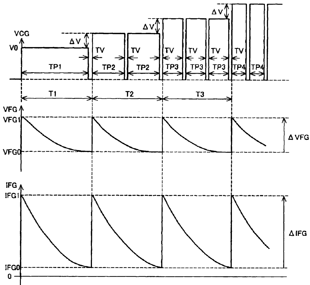
FIG. 3 WAVEFORM DIAGRAM DIRECTED TO FIRST EMBODIMENT
