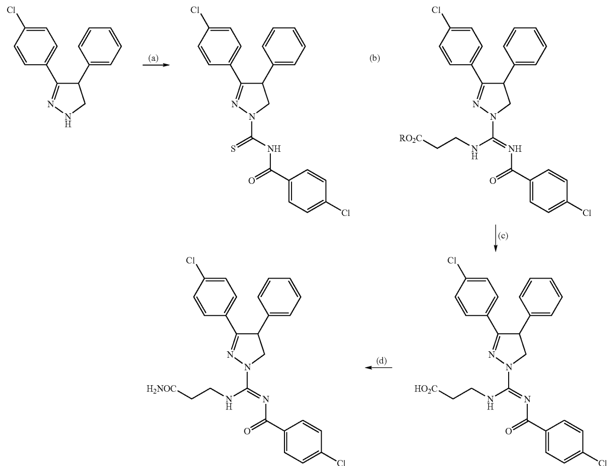
Scheme 6
