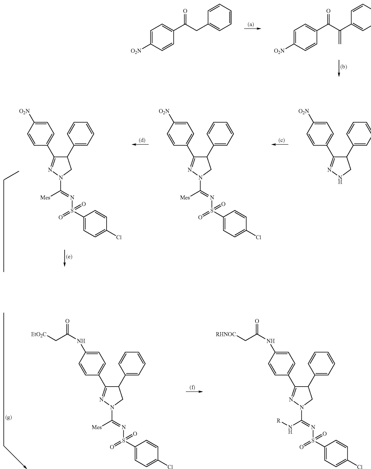
Scheme 7
