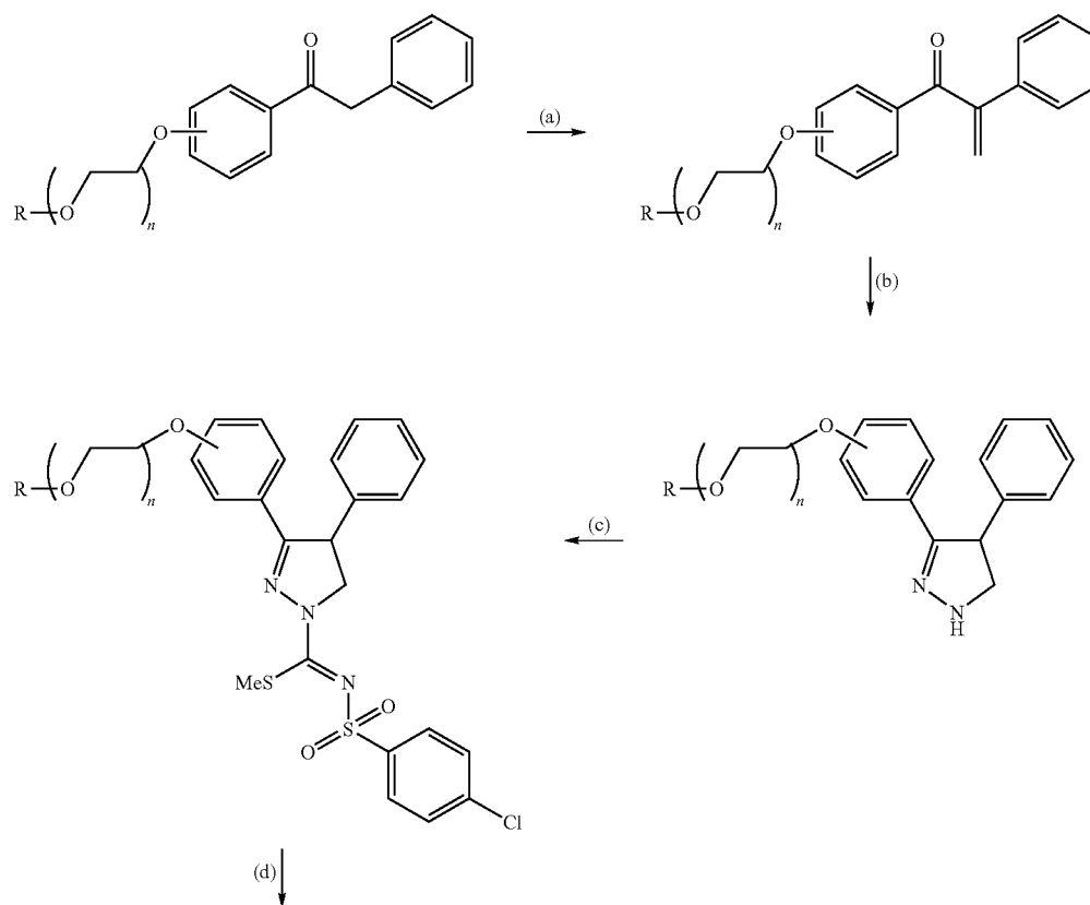
Scheme 9
