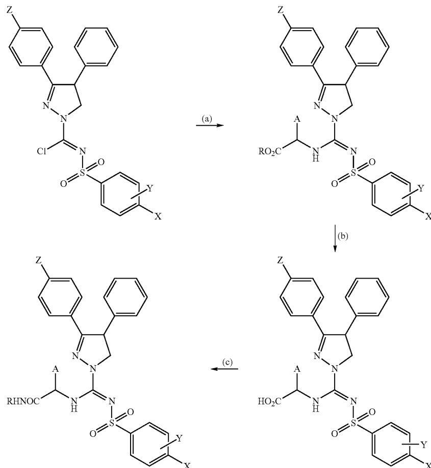
SCHEME 3a
