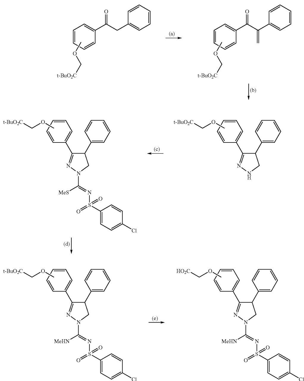
Scheme 1
