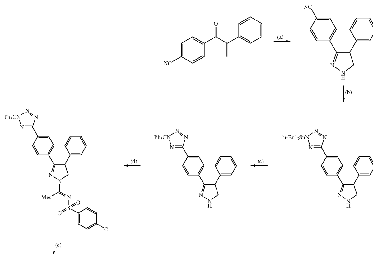
Scheme 8
