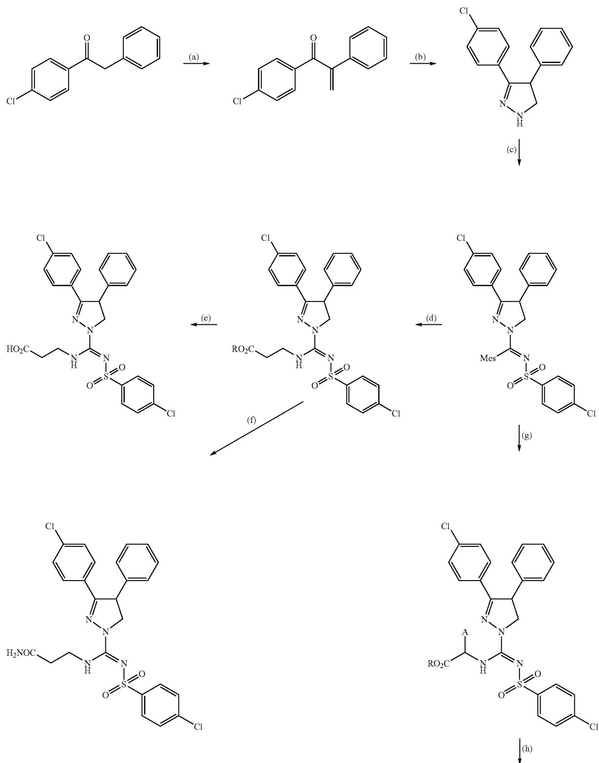
Scheme 3
