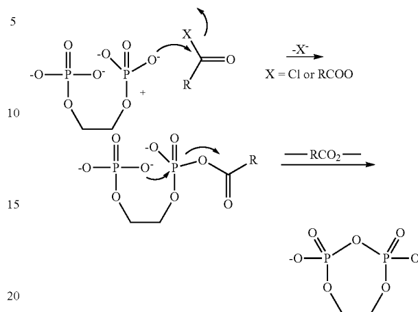
Scheme 2. Mechanism of internal pyrophosphate formation
