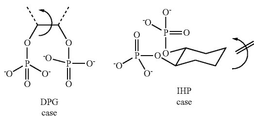
Scheme 5. Explantation of the behaviour of DPG and IHP toward acyl anhydrides.
