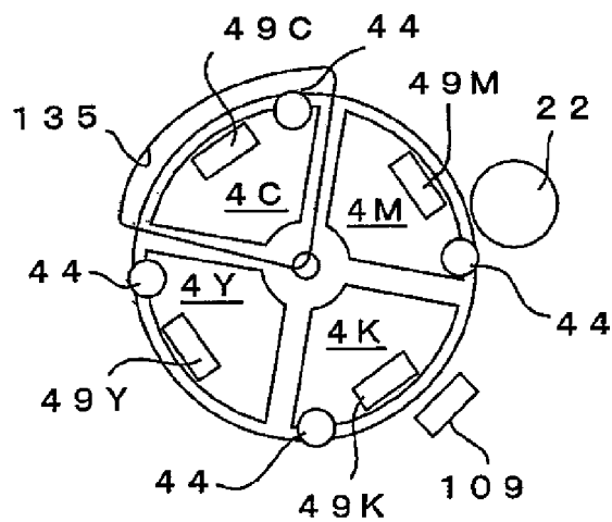
FIG. 5C : MOUNTING/DISMOUNTING POSITION
