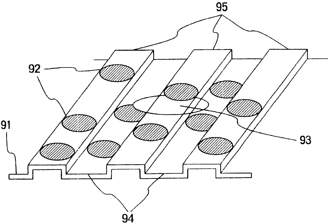
FIG. 13 PRIOR ART
