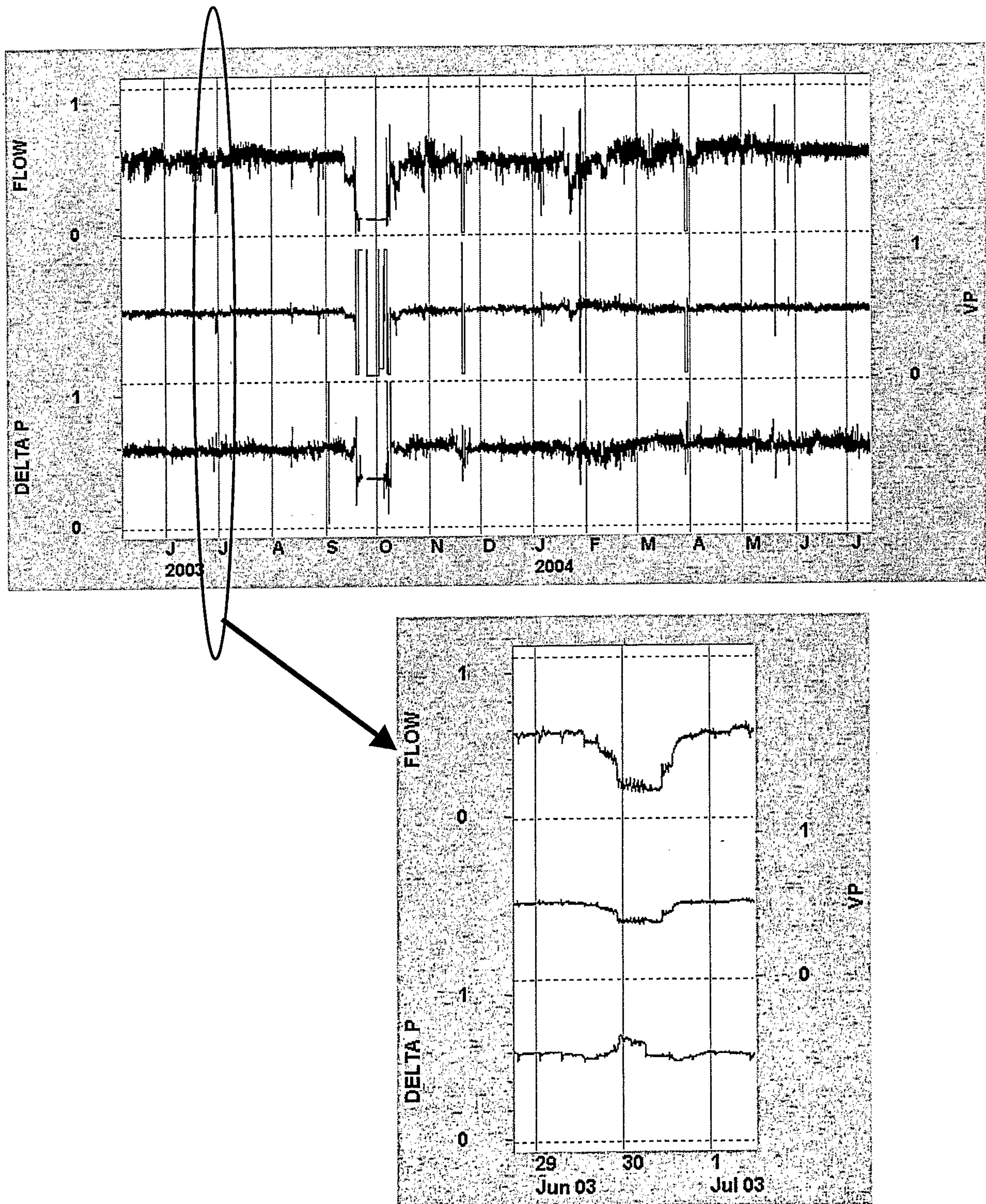
Figure 15 Valve to Flow Data
