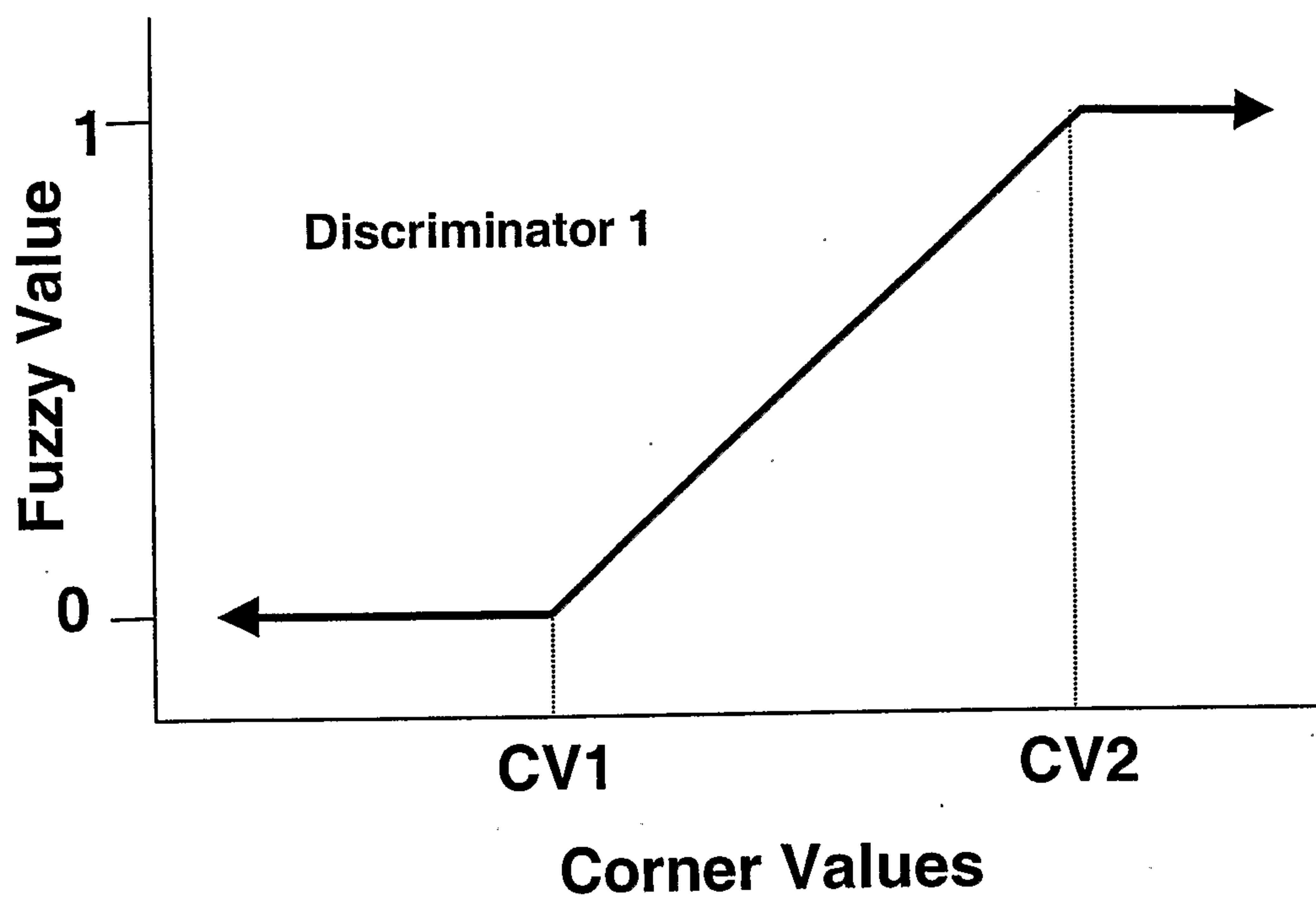
Figure 16 Fuzzy Discriminators
