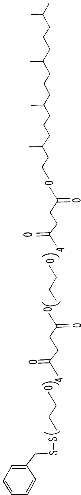
LINKER LIPID A
