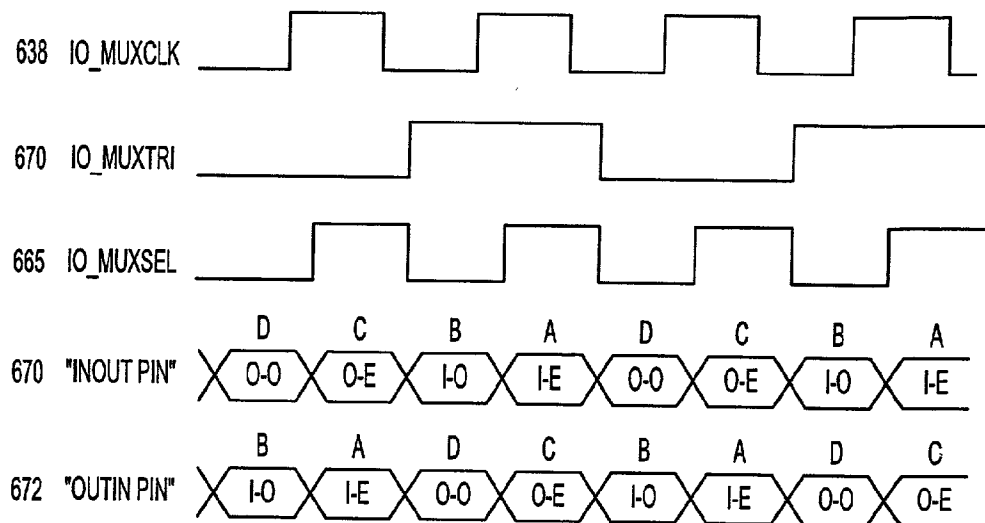
TIMING FOR 4-WAY TIME MULTIPLEXING (BI-DIRECTIONAL)
