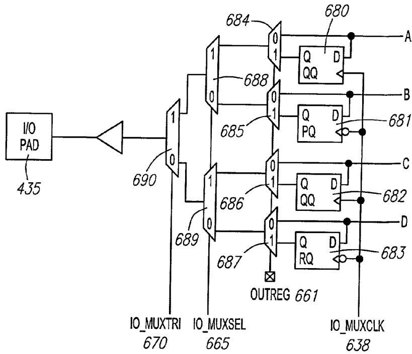
LOGIC FOR 4-WAY TIME MULTIPLEXING (UNI-DIRECTIONAL OUTPUT)
