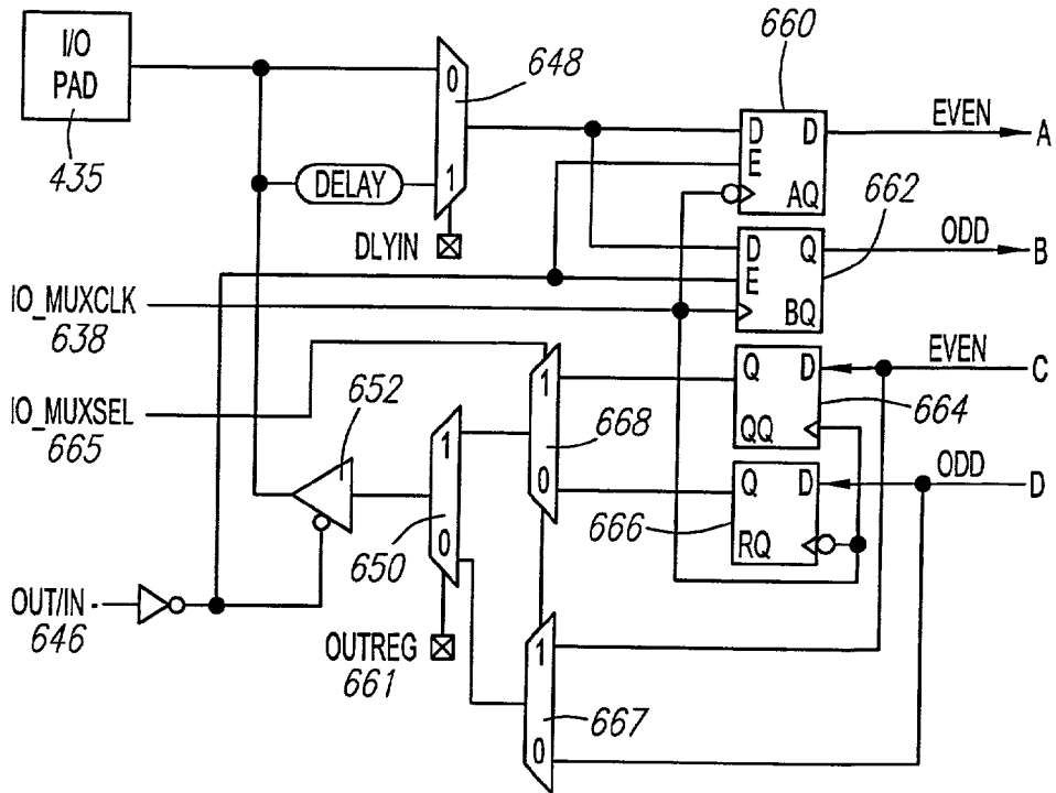
LOGIC FOR 2-WAY TIME MULTIPLEXING
