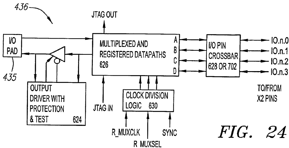
I/O BLOCK MAJOR COMPONENTS
