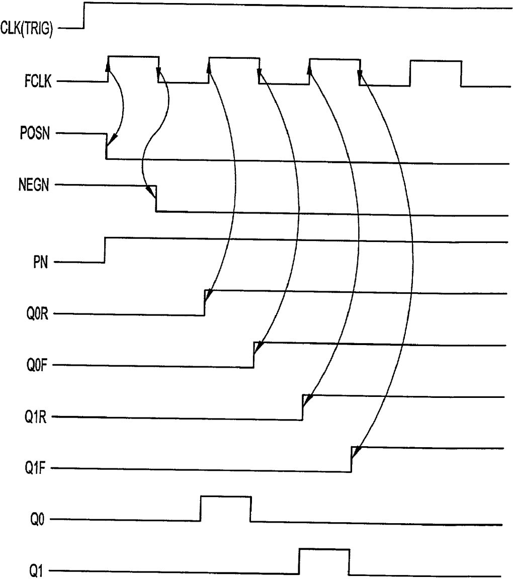
LEPULSE TIMING
