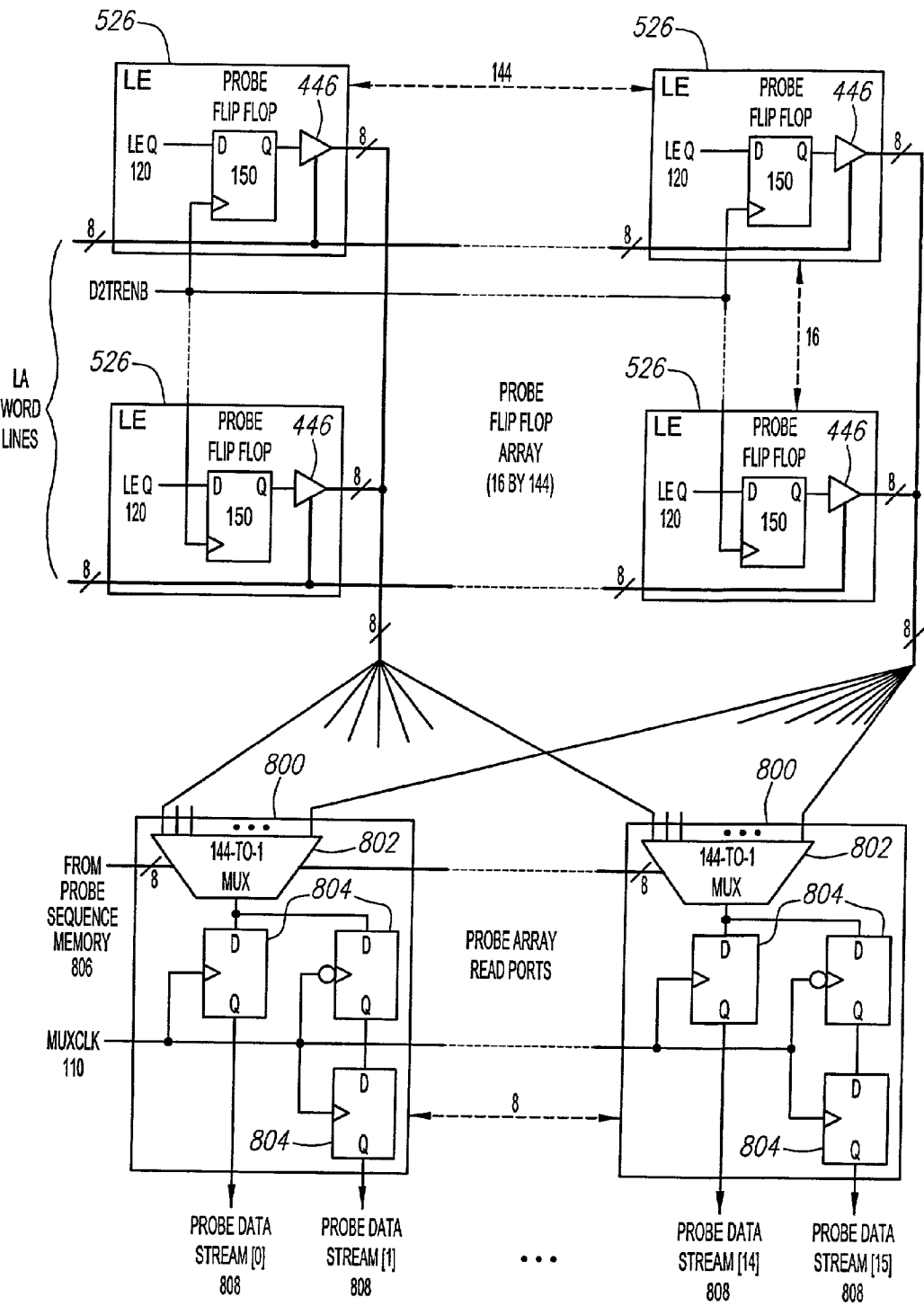
PROBE FLIP FLOP ARRAY AND READ PORTS
