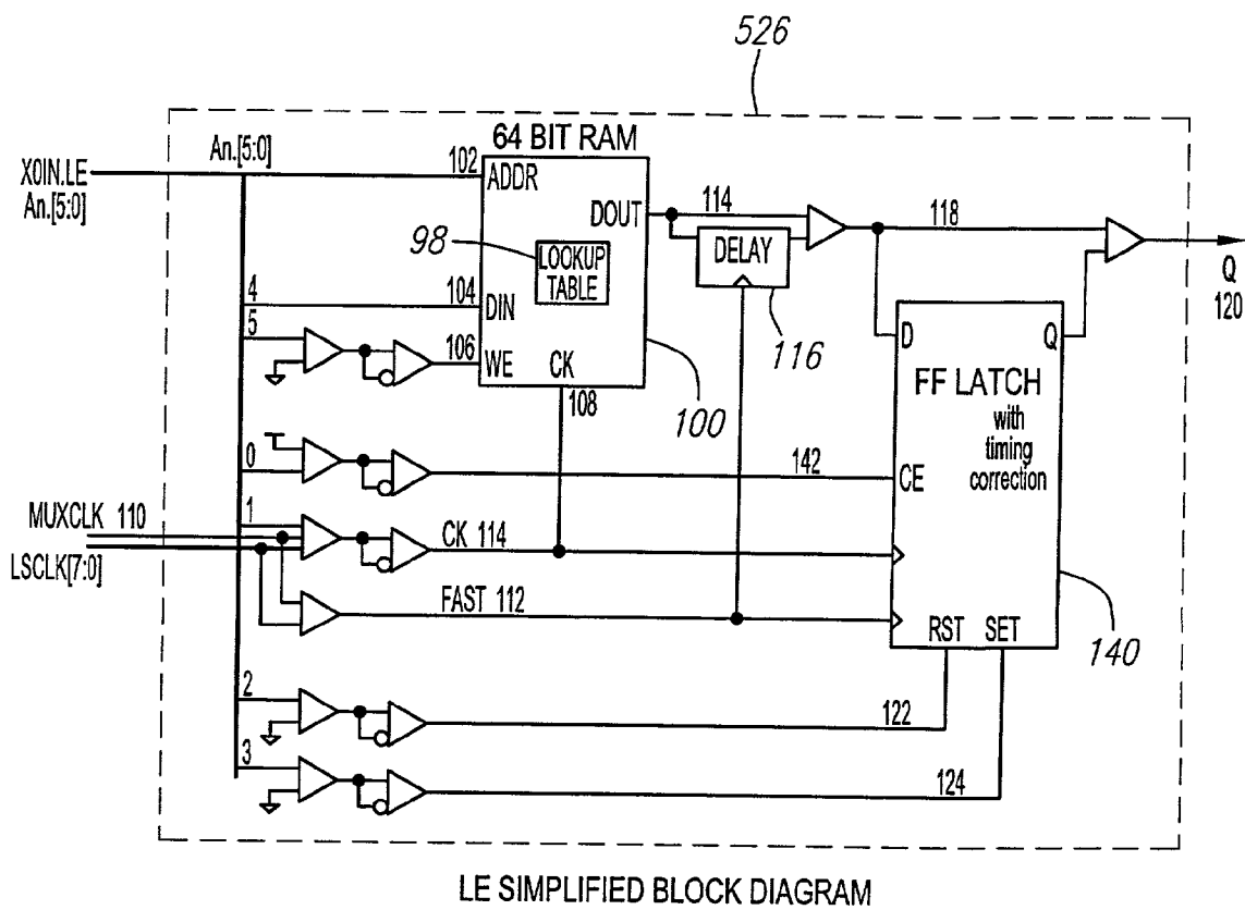
LE SIMPLIFIED BLOCK DIAGRAM FIG. 10
