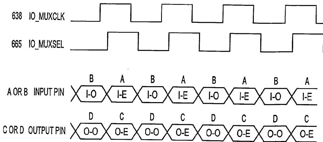
TIMING FOR 2-WAY TIME MULTIPLEXING
