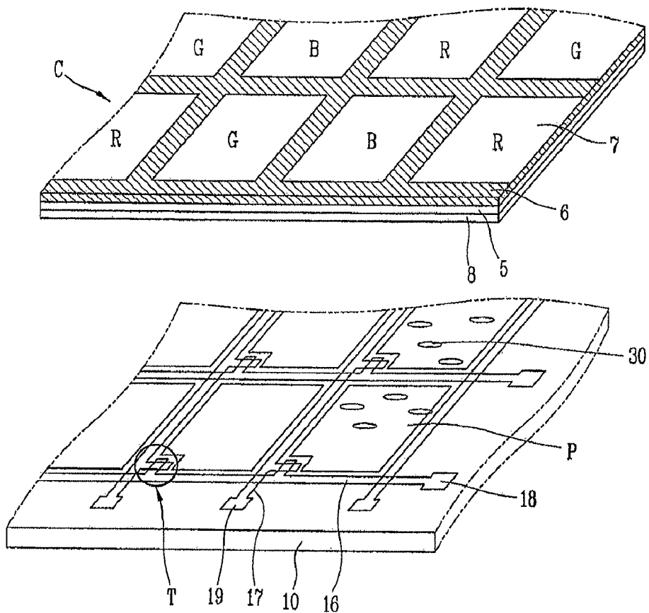
FIG. 2 RELATED ART
