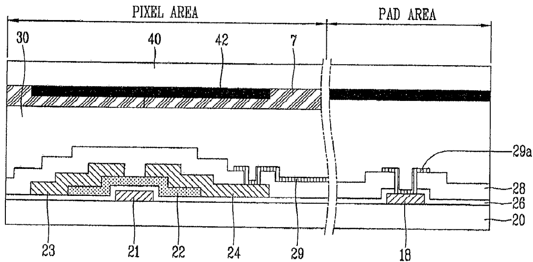
FIG. 2 RELATED ART
