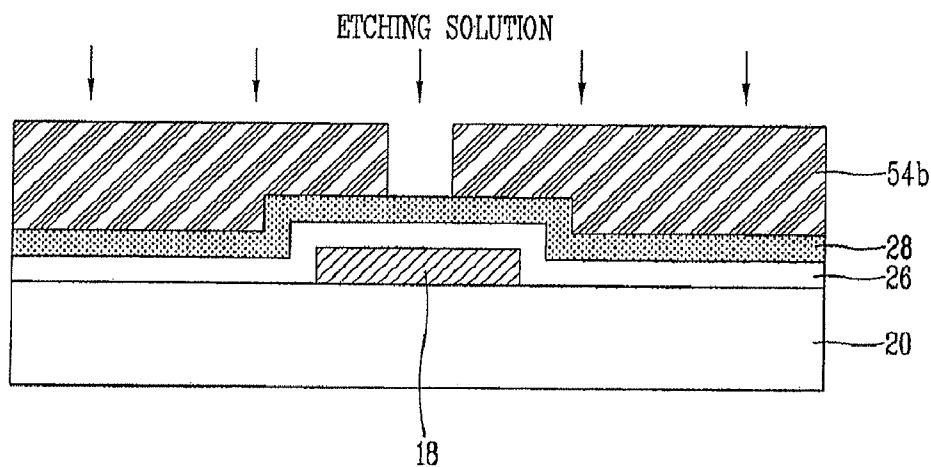
FIG. 3C RELATED ART
