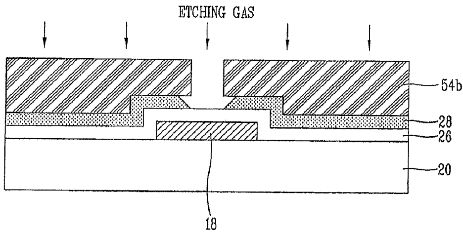
FIG. 3C RELATED ART
