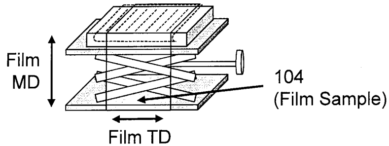
Figure 7c: Testing Fixture After Shrink Tunnel
