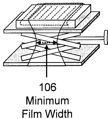
Figure 7c: Testing Fixture After Shrink Tunnel
