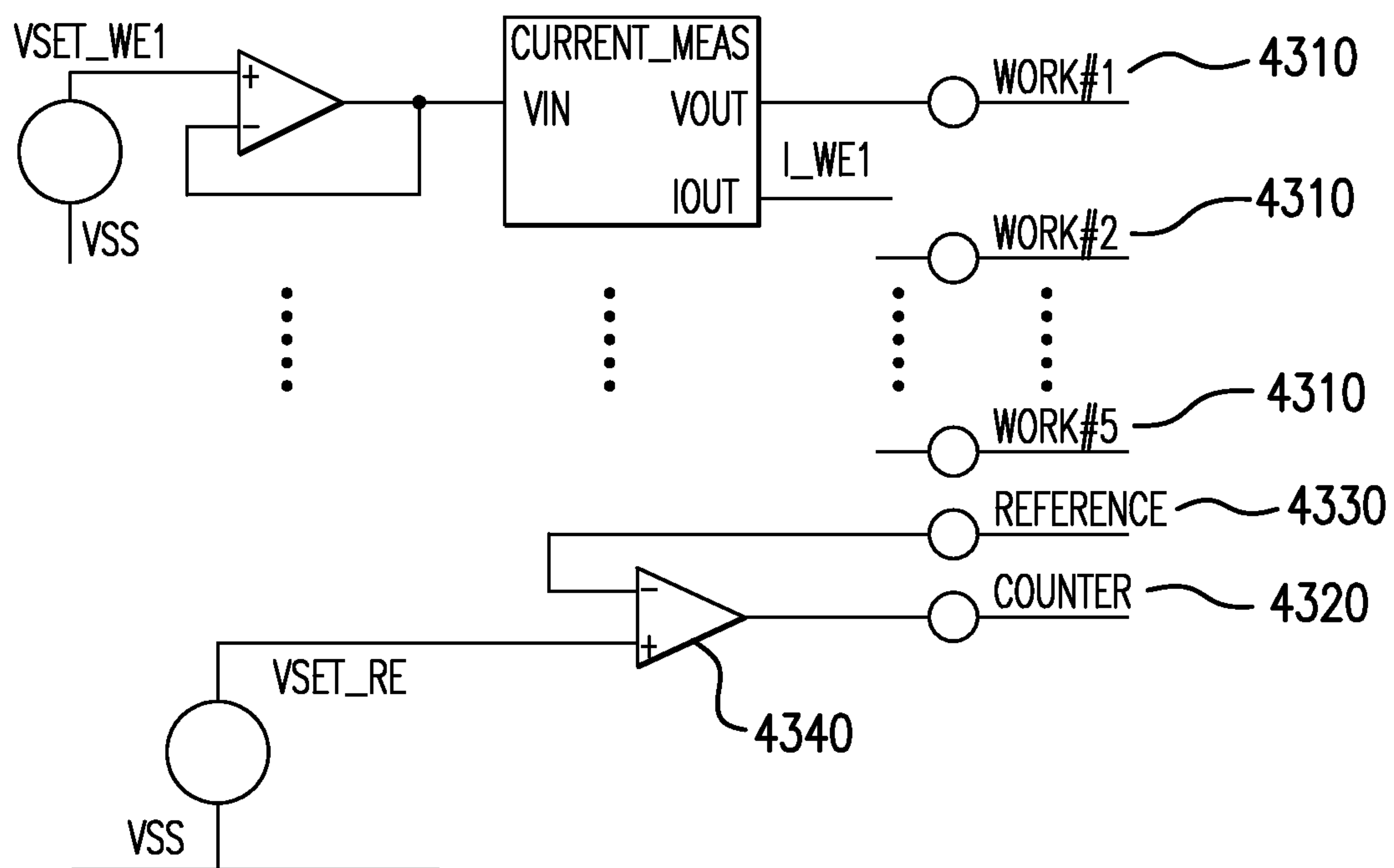
POTENTIOSTAT CONFIGURATION
